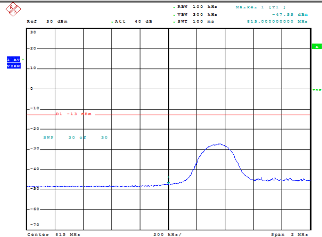
Band18-5MHz-QPSK-23875-1RB#24
