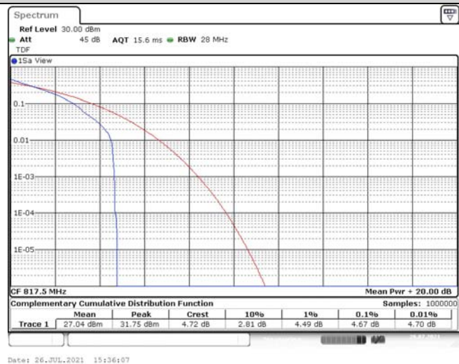
Band18-5MHz-QPSK-23875-25RB#0
