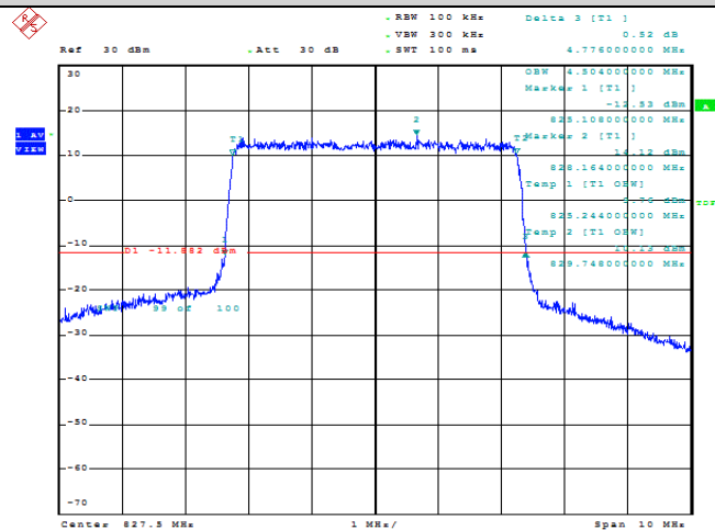
Band18-5MHz-QPSK-23975-25RB#0-4.504
