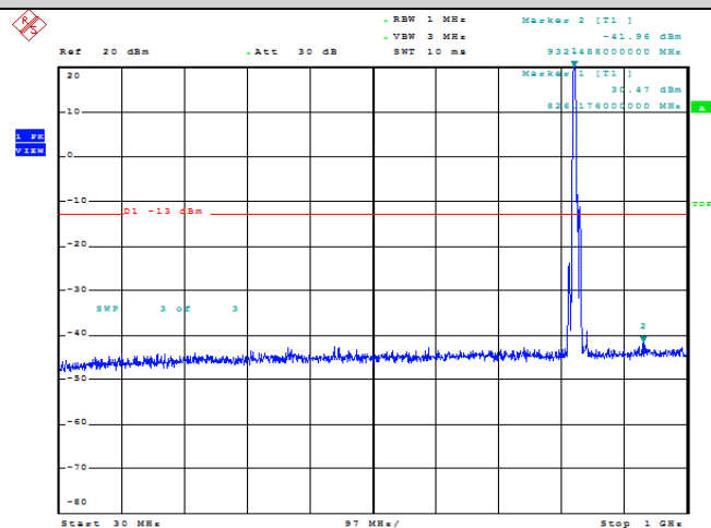
Band18-5MHz-QPSK-23975-1RB#0-Range1:30~1000MHz
