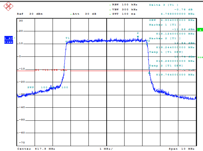
Band18-5MHz-QPSK-23875-25RB#0-4.504
