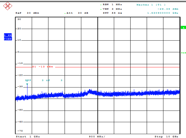
Band18-5MHz-QPSK-23875-1RB#0-Range2:1000~10000MHz
