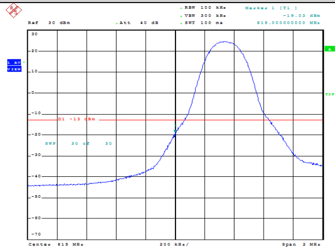
Band18-5MHz-QPSK-23875-1RB#0
