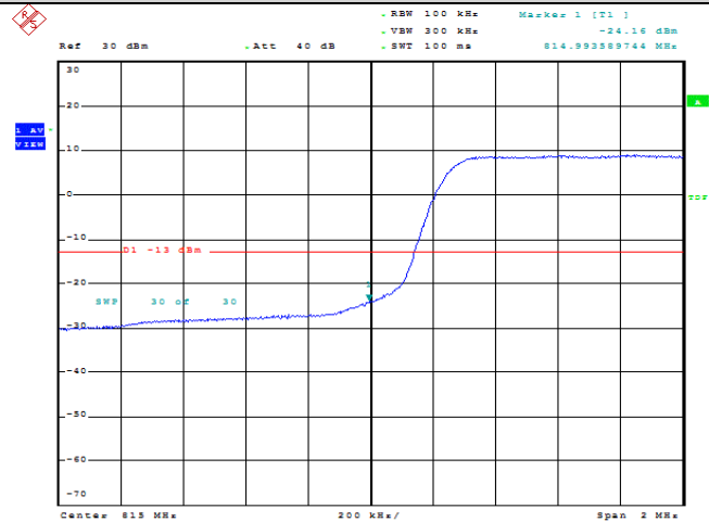
Band18-5MHz-QPSK-23875-25RB#0
