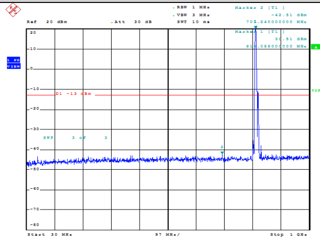
Band18-5MHz-QPSK-23875-1RB#0-Range1:30~1000MHz
