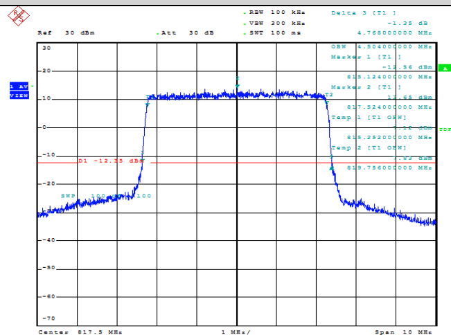
Band18-5MHz-16QAM-23875-25RB#0-4.504
