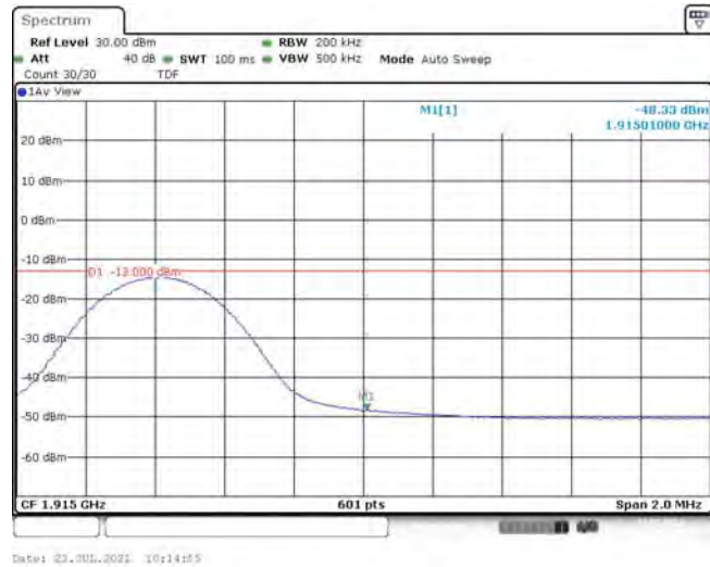
Band25-10MHz-16QAM-26640-1RB#49
