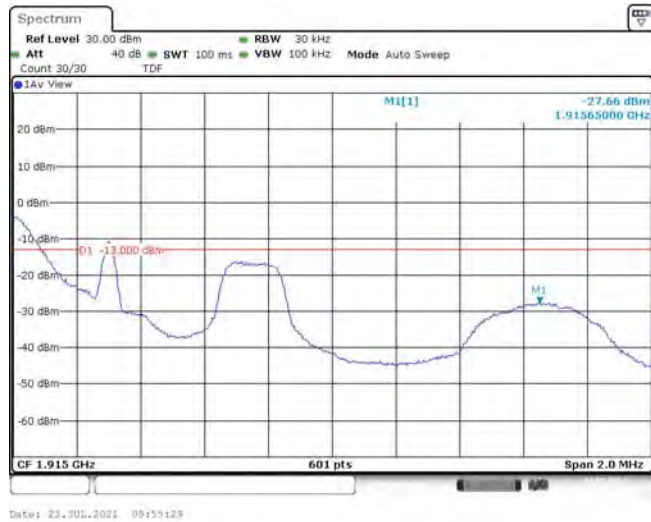
Band25-1.4MHz-QPSK-26683-1RB#5
