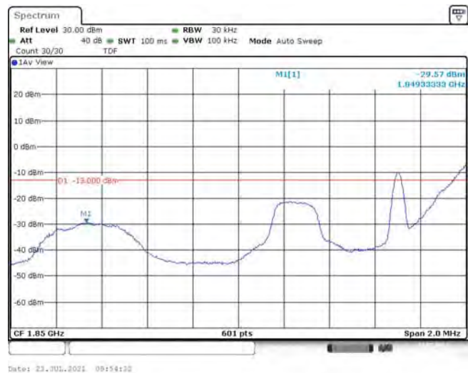
Band25-1.4MHz-QPSK-26047-6RB#0
