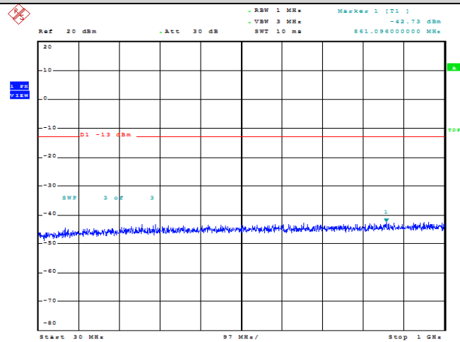
Band25-1.4MHz-QPSK-26047-1RB#0-Range1:30~1000MHz
