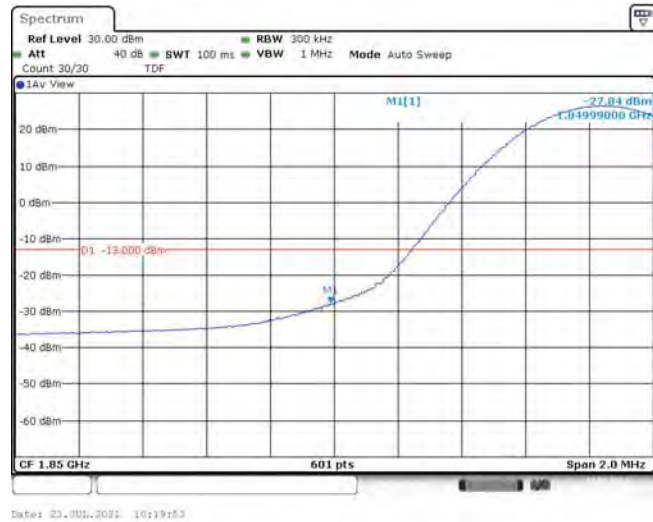
Band25-15MHz-QPSK-26115-1RB#74
