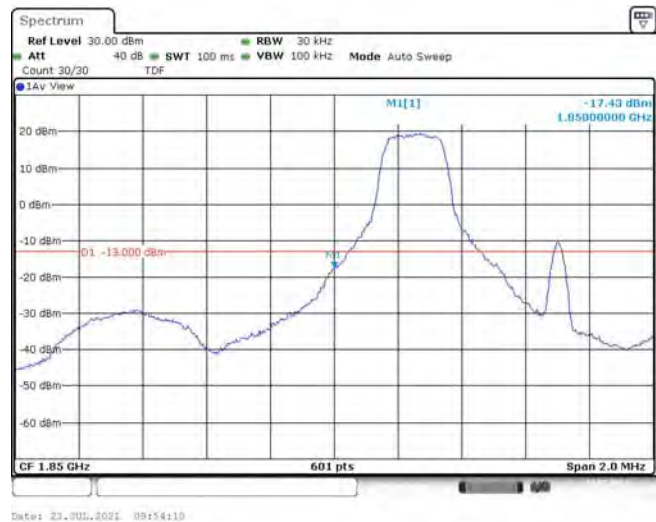
Band25-1.4MHz-QPSK-26047-1RB#5
