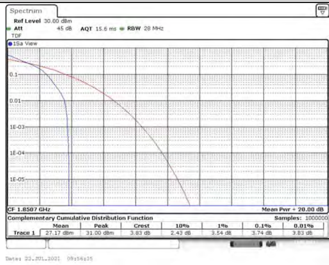
Band25-1.4MHz-QPSK-26047-6RB#0
