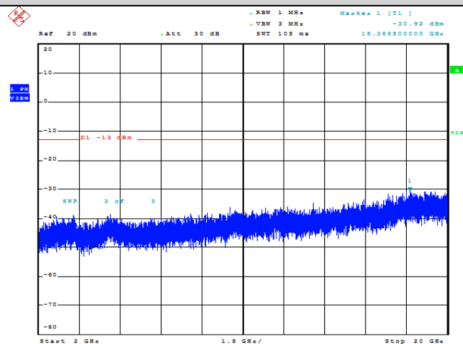
Band25-1.4MHz-QPSK-26047-1RB#0-Range3:2000~20000MHz
