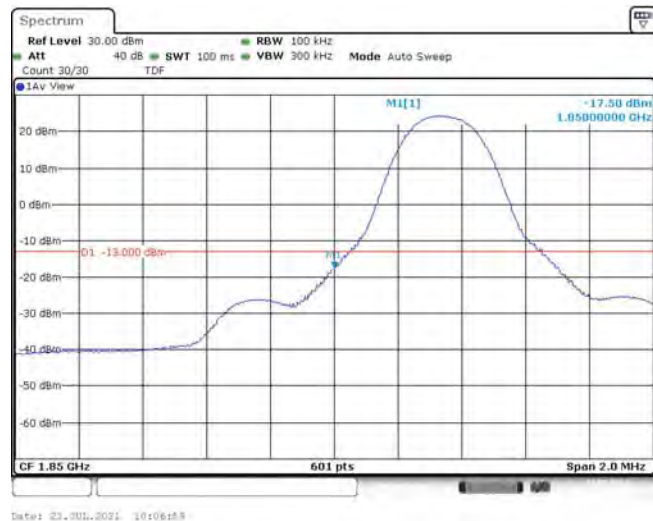
Band25-5MHz-QPSK-26065-1RB#24
