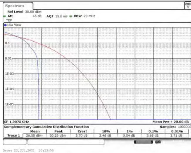
Band25-15MHz-QPSK-26615-75RB#0
