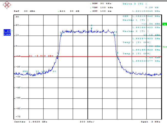
Band25-1.4MHz-QPSK-26365-6RB#0-1.096
