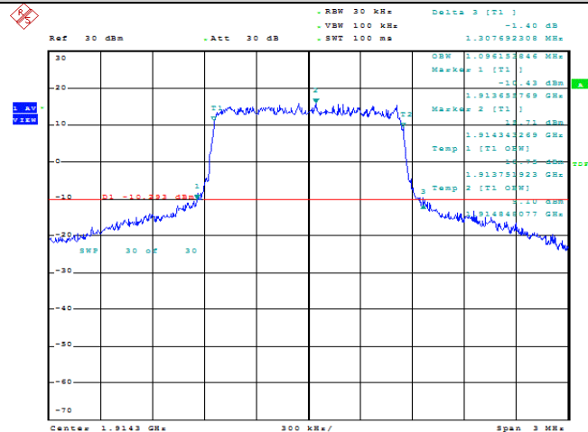
Band25-1.4MHz-QPSK-26683-6RB#0-1.096
