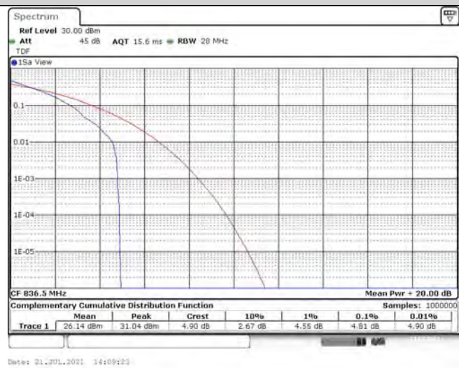
Band5-1.4MHz-QPSK-20525-1RB#0
