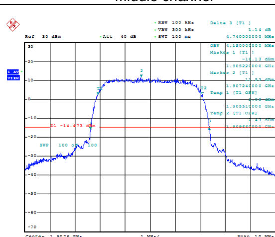
Middle channel
