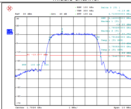
Middle channel
