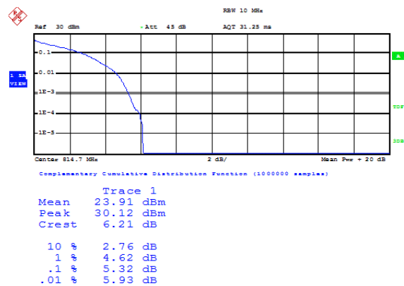
Band26-1.4MHz-QPSK-26697-6RB#0
