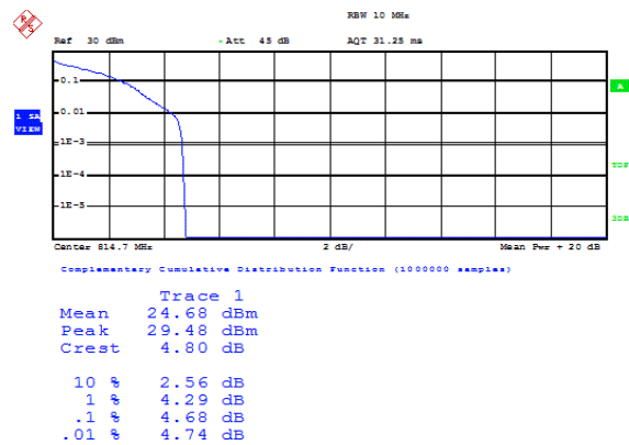
Band26-1.4MHz-QPSK-26697-1RB#0
