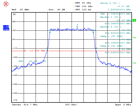
Band26-1.4MHz-QPSK-26697-6RB#0-1.095
