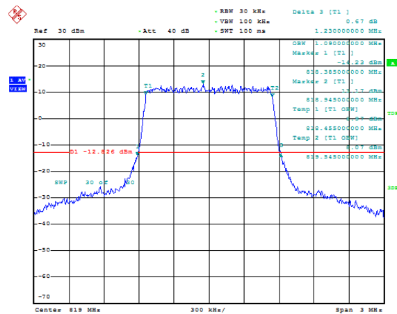
Band26-1.4MHz-QPSK-26740-6RB#0-1.09
