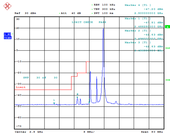
Band7-5MHz-QPSK-20775-1RB#24
