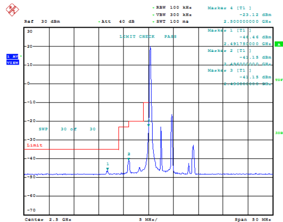
Band7-5MHz-QPSK-20775-1RB#0
