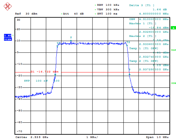
Band7-5MHz-QPSK-21100-25RB#0-4.51
