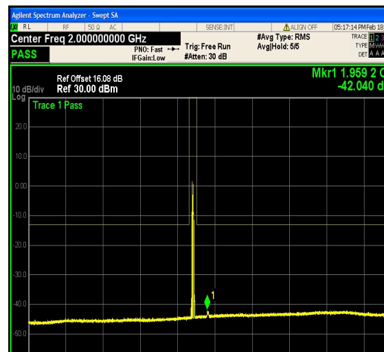
1-N25-PC3-15-10-M-27-CP-256QAM-Outer_ Full-52@0-0.15-30-Ant1--64.44--33-PASS
