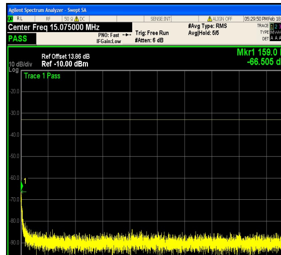
1-N25-PC3-15-10-H-9-DFT-16QAM-Outer_F ull-50@0-0.15-30-Ant1--66.51--33-PASS
