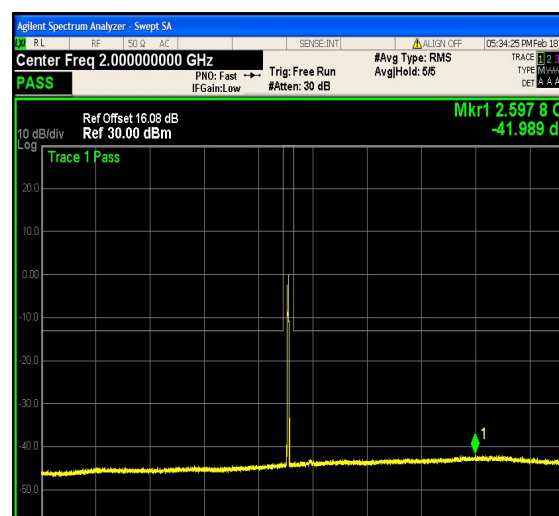
1-N25-PC3-15-10-H-12-DFT-64QAM-Outer_ Full-50@0-0.15-30-Ant1--64.36--33-PASS
