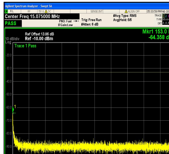
1-N25-PC3-15-10-H-12-DFT-64QAM-Outer_ Full-50@0-0.15-30-Ant1--64.36--33-PASS
