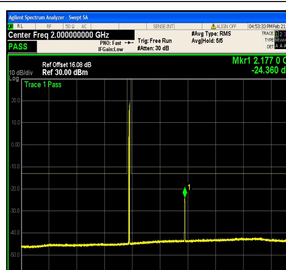
1-N66-PC3-15-5-H-17-CP-QPSK-Edge_1RB _Right-1@24-1000-3000-Ant1--24.36--13-PASS
