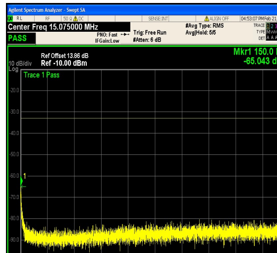
1-N66-PC3-15-5-H-17-CP-QPSK-Edge_1RB _Right-1@24-0.15-30-Ant1--65.04--33-PASS
