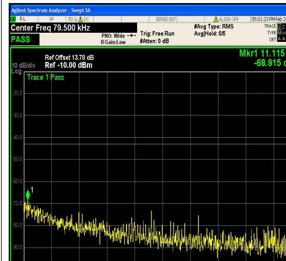
1-N66-PC3-15-5-H-23-CP-64QAM-Edge_1R B_Right-1@24-0.009-0.15-Ant1--68.92--43-P ASS
