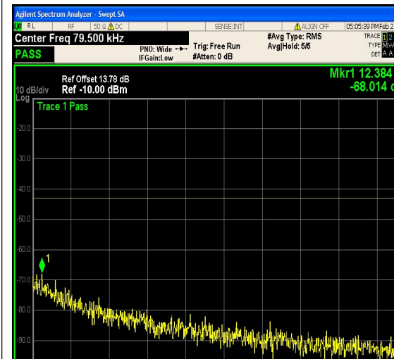
1-N66-PC3-15-5-H-26-CP-256QAM-Edge_1 RB_Right-1@24-0.009-0.15-Ant1--68.01--43- PASS
