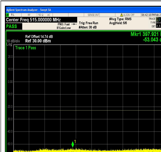
1-N66-PC3-15-10-M-25-CP-256QAM-Edge_ 1RB_Left-1@0-30-1000-Ant1--53.04--23-PA SS
