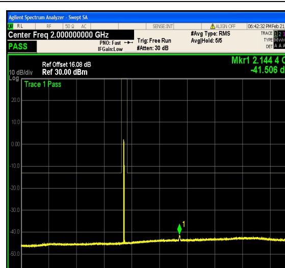
1-N66-PC3-15-10-M-25-CP-256QAM-Edge_ 1RB_Left-1@0-1000-3000-Ant1--41.51--13-P ASS
