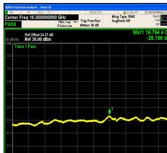
1-N66-PC3-15-15-L-15-DFT-256QAM-Outer_
