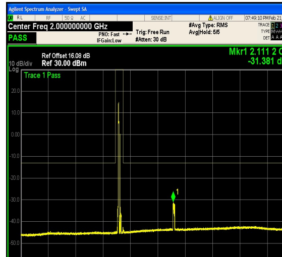
1-N66-PC3-15-15-L-15-DFT-256QAM-Outer_ Full-75@0-1000-3000-Ant1--31.38--13-PASS
