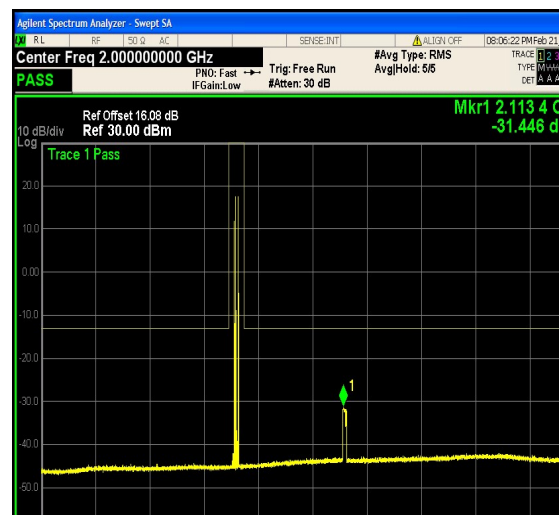
1-N66-PC3-15-15-L-27-CP-256QAM-Outer_ Full-79@0-1000-3000-Ant1--31.45--13-PASS
