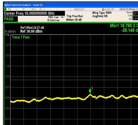
1-N66-PC3-15-15-L-26-CP-256QAM-Edge_1 RB_Right-1@78-12000-20000-Ant1--26.15-- 13-PASS
