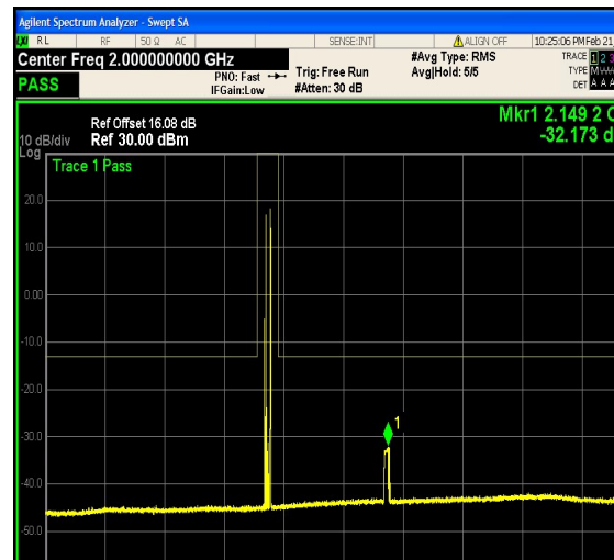
1-N66-PC3-15-20-M-11-DFT-64QAM-Edge_1 RB_Right-1@105-1000-3000-Ant1--32.17--1 3-PASS
