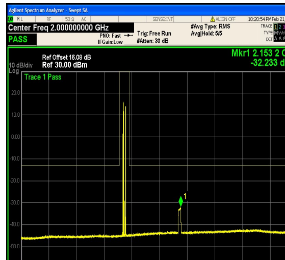
1-N66-PC3-15-20-M-8-DFT-16QAM-Edge_1 RB_Right-1@105-1000-3000-Ant1--32.23--1 3-PASS
