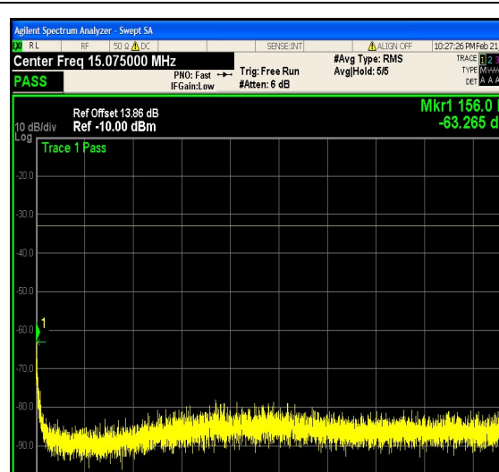
1-N66-PC3-15-20-M-13-DFT-256QAM-Edge _1RB_Left-1@0-0.15-30-Ant1--63.27--33-PA SS
