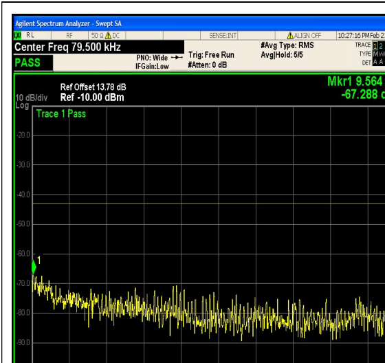
1-N66-PC3-15-20-M-13-DFT-256QAM-Edge _1RB_Left-1@0-0.009-0.15-Ant1--67.29--43- PASS
