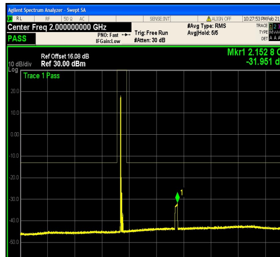
1-N66-PC3-15-20-M-13-DFT-256QAM-Edge _1RB_Left-1@0-1000-3000-Ant1--31.95--13- PASS
