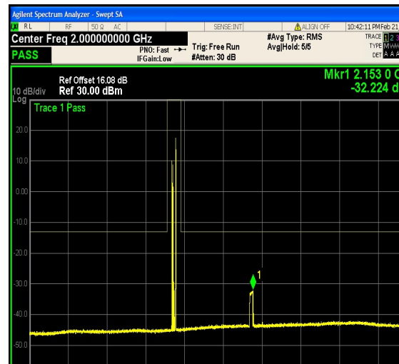
1-N66-PC3-15-20-M-23-CP-64QAM-Edge_1 RB_Right-1@105-1000-3000-Ant1--32.22--1 3-PASS
