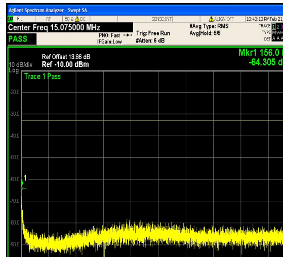
1-N66-PC3-15-20-M-24-CP-64QAM-Outer_F ull-106@0-0.15-30-Ant1--64.31--33-PASS
