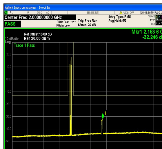
1-N66-PC3-15-20-M-24-CP-64QAM-Outer_F ull-106@0-0.15-30-Ant1--64.31--33-PASS
