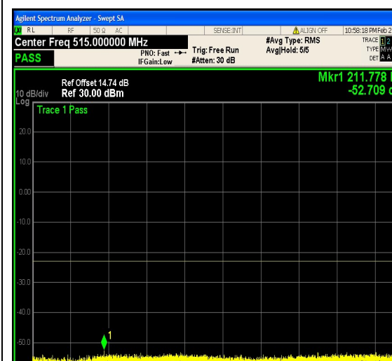
1-N66-PC3-15-20-H-6-DFT-QPSK-Outer_Full -100@0-0.009-0.15-Ant1--68.76--43-PASS
