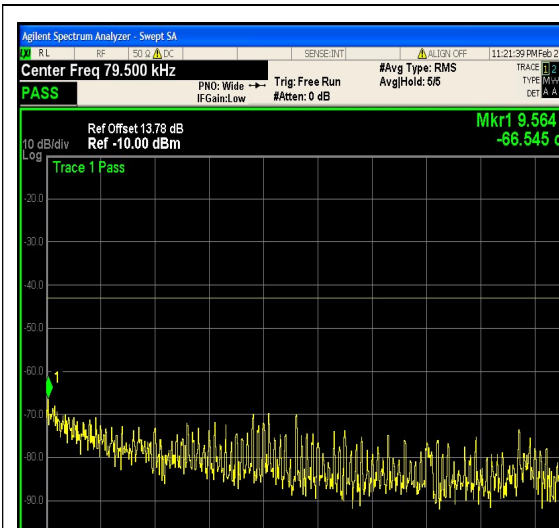
1-N66-PC3-15-20-H-23-CP-64QAM-Edge_1 RB_Right-1@105-0.009-0.15-Ant1--66.54--4 3-PASS
