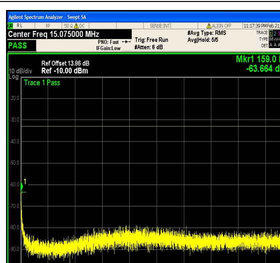
1-N66-PC3-15-20-H-20-CP-16QAM-Edge_1 RB_Right-1@105-0.15-30-Ant1--63.66--33-P ASS
