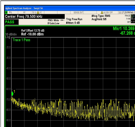
1-N66-PC3-15-20-H-20-CP-16QAM-Edge_1 RB_Right-1@105-0.009-0.15-Ant1--67.27--4 3-PASS
