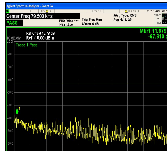
1-N66-PC3-15-20-H-24-CP-64QAM-Outer_F ull-106@0-0.009-0.15-Ant1--67.61--43-PASS
