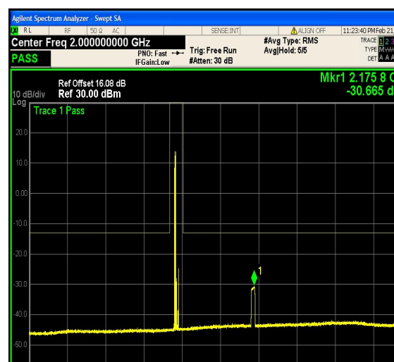
1-N66-PC3-15-20-H-24-CP-64QAM-Outer_F ull-106@0-0.15-30-Ant1--65.17--33-PASS
