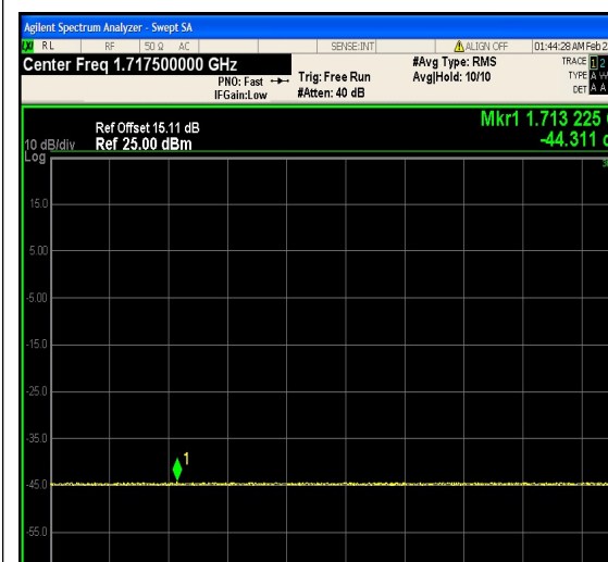
1-N66-PC3-15-15-L-4-CP-QPSK-Edge_1RB _Left-1@0-Ant1-1710.0~1725.0(1713.225MH z,-44.31MHz,Limit30,Margin[74.31])-PASS-se e graph
