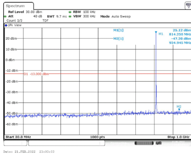
Band26-3MHz-16QAM-26705-1RB#0-Range1:30~1000MHz
