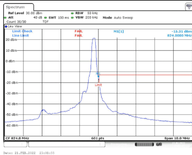
Band26-3MHz-QPSK-26775-1RB#14
