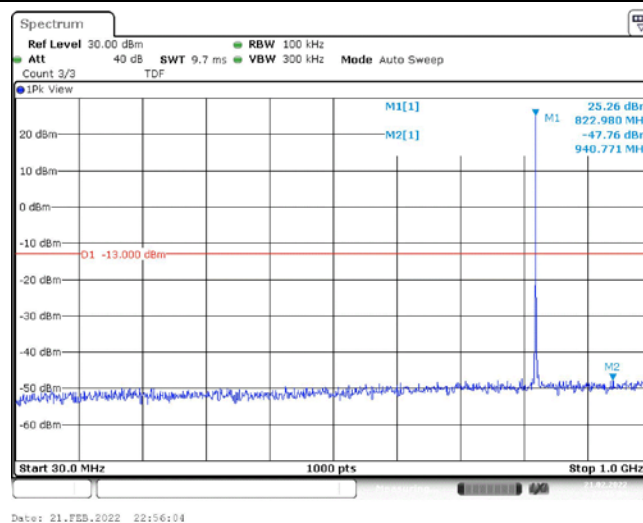
Band26-1.4MHz-16QAM-26783-1RB#0-Range1:30~1000MHz
