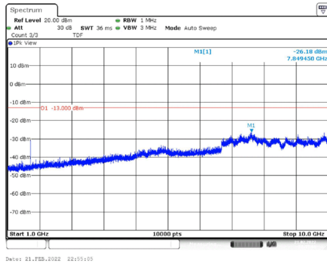
Band26-1.4MHz-QPSK-26740-1RB#0-Range2:1000~10000MHz
