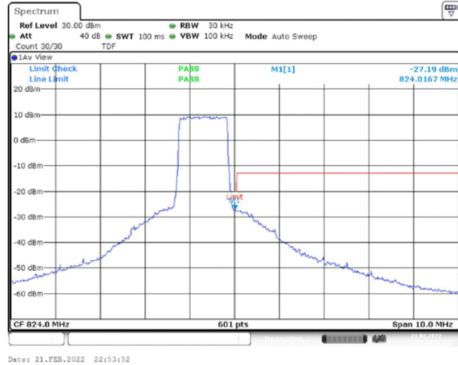
Band26-1.4MHz-16QAM-26783-6RB#0
