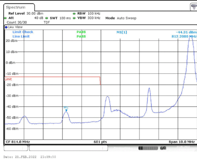
Band26-5MHz-QPSK-26715-1RB#24
