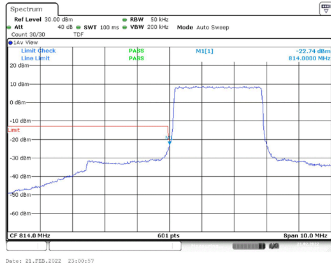
Band26-3MHz-QPSK-26705-15RB#0
