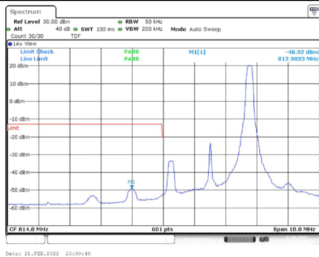
Band26-3MHz-16QAM-26705-1RB#14
