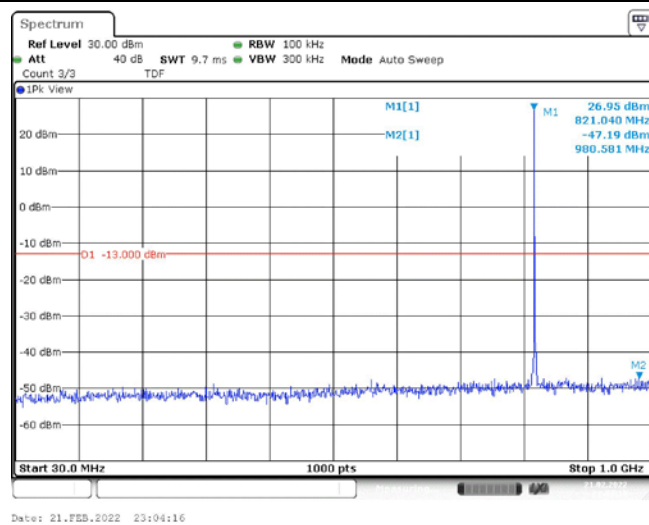
Band26-3MHz-QPSK-26775-1RB#0-Range1:30~1000MHz
