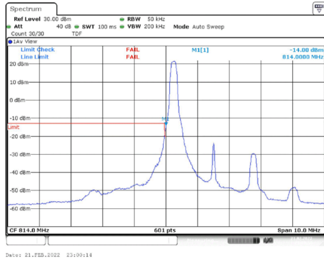
Band26-3MHz-QPSK-26705-1RB#0
