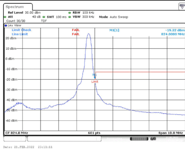
Band26-5MHz-QPSK-26765-1RB#24
