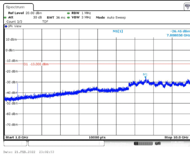
Band26-3MHz-QPSK-26705-1RB#0-Range2:1000~10000MHz
