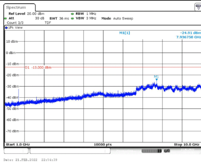
Band26-1.4MHz-16QAM-26697-1RB#0-Range2:1000~10000MHz
