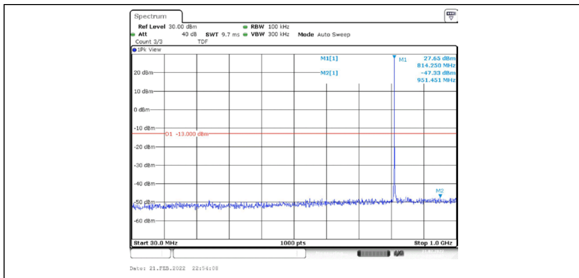
Band26-1.4MHz-QPSK-26697-1RB#0-Range1:30~1000MHz
