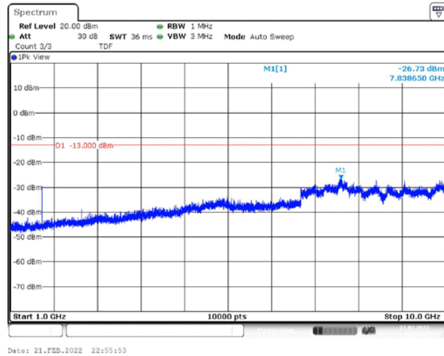
Band26-1.4MHz-QPSK-26783-1RB#0-Range2:1000~10000MHz
