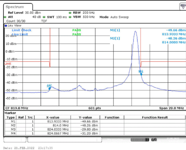
Band26-10MHz-QPSK-26740-1RB#49
