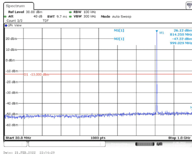
Band26-1.4MHz-16QAM-26697-1RB#0-Range1:30~1000MHz
