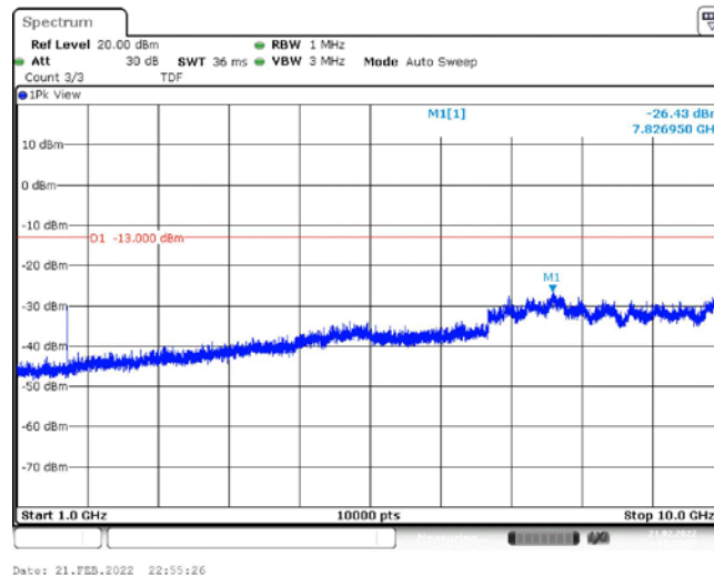
Band26-1.4MHz-16QAM-26740-1RB#0-Range2:1000~10000MHz
