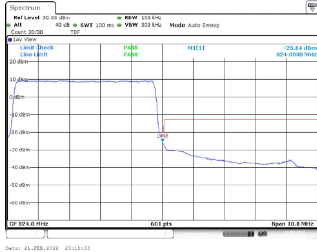
Band26-5MHz-QPSK-26765-25RB#0
