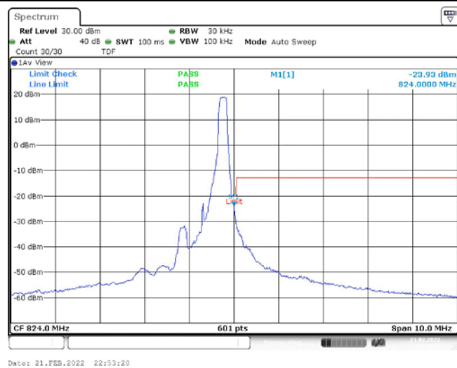
Band26-1.4MHz-QPSK-26783-1RB#5
