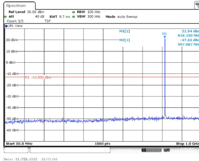
Band26-1.4MHz-16QAM-26740-1RB#0-Range1:30~1000MHz
