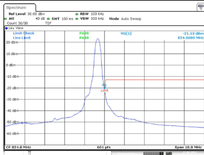
Band26-5MHz-16QAM-26765-1RB#0
