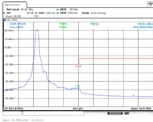
Band26-3MHz-QPSK-26775-1RB#0
