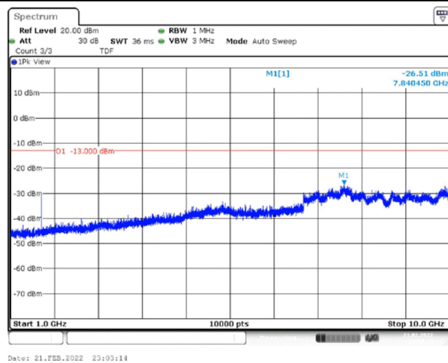
Band26-3MHz-16QAM-26705-1RB#0-Range2:1000~10000MHz
