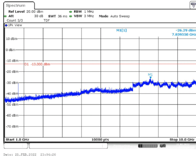
Band26-3MHz-QPSK-26775-1RB#0-Range2:1000~10000MHz
