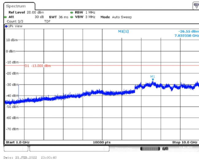
Band26-3MHz-QPSK-26740-1RB#0-Range2:1000~10000MHz
