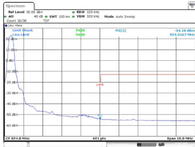
Band26-5MHz-16QAM-26715-25RB#0
