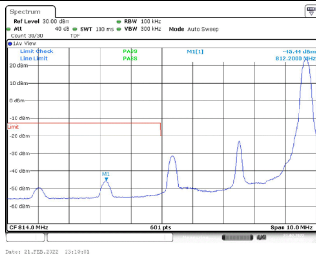
Band26-5MHz-16QAM-26715-1RB#24
