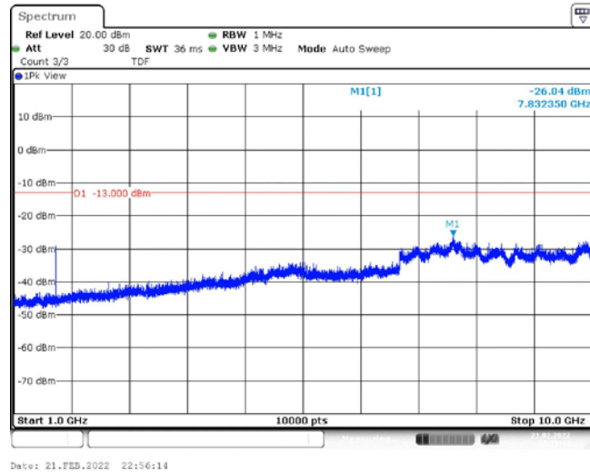
Band26-1.4MHz-16QAM-26783-1RB#0-Range2:1000~10000MHz
