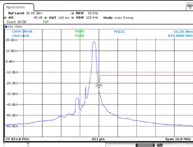
Band26-1.4MHz-16QAM-26783-1RB#0
