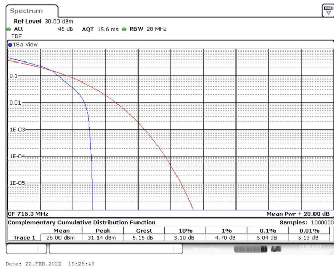
Band12-1.4MHz-16QAM-23173-1RB#0
