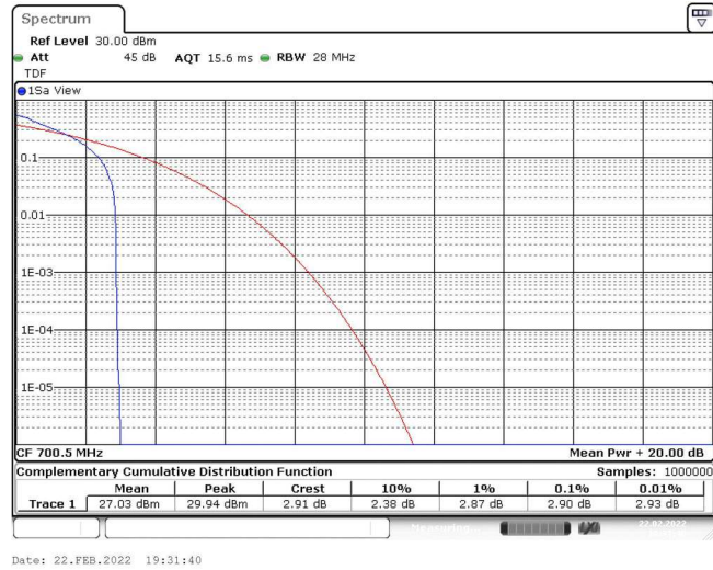
Band12-3MHz-QPSK-23025-1RB#0
