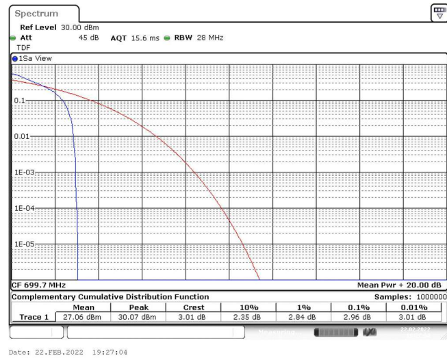
Band12-1.4MHz-QPSK-23017-1RB#0
