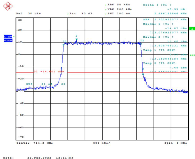
Band12-3MHz-16QAM-23165-15RB#0-2.702
