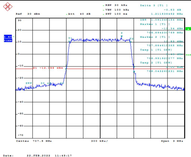
Band12-1.4MHz-16QAM-23095-6RB#0-1.091
