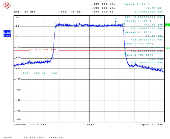
Band12-5MHz-16QAM-23155-25RB#0-4.52
