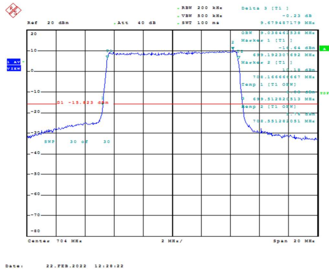
Band12-10MHz-16QAM-23060-50RB#0-9.038
