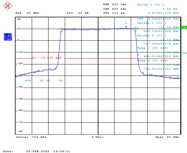
Band12-10MHz-QPSK-23060-50RB#0-9.038
