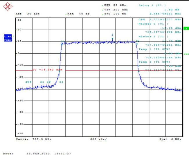
Band12-3MHz-16QAM-23095-15RB#0-2.702
