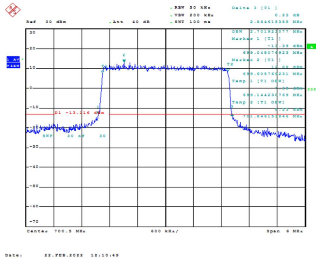
Band12-3MHz-QPSK-23025-15RB#0-2.702
