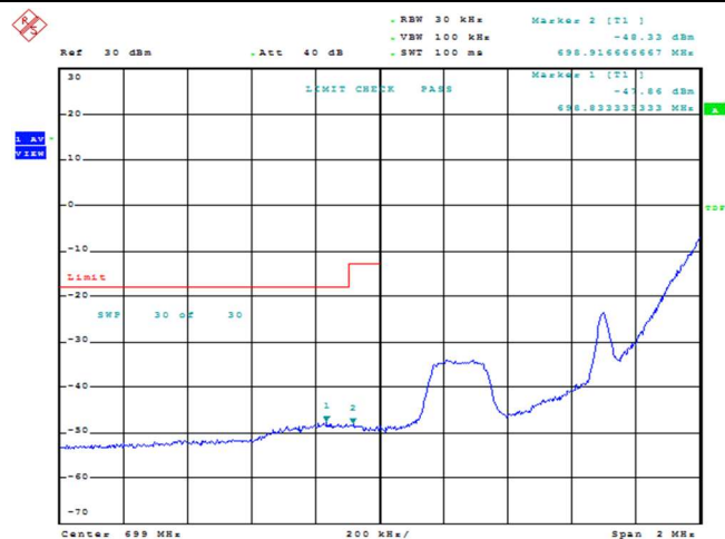
Band12-1.4MHz-16QAM-23017-1RB#0
