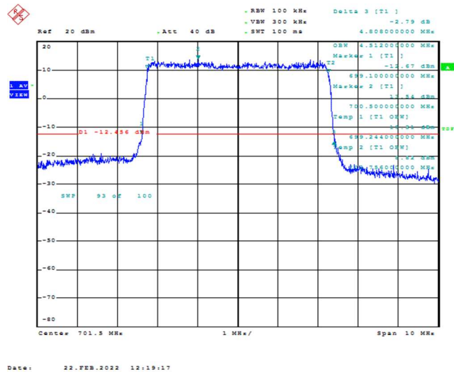
Band12-5MHz-QPSK-23035-25RB#0-4.512
