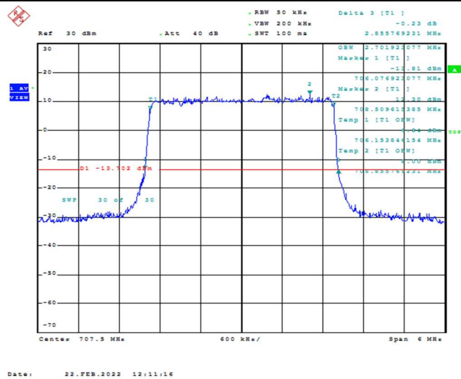
Band12-3MHz-QPSK-23095-15RB#0-2.702
