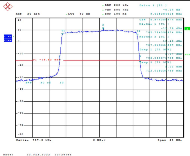
Band12-10MHz-16QAM-23095-50RB#0-8.974
