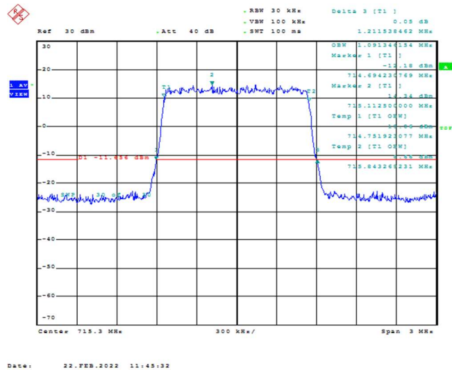
Band12-1.4MHz-QPSK-23173-6RB#0-1.091
