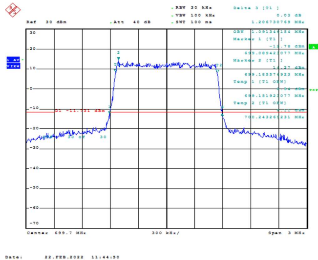
Band12-1.4MHz-16QAM-23017-6RB#0-1.091
