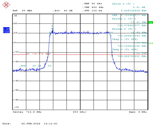
Band12-3MHz-QPSK-23165-15RB#0-2.702
