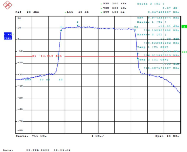
Band12-10MHz-QPSK-23130-50RB#0-8.974
