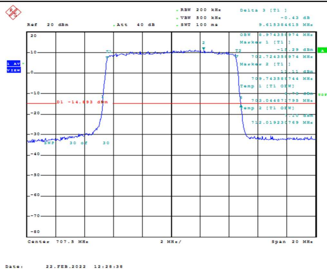
Band12-10MHz-QPSK-23095-50RB#0-8.974
