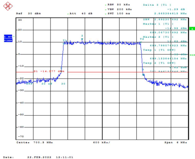
Band12-3MHz-16QAM-23025-15RB#0-2.692
