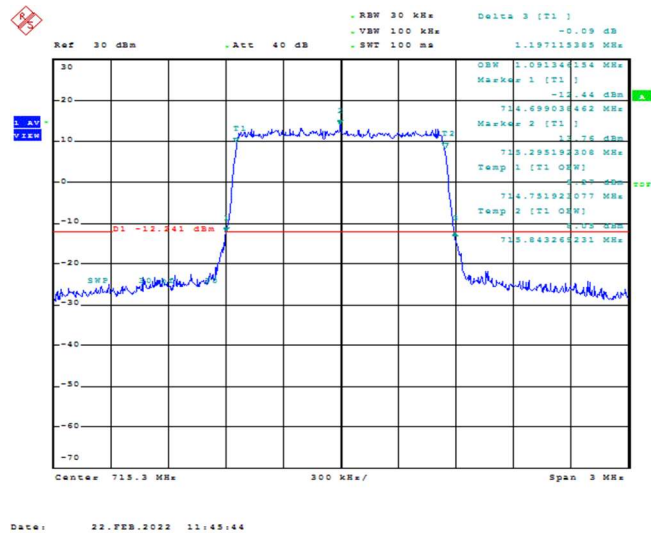
Band12-1.4MHz-16QAM-23173-6RB#0-1.091
