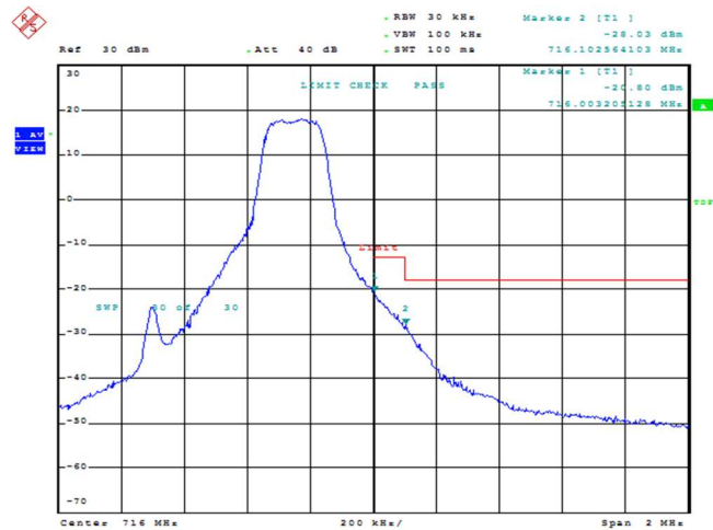
Band12-1.4MHz-16QAM-23173-1RB#0
