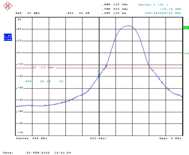
Band12-5MHz-16QAM-23035-1RB#0
