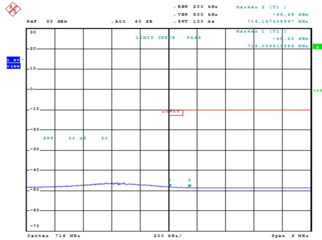
Band12-10MHz-QPSK-23060-50RB#0
