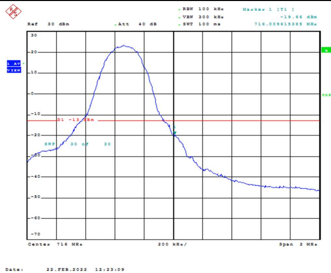
Band12-5MHz-16QAM-23155-1RB#24
