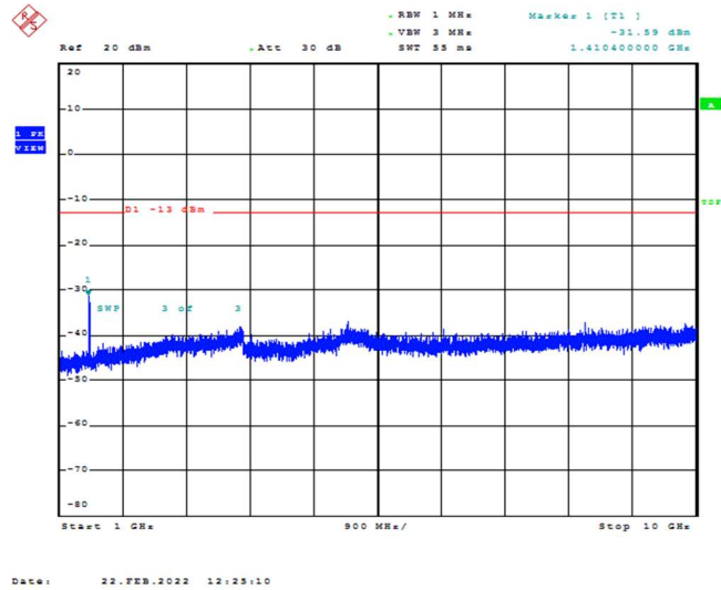
Band12-5MHz-16QAM-23095-1RB#0-Range2:1000~10000MHz
