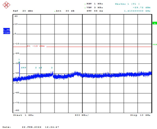
Band12-5MHz-QPSK-23095-1RB#0-Range2:1000~10000MHz
