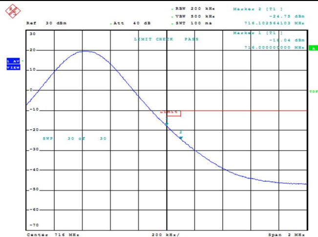
Band12-10MHz-QPSK-23130-1RB#0
