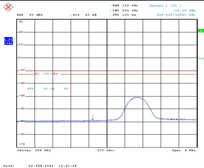
Band12-5MHz-16QAM-23035-1RB#24
