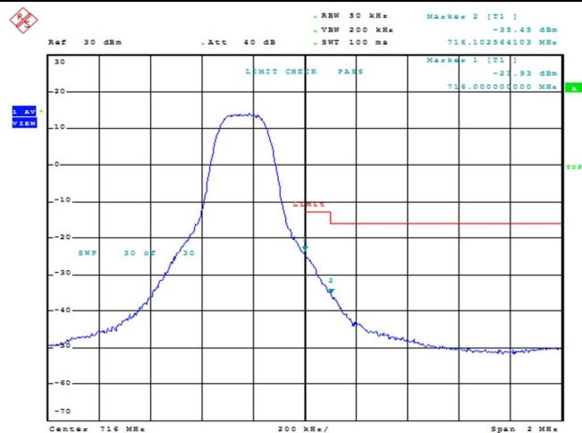
Band12-3MHz-16QAM-23165-1RB#0
