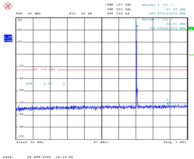
Band12-3MHz-16QAM-23165-1RB#0-Range1:30~1000MHz
