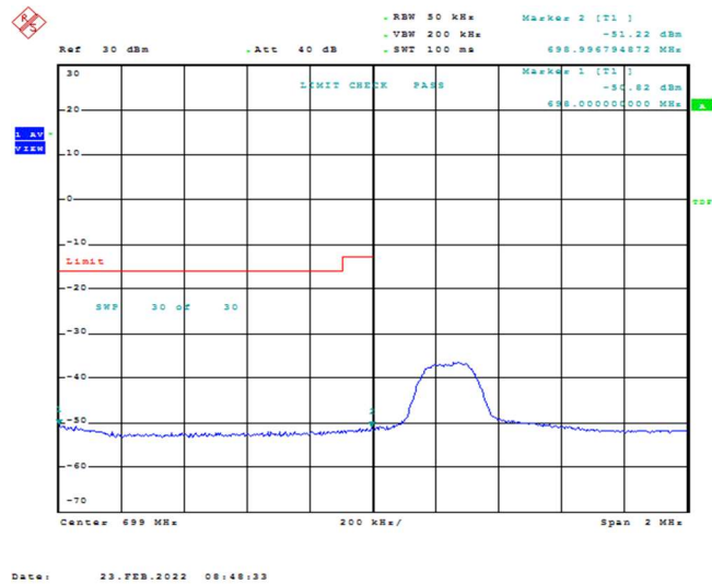
Band12-3MHz-16QAM-23025-1RB#14
