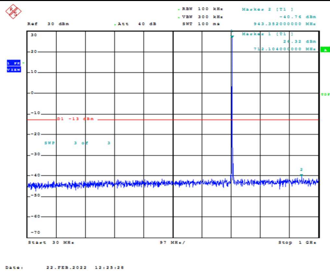
Band12-5MHz-QPSK-23155-1RB#0-Range1:30~1000MHz
