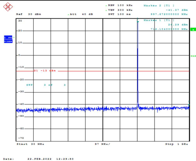
Band12-5MHz-16QAM-23155-1RB#0-Range1:30~1000MHz
