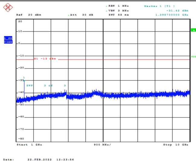
Band12-5MHz-QPSK-23035-1RB#0-Range2:1000~10000MHz
