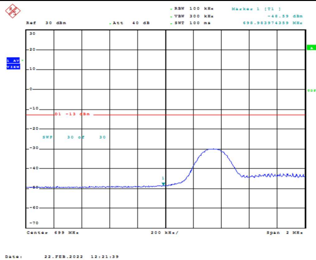
Band12-5MHz-QPSK-23035-1RB#24
