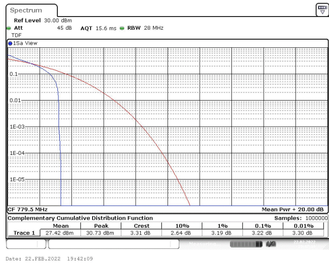
Band13-5MHz-QPSK-23205-1RB#0
