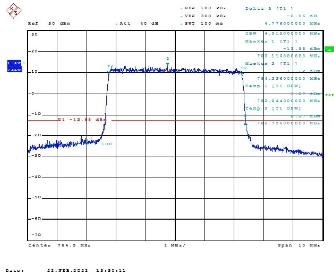
Band13-5MHz-16QAM-23255-25RB#0-4.512
