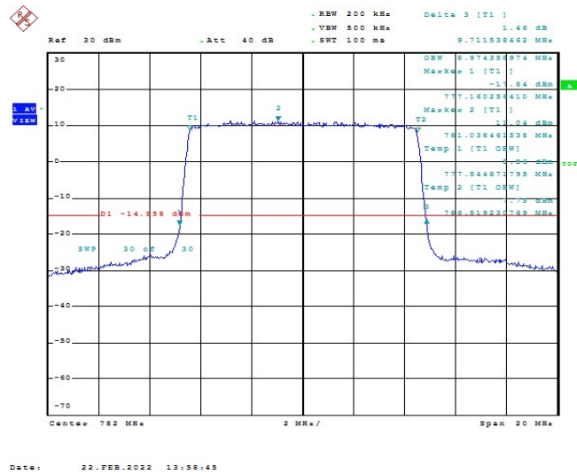
Band13-10MHz-QPSK-23230-50RB#0-8.974
