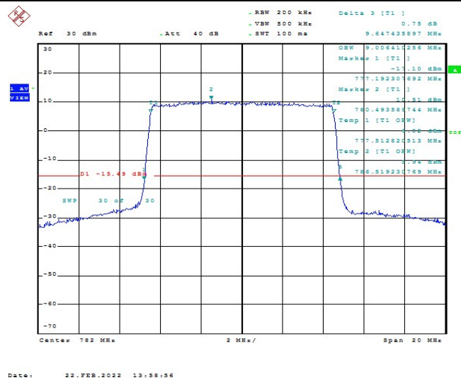
Band13-10MHz-16QAM-23230-50RB#0-9.006
