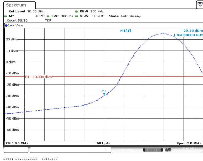
Band2-10MHz-16QAM-18650-1RB#0
