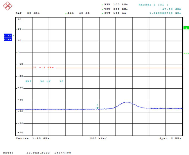
Band2-5MHz-16QAM-18625-1RB#24
