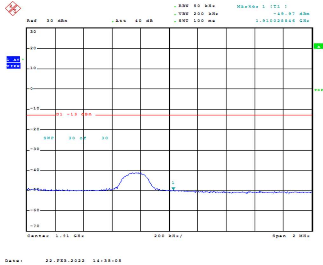
Band2-3MHz-16QAM-19185-1RB#0
