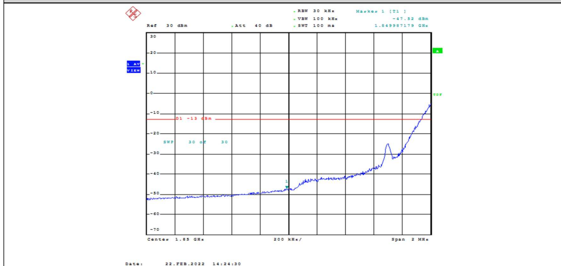
Band2-1.4MHz-QPSK-18607-1RB#5
