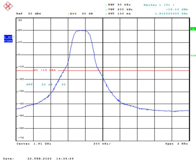
Band2-3MHz-16QAM-19185-1RB#14
