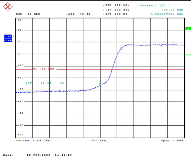
Band2-5MHz-16QAM-18625-25RB#0
