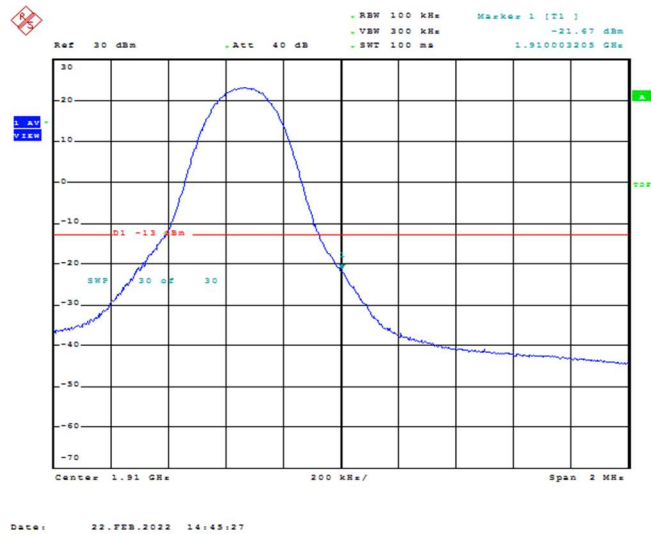
Band2-5MHz-16QAM-19175-1RB#24
