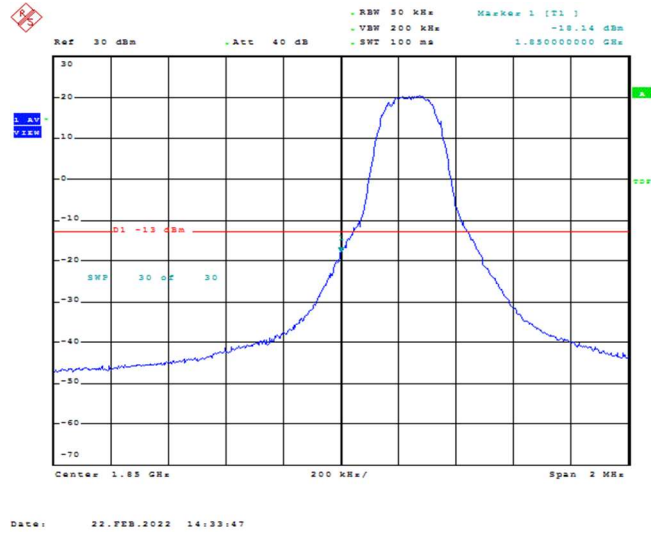
Band2-3MHz-16QAM-18615-1RB#0
