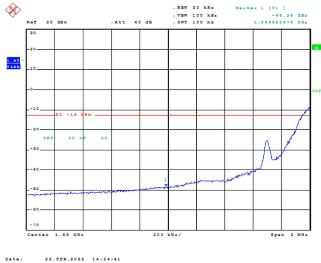
Band2-1.4MHz-16QAM-18607-1RB#5
