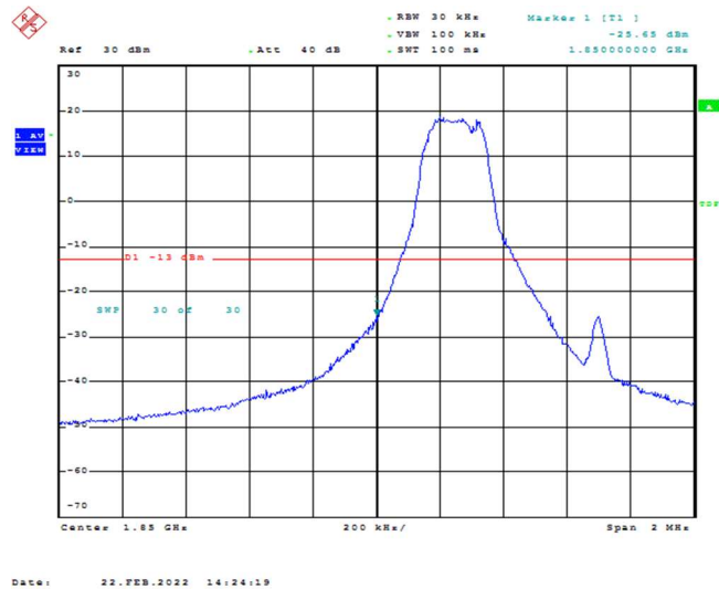
Band2-1.4MHz-16QAM-18607-1RB#0
