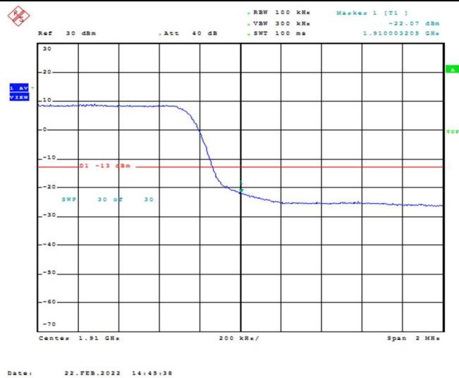
Band2-5MHz-QPSK-19175-25RB#0
