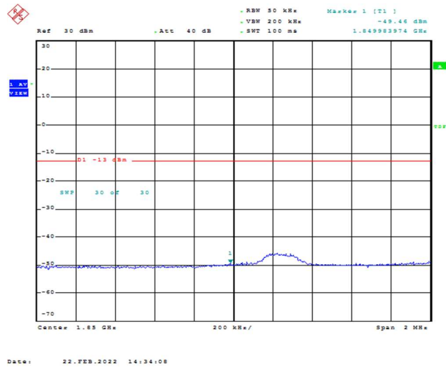
Band2-3MHz-16QAM-18615-1RB#14
