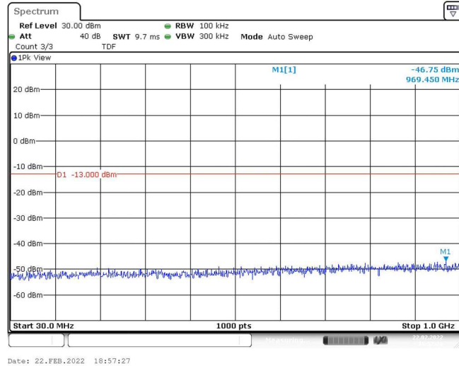
Band2-10MHz-QPSK-19150-1RB#0-Range1:30~1000MHz
