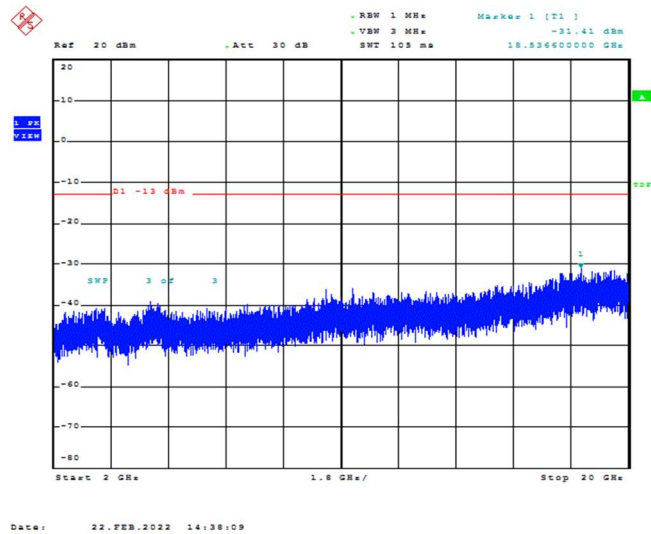
Band2-3MHz-16QAM-18900-1RB#0-Range3:2000~20000MHz
