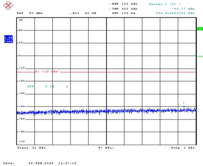
Band2-3MHz-QPSK-18900-1RB#0-Range1:30~1000MHz
