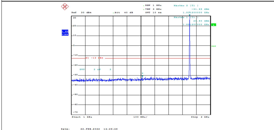
Band2-1.4MHz-QPSK-18607-1RB#0-Range2:1000~2000MHz
