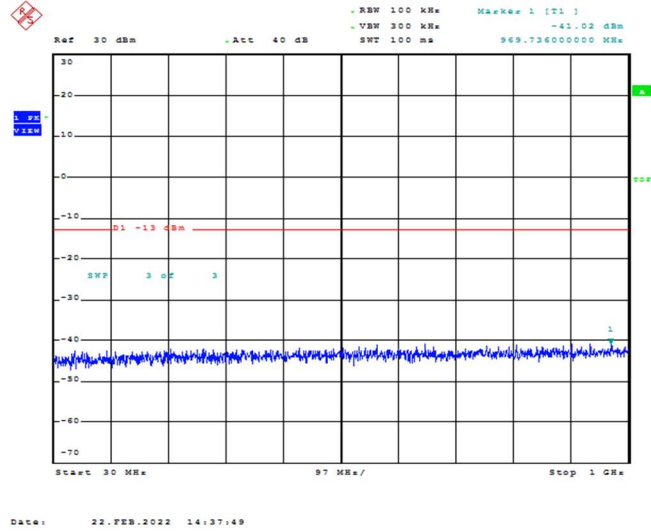
Band2-3MHz-16QAM-18900-1RB#0-Range1:30~1000MHz
