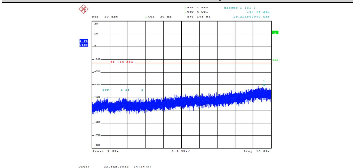
Band2-1.4MHz-QPSK-18607-1RB#0-Range3:2000~20000MHz
