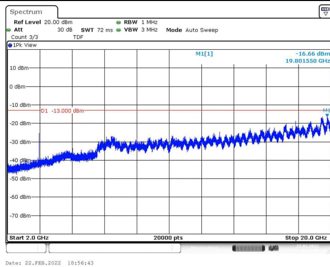
Band2-10MHz-QPSK-18900-1RB#0-Range3:2000~20000MHz
