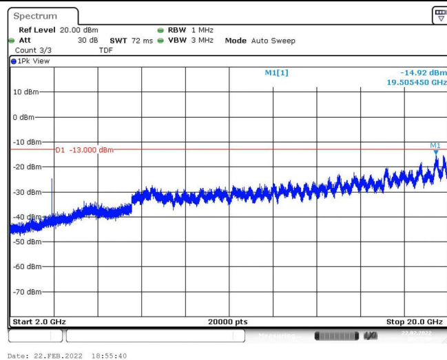
Band2-10MHz-QPSK-18650-1RB#0-Range3:2000~20000MHz
