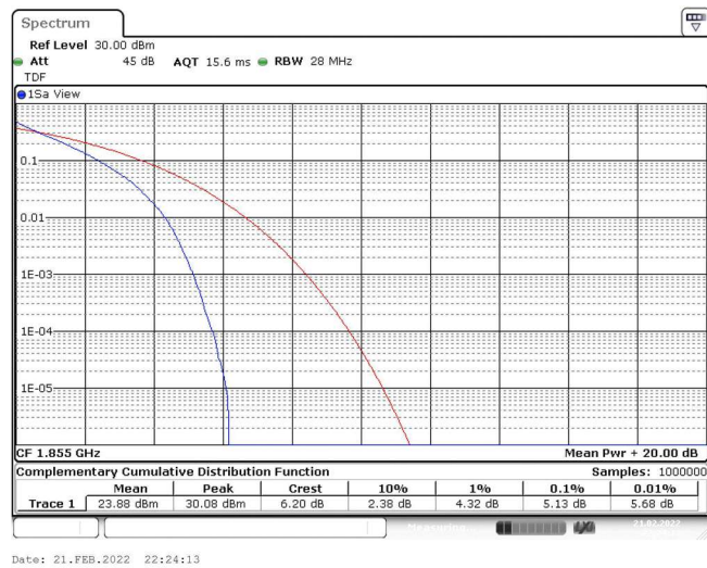
Band25-10MHz-QPSK-26090-50RB#0
