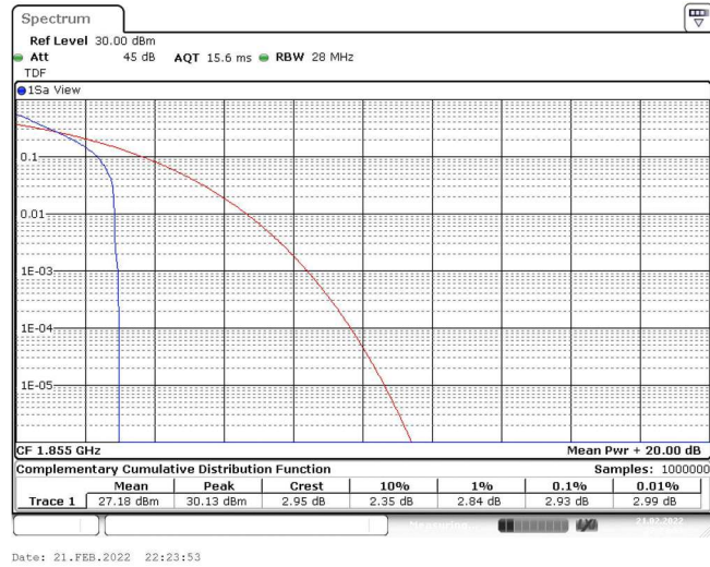
Band25-10MHz-QPSK-26090-1RB#0
