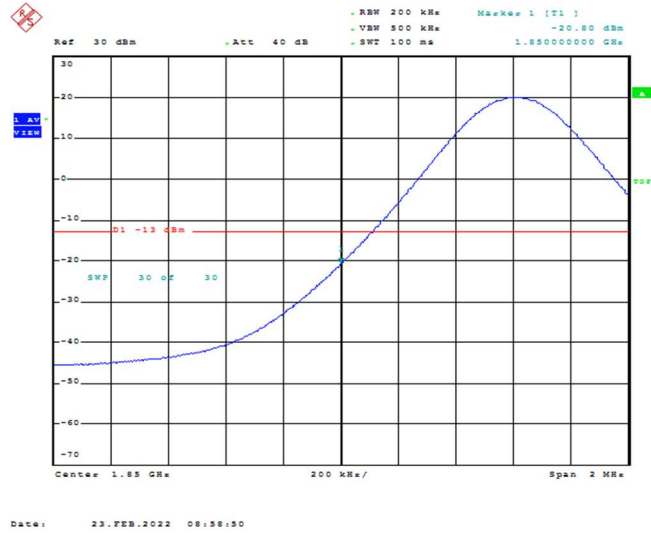
Band25-10MHz-QPSK-26090-1RB#0
