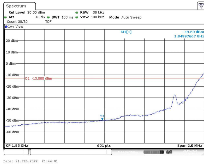
Band25-1.4MHz-16QAM-26047-1RB#5
