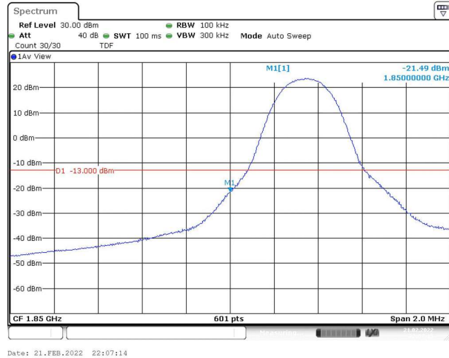
Band25-5MHz-16QAM-26065-1RB#0
