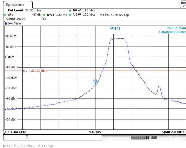
Band25-1.4MHz-16QAM-26047-1RB#0
