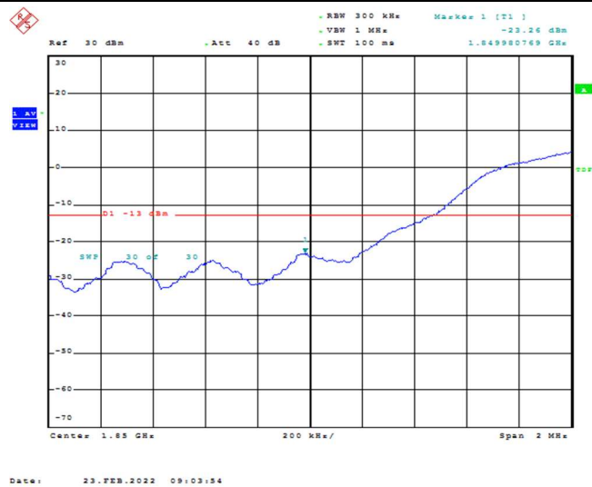
Band25-15MHz-QPSK-26115-75RB#0
