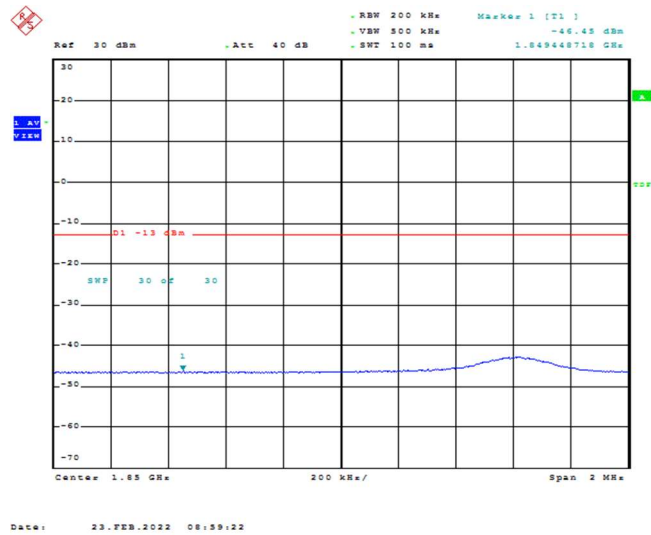
Band25-10MHz-16QAM-26090-1RB#49
