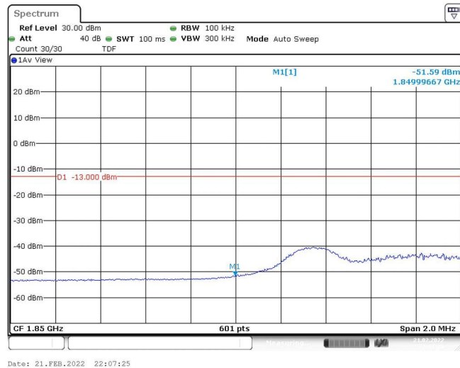
Band25-5MHz-QPSK-26065-1RB#24
