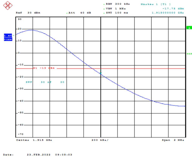
Band25-15MHz-16QAM-26615-1RB#74
