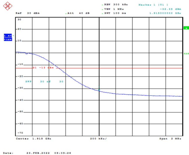
Band25-15MHz-16QAM-26615-75RB#0
