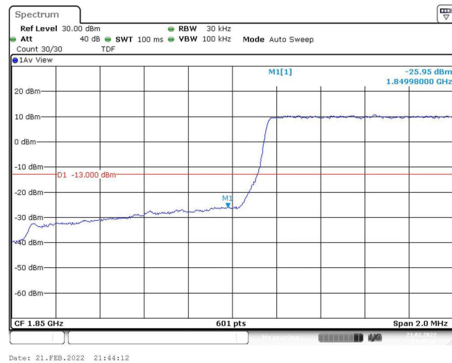
Band25-1.4MHz-QPSK-26047-6RB#0
