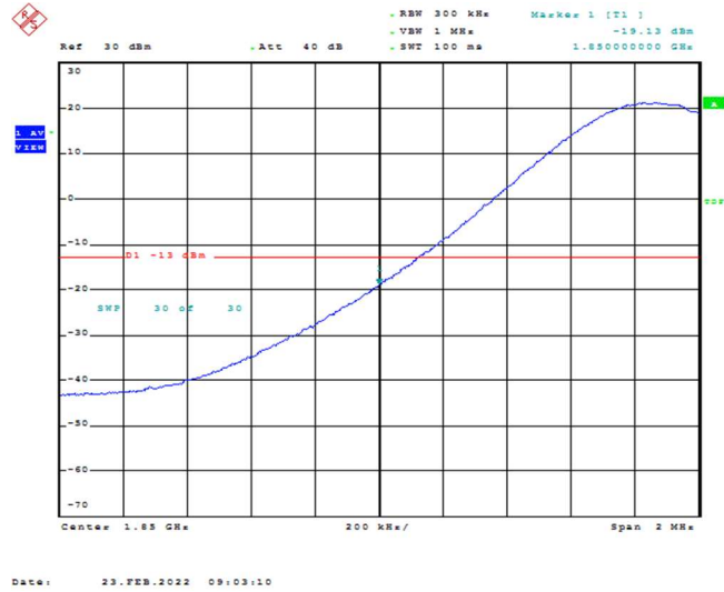
Band25-15MHz-QPSK-26115-1RB#0
