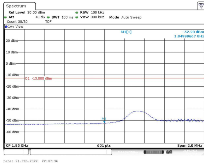
Band25-5MHz-16QAM-26065-1RB#24
