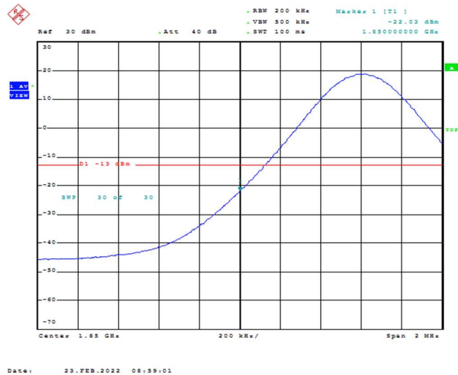
Band25-10MHz-16QAM-26090-1RB#0
