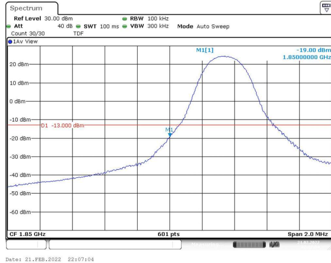
Band25-5MHz-QPSK-26065-1RB#0
