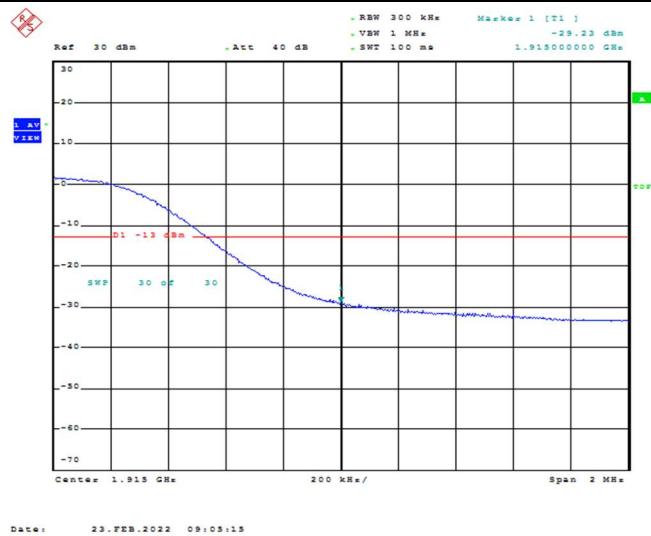
Band25-15MHz-QPSK-26615-75RB#0
