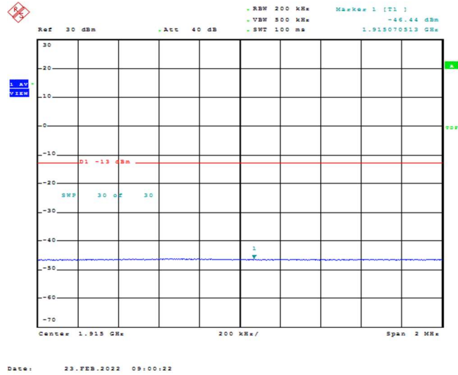
Band25-10MHz-16QAM-26640-1RB#0
