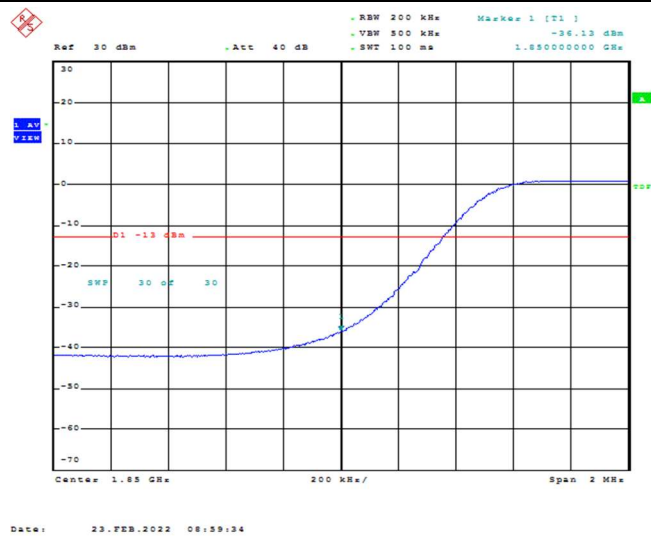
Band25-10MHz-QPSK-26090-50RB#0
