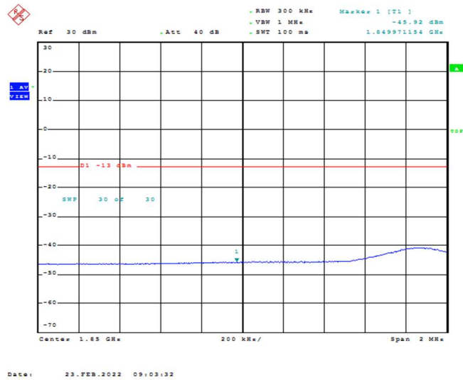
Band25-15MHz-QPSK-26115-1RB#74
