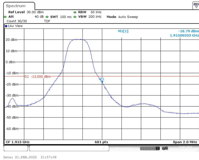
Band25-3MHz-16QAM-26675-1RB#14
