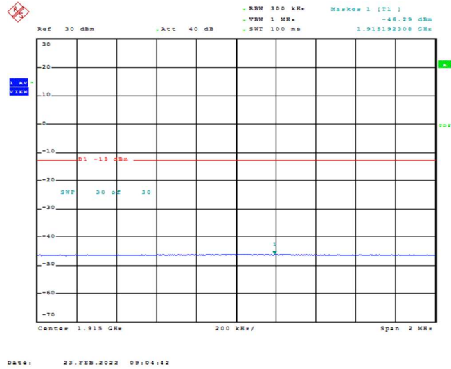
Band25-15MHz-16QAM-26615-1RB#0
