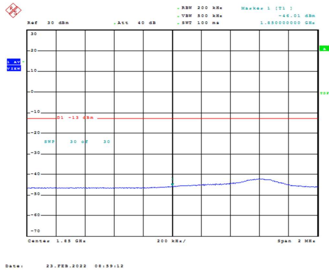
Band25-10MHz-QPSK-26090-1RB#49
