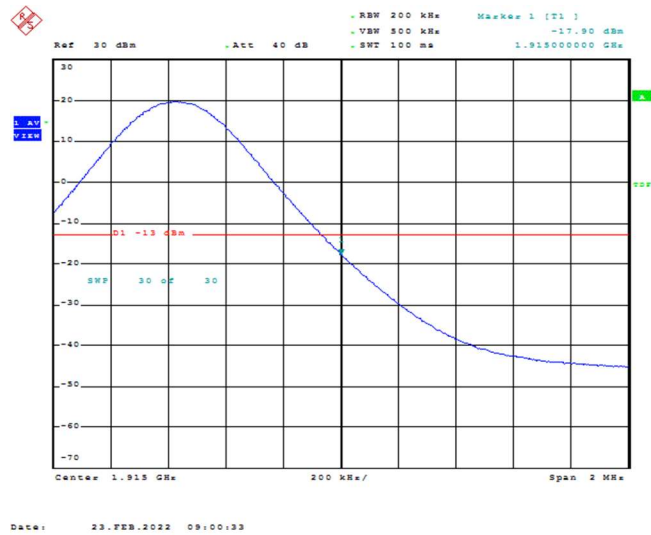
Band25-10MHz-QPSK-26640-1RB#49
