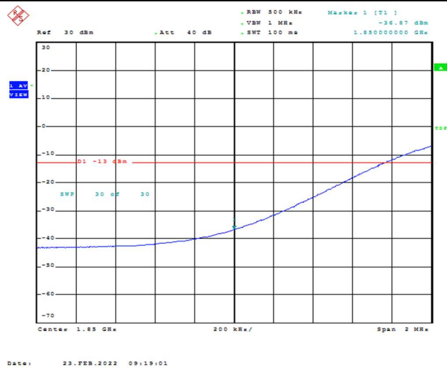
Band25-20MHz-QPSK-26140-100RB#0
