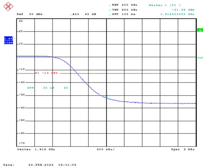
Band25-10MHz-16QAM-26640-50RB#0
