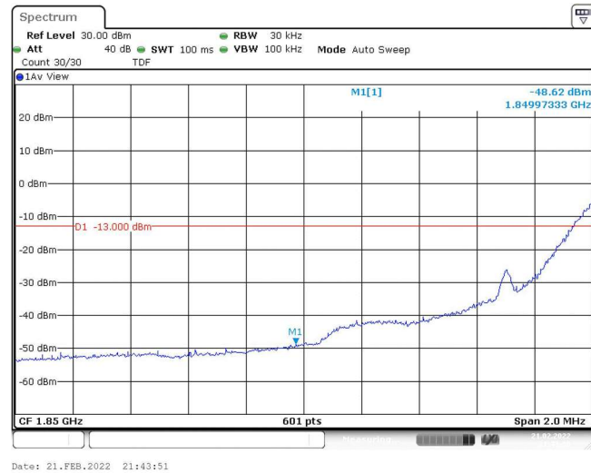
Band25-1.4MHz-QPSK-26047-1RB#5
