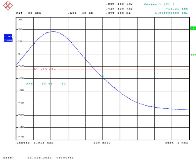
Band25-10MHz-16QAM-26640-1RB#49
