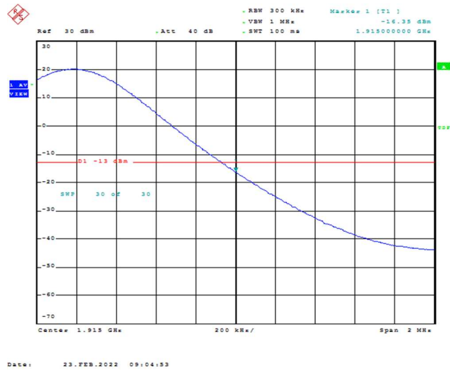
Band25-15MHz-QPSK-26615-1RB#74
