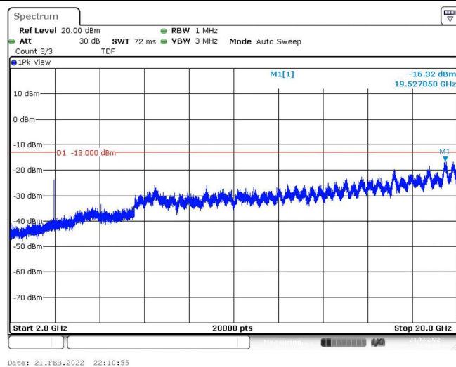
Band25-5MHz-QPSK-26365-1RB#0-Range3:2000~20000MHz
