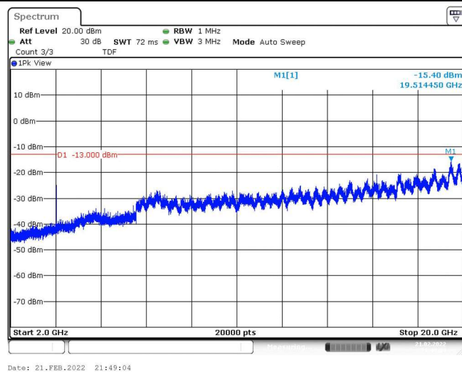
Band25-1.4MHz-QPSK-26683-1RB#0-Range3:2000~20000MHz
