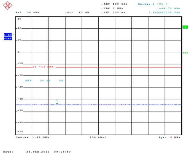
Band25-20MHz-16QAM-26140-1RB#99
