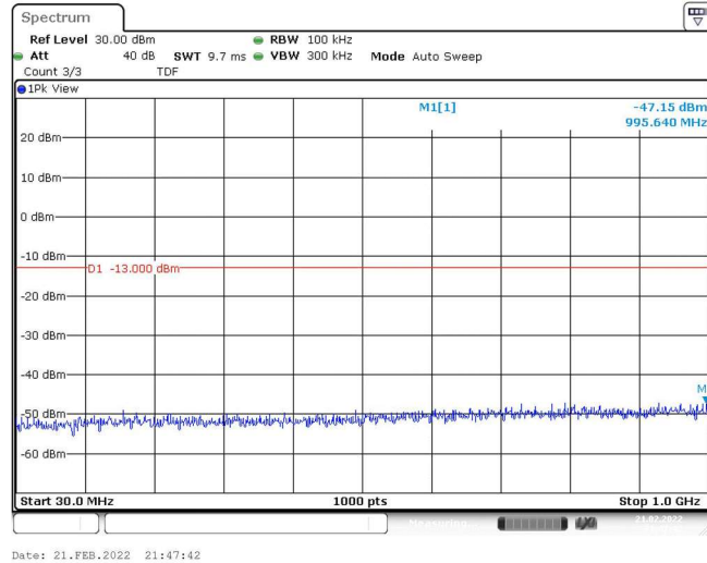
Band25-1.4MHz-QPSK-26365-1RB#0-Range1:30~1000MHz
