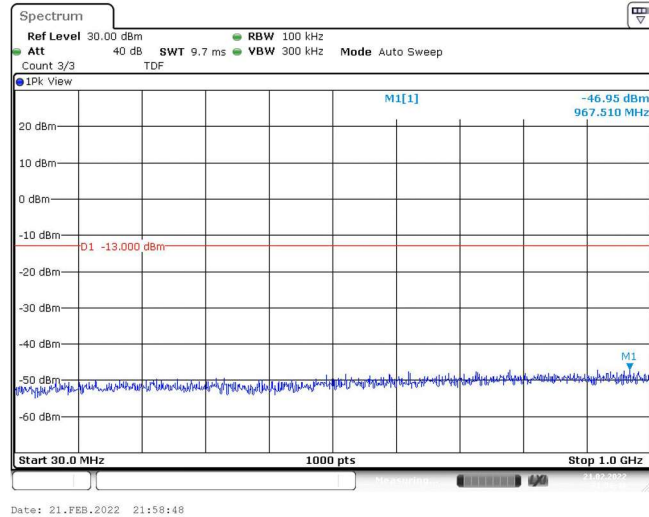
Band25-3MHz-QPSK-26365-1RB#0-Range1:30~1000MHz
