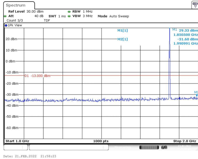
Band25-3MHz-16QAM-26055-1RB#0-Range2:1000~2000MHz
