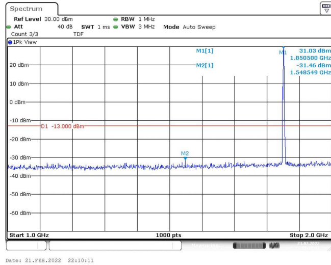
Band25-5MHz-16QAM-26065-1RB#0-Range2:1000~2000MHz
