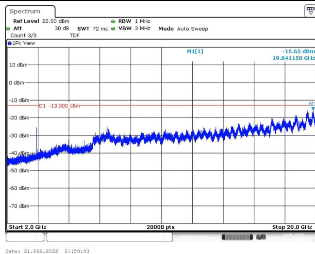
Band25-3MHz-QPSK-26055-1RB#0-Range3:2000~20000MHz
