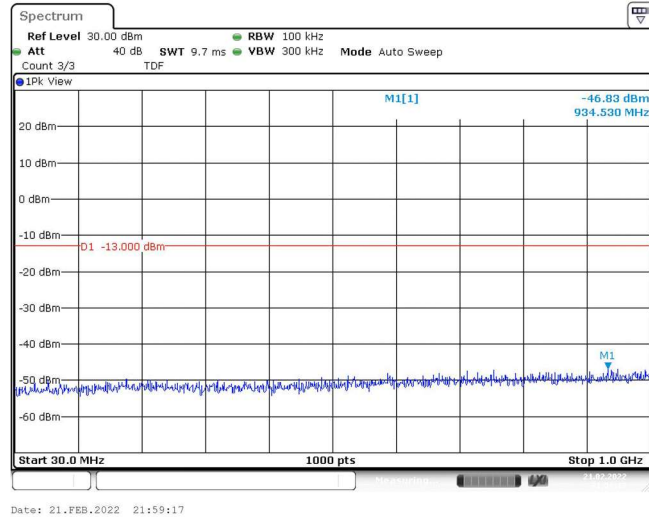
Band25-3MHz-16QAM-26365-1RB#0-Range1:30~1000MHz
