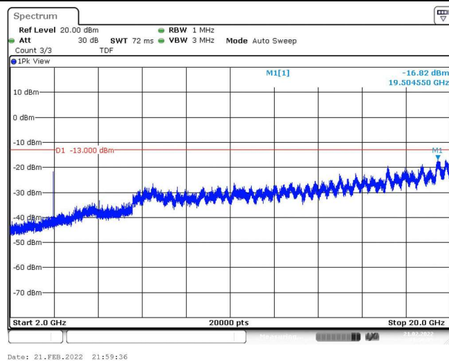
Band25-3MHz-16QAM-26365-1RB#0-Range3:2000~20000MHz
