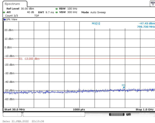
Band25-5MHz-QPSK-26365-1RB#0-Range1:30~1000MHz
