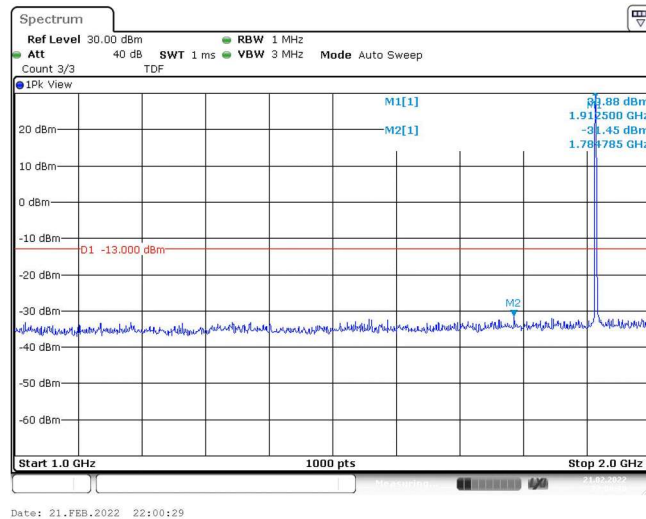
Band25-3MHz-16QAM-26675-1RB#0-Range2:1000~2000MHz
