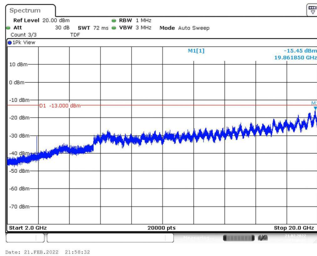
Band25-3MHz-16QAM-26055-1RB#0-Range3:2000~20000MHz
