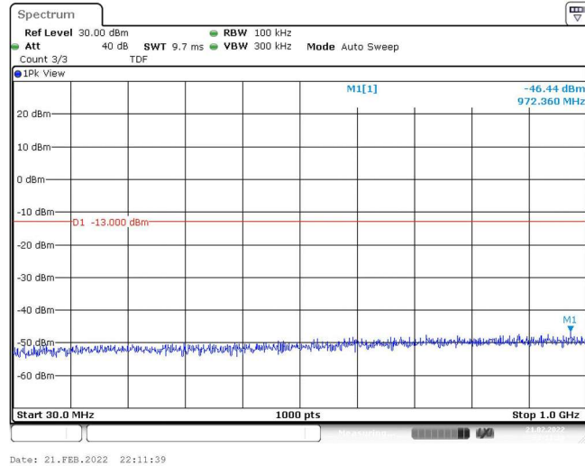
Band25-5MHz-QPSK-26665-1RB#0-Range1:30~1000MHz
