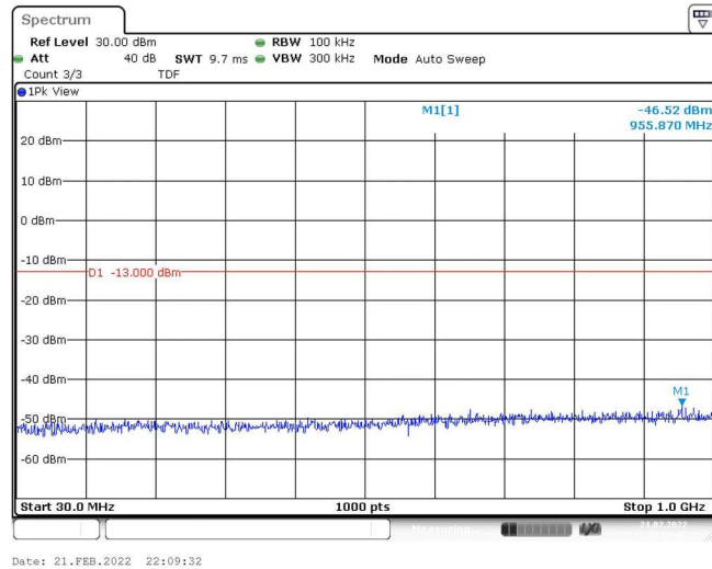
Band25-5MHz-QPSK-26065-1RB#0-Range1:30~1000MHz
