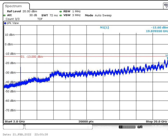
Band25-3MHz-16QAM-26675-1RB#0-Range3:2000~20000MHz
