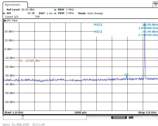
Band25-5MHz-QPSK-26665-1RB#0-Range2:1000~2000MHz
