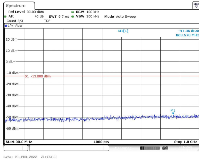
Band25-1.4MHz-QPSK-26047-1RB#0-Range1:30~1000MHz
