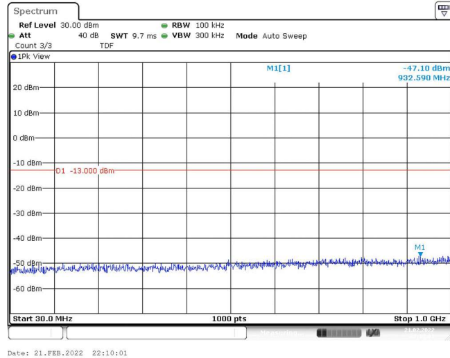
Band25-5MHz-16QAM-26065-1RB#0-Range1:30~1000MHz
