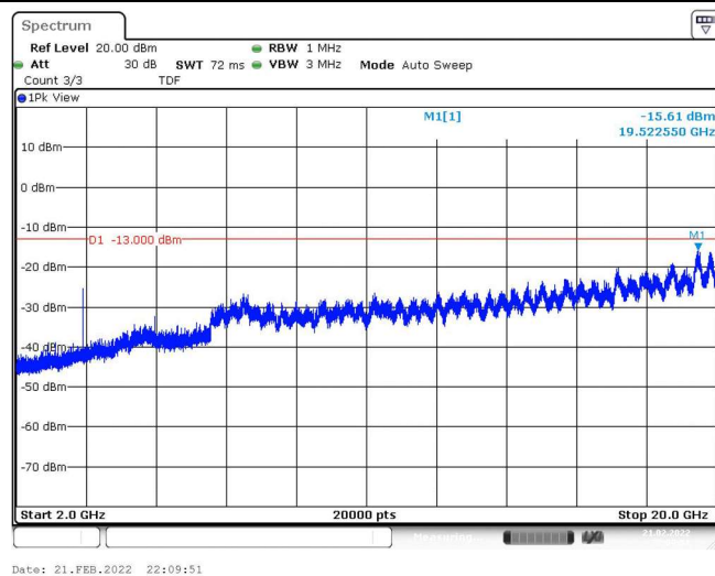
Band25-5MHz-QPSK-26065-1RB#0-Range3:2000~20000MHz
