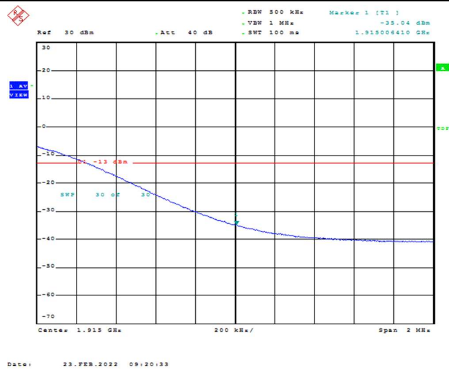
Band25-20MHz-16QAM-26590-100RB#0
