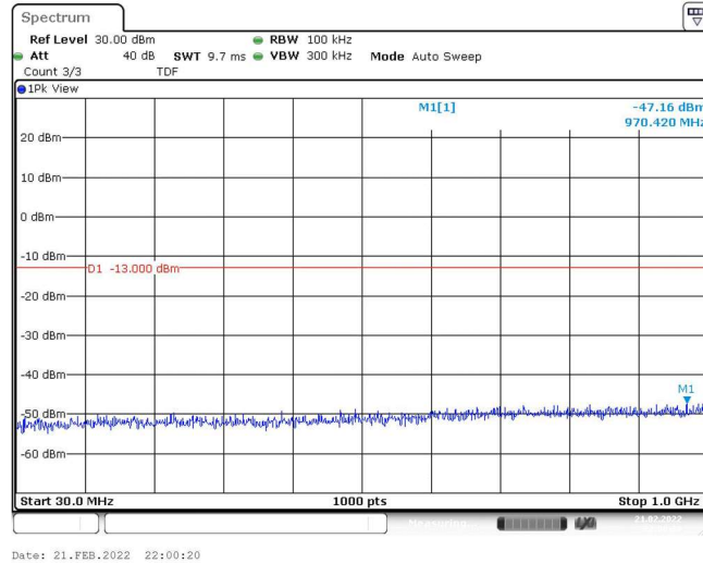
Band25-3MHz-16QAM-26675-1RB#0-Range1:30~1000MHz
