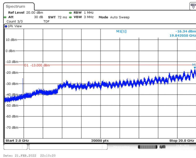
Band25-5MHz-16QAM-26065-1RB#0-Range3:2000~20000MHz
