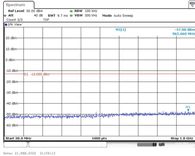
Band25-3MHz-16QAM-26055-1RB#0-Range1:30~1000MHz
