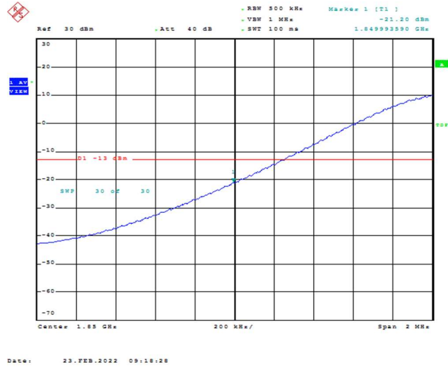
Band25-20MHz-16QAM-26140-1RB#0
