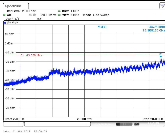
Band25-3MHz-QPSK-26675-1RB#0-Range3:2000~20000MHz
