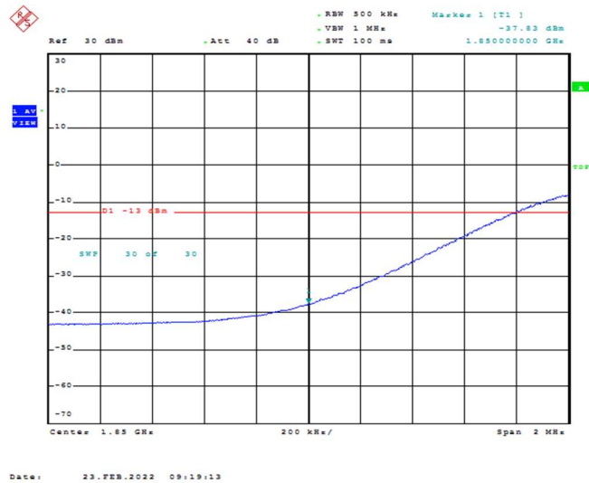
Band25-20MHz-16QAM-26140-100RB#0
