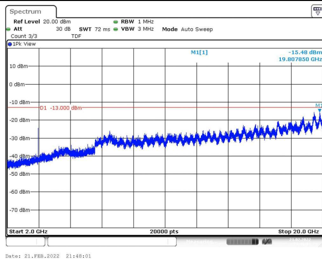
Band25-1.4MHz-QPSK-26365-1RB#0-Range3:2000~20000MHz
