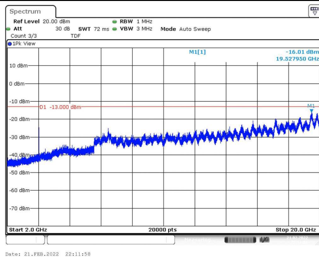
Band25-5MHz-QPSK-26665-1RB#0-Range3:2000~20000MHz
