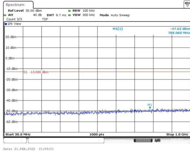
Band25-3MHz-QPSK-26675-1RB#0-Range1:30~1000MHz
