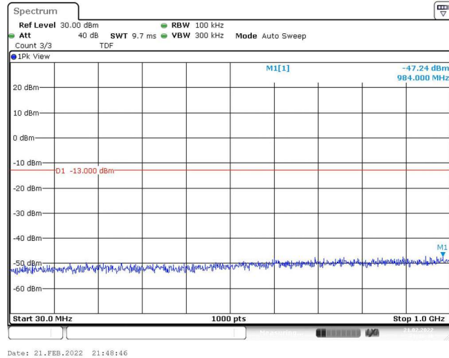
Band25-1.4MHz-QPSK-26683-1RB#0-Range1:30~1000MHz
