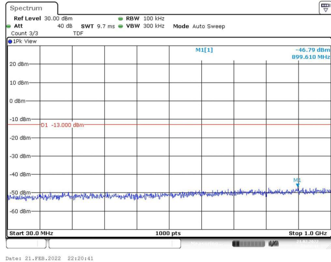
Band25-10MHz-QPSK-26090-1RB#0-Range1:30~1000MHz
