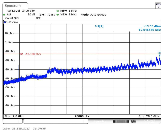
Band25-10MHz-QPSK-26090-1RB#0-Range3:2000~20000MHz
