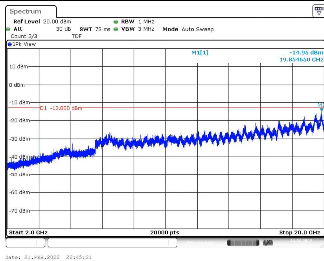
Band25-20MHz-QPSK-26590-1RB#0-Range3:2000~20000MHz
