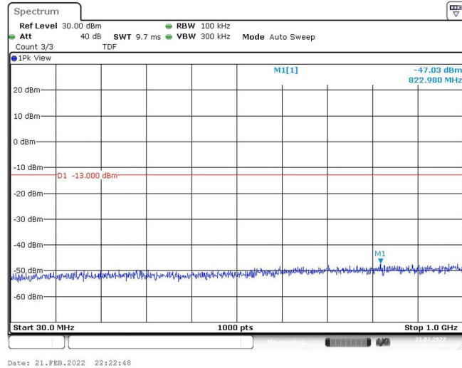
Band25-10MHz-QPSK-26640-1RB#0-Range1:30~1000MHz
