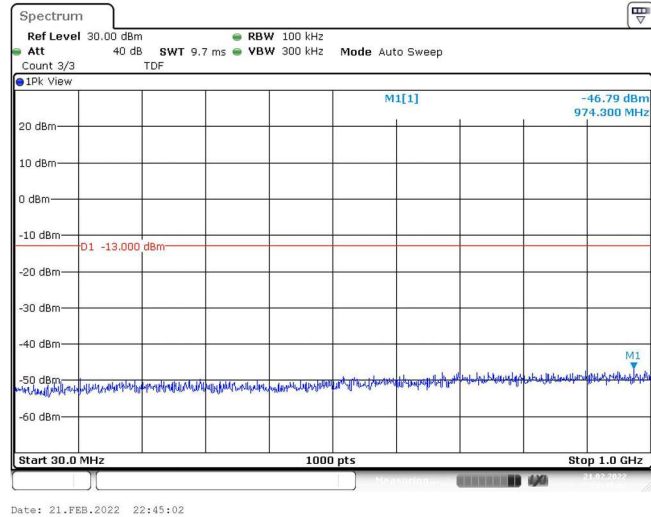
Band25-20MHz-QPSK-26590-1RB#0-Range1:30~1000MHz
