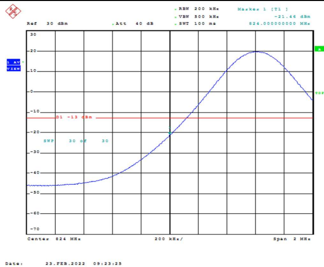
Band26-10MHz-QPSK-26840-1RB#0
