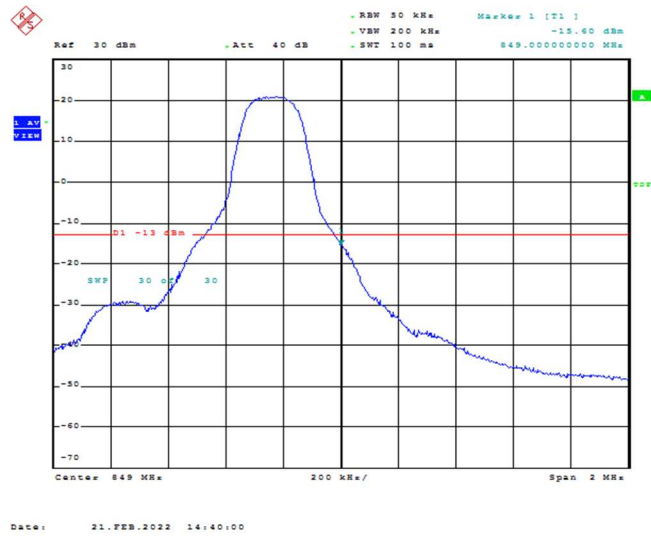
Band26-3MHz-QPSK-27025-1RB#14
