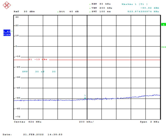
Band26-3MHz-16QAM-26805-1RB#14
