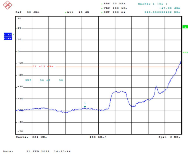
Band26-1.4MHz-16QAM-26797-1RB#5
