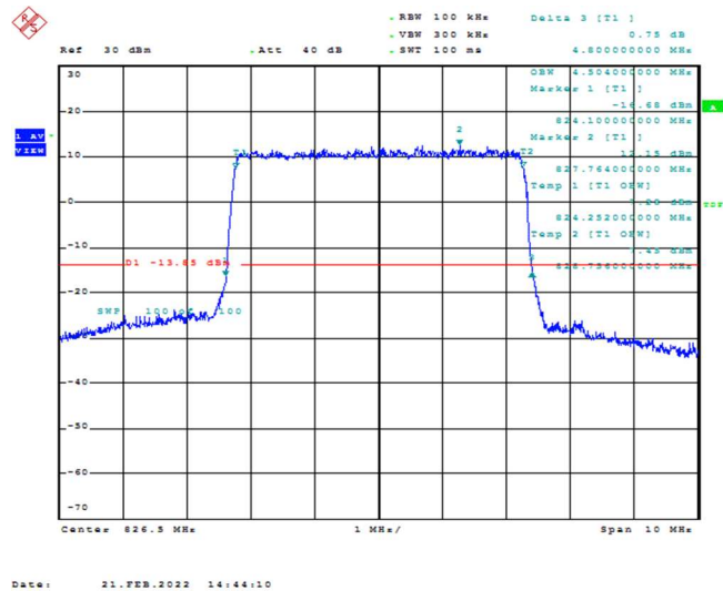
Band26-5MHz-16QAM-26815-25RB#0-4.504
