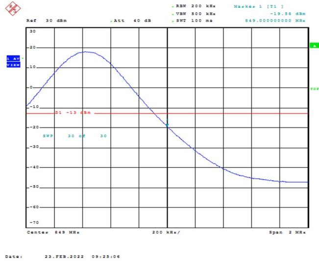
Band26-10MHz-QPSK-26990-1RB#49
