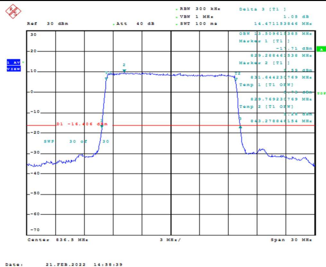
Band26-15MHz-16QAM-26915-75RB#0-13.51
