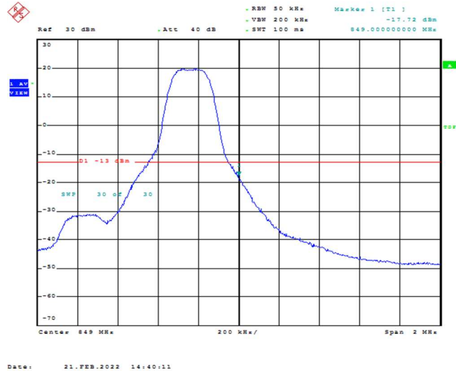
Band26-3MHz-16QAM-27025-1RB#14
