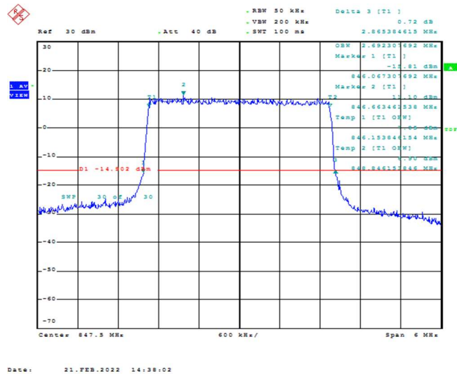
Band26-3MHz-16QAM-27025-15RB#0-2.692
