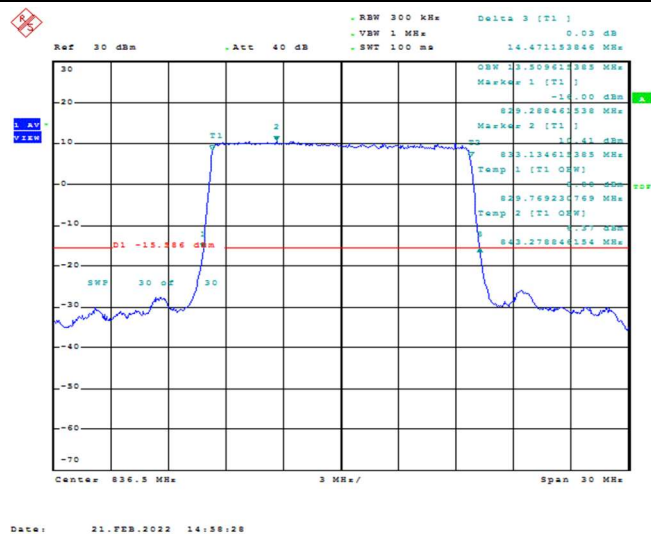
Band26-15MHz-QPSK-26915-75RB#0-13.51
