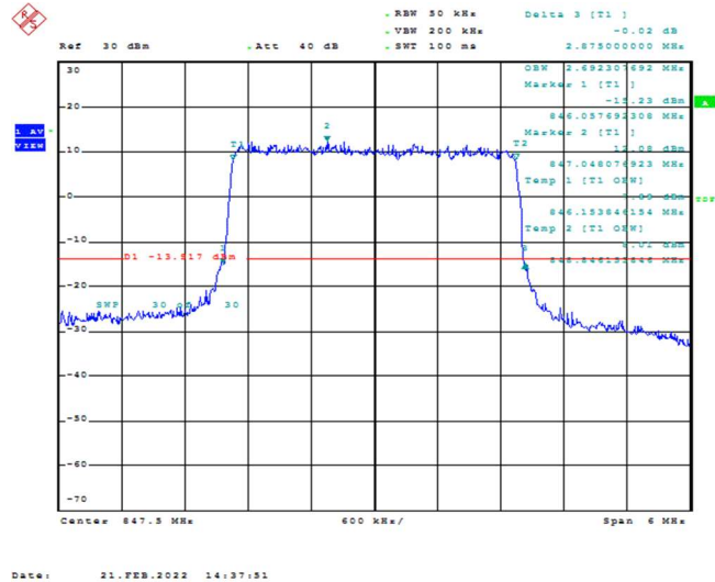
Band26-3MHz-QPSK-27025-15RB#0-2.692
