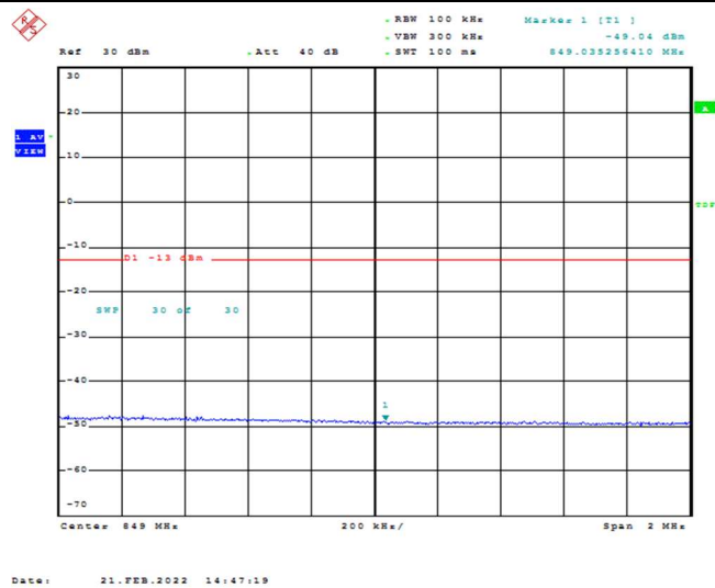
Band26-5MHz-16QAM-27015-1RB#0
