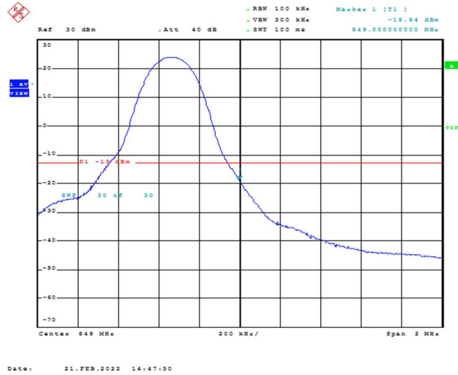
Band26-5MHz-QPSK-27015-1RB#24
