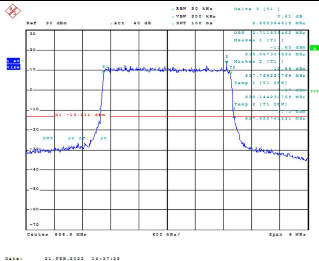
Band26-3MHz-QPSK-26915-15RB#0-2.712
