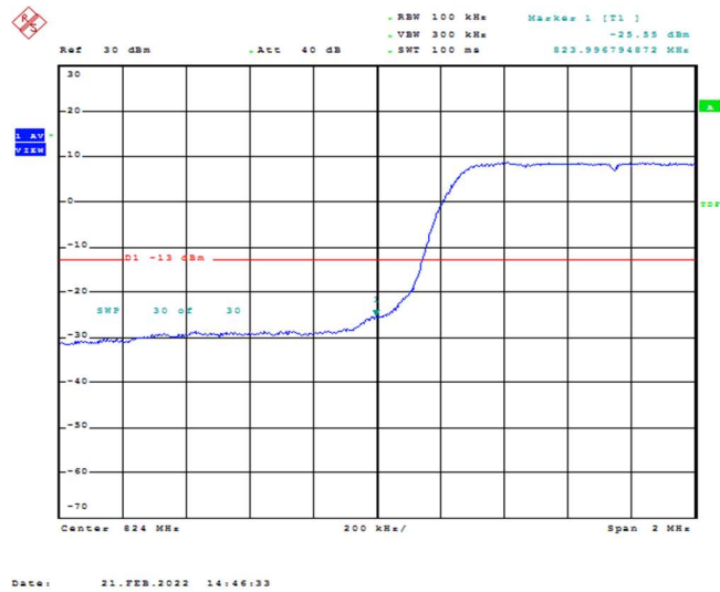
Band26-5MHz-QPSK-26815-25RB#0
