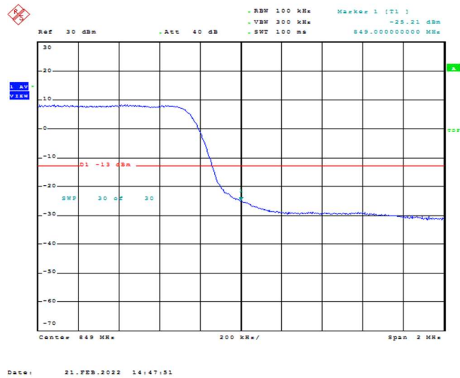
Band26-5MHz-QPSK-27015-25RB#0
