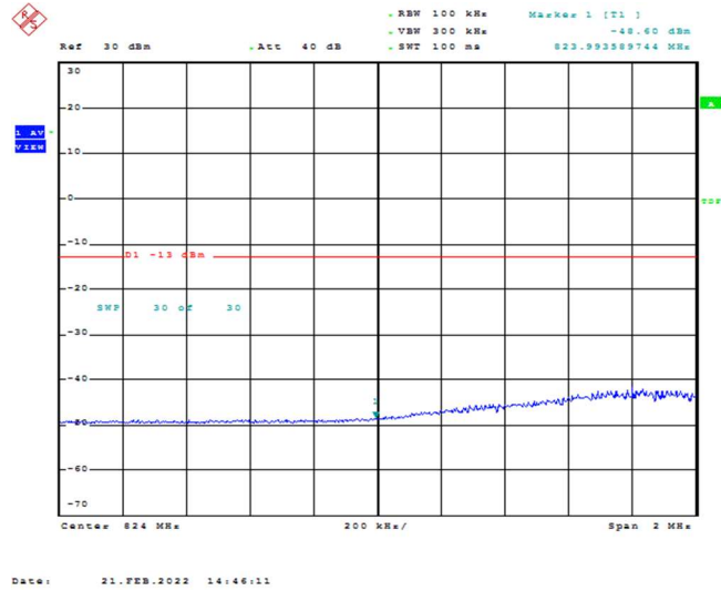
Band26-5MHz-QPSK-26815-1RB#24
