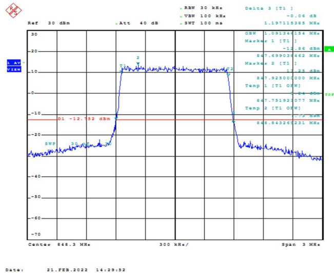
Band26-1.4MHz-16QAM-27033-6RB#0-1.091
