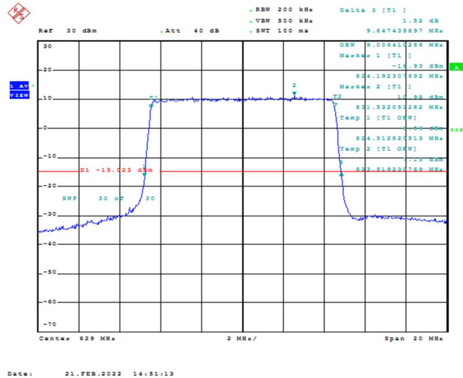
Band26-10MHz-QPSK-26840-50RB#0-9.006
