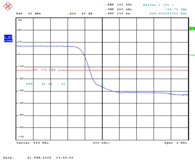
Band26-5MHz-16QAM-27015-25RB#0
