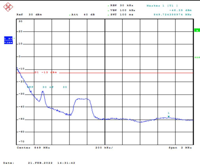
Band26-1.4MHz-16QAM-27033-1RB#0
