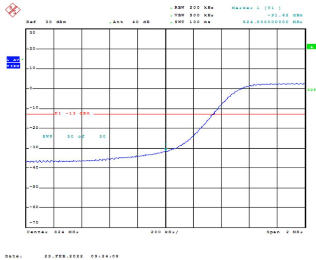
Band26-10MHz-QPSK-26840-50RB#0
