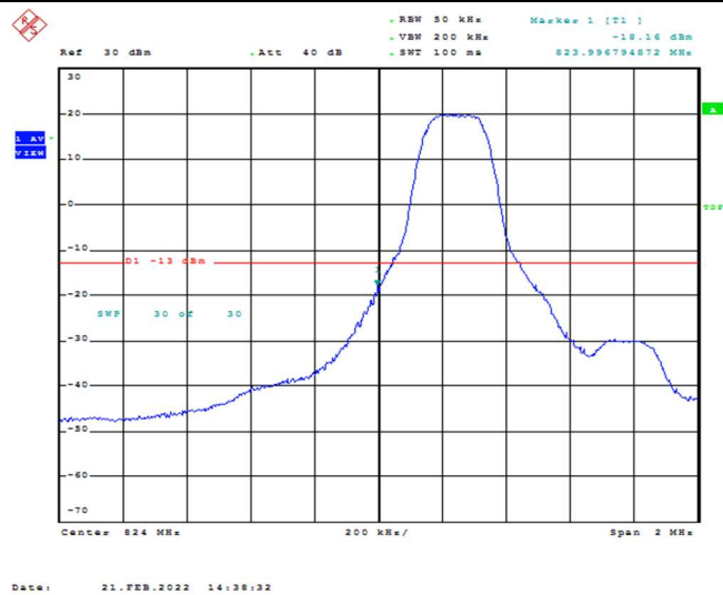
Band26-3MHz-16QAM-26805-1RB#0
