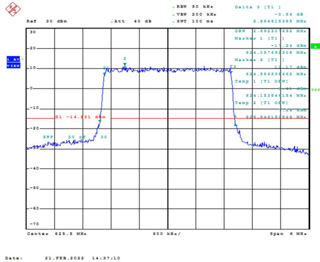
Band26-3MHz-16QAM-26805-15RB#0-2.692
