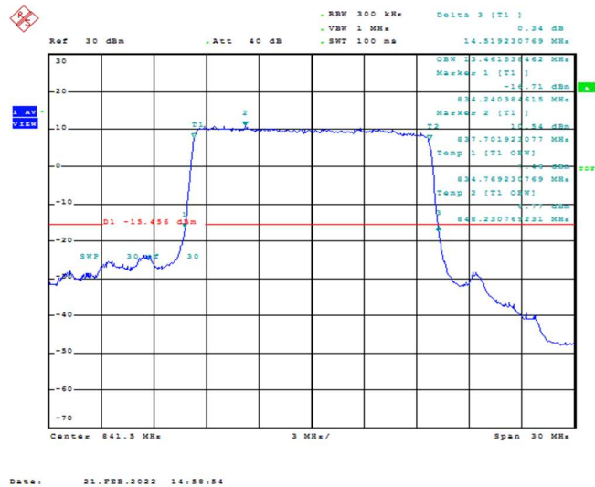
Band26-15MHz-QPSK-26965-75RB#0-13.462
