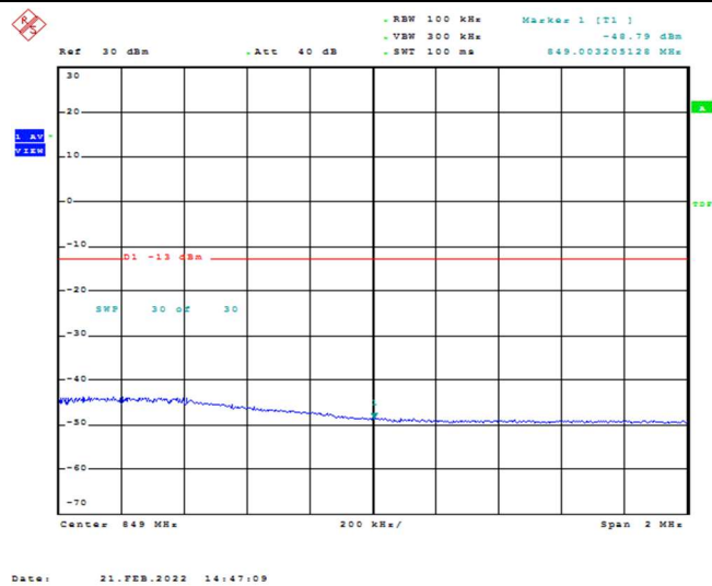
Band26-5MHz-QPSK-27015-1RB#0
