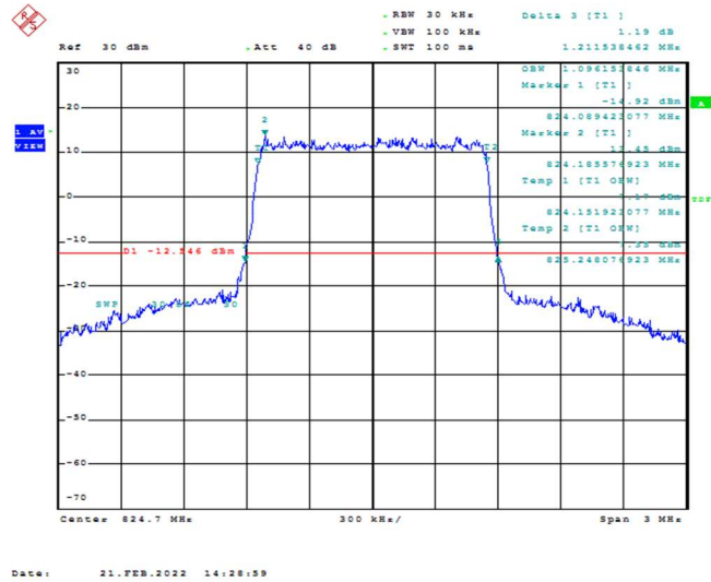
Band26-1.4MHz-16QAM-26797-6RB#0-1.096
