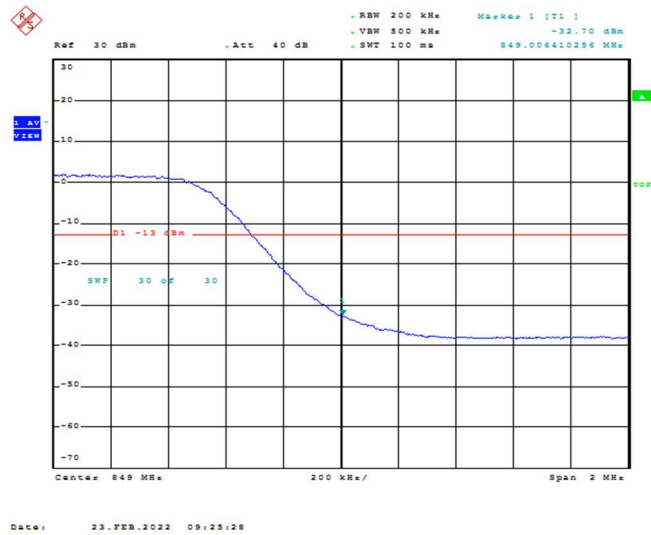
Band26-10MHz-QPSK-26990-50RB#0
