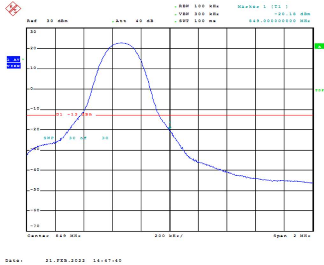
Band26-5MHz-16QAM-27015-1RB#24
