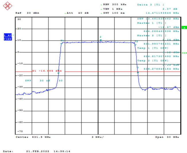
Band26-15MHz-16QAM-26865-75RB#0-13.462
