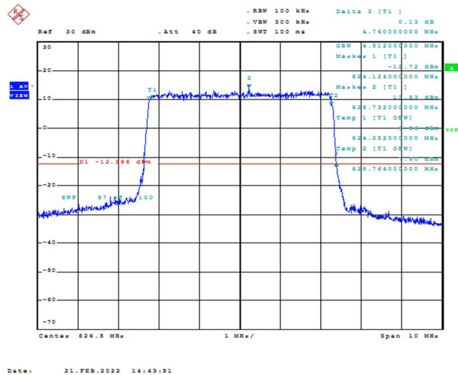
Band26-5MHz-QPSK-26815-25RB#0-4.512
