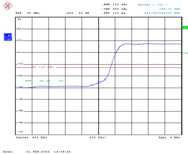
Band26-5MHz-16QAM-26815-25RB#0
