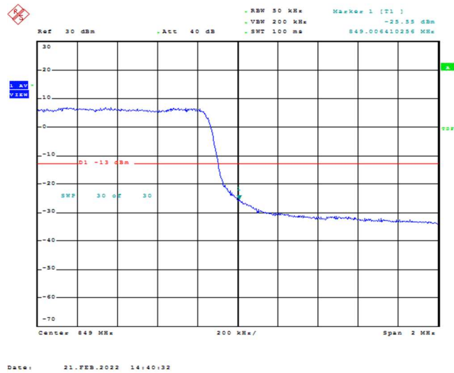
Band26-3MHz-16QAM-27025-15RB#0
