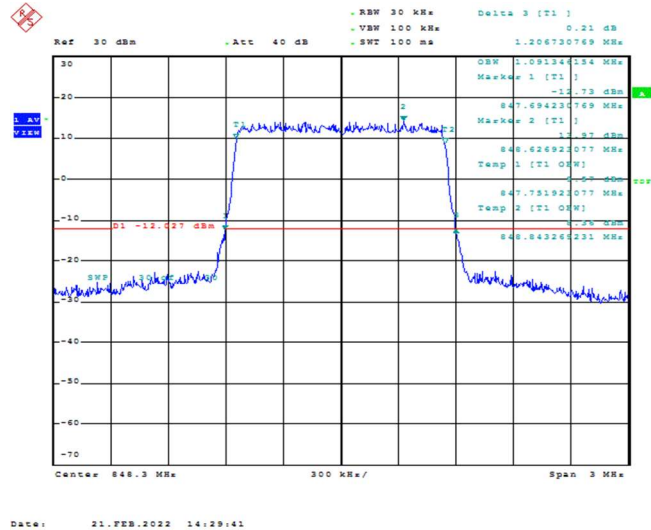
Band26-1.4MHz-QPSK-27033-6RB#0-1.091
