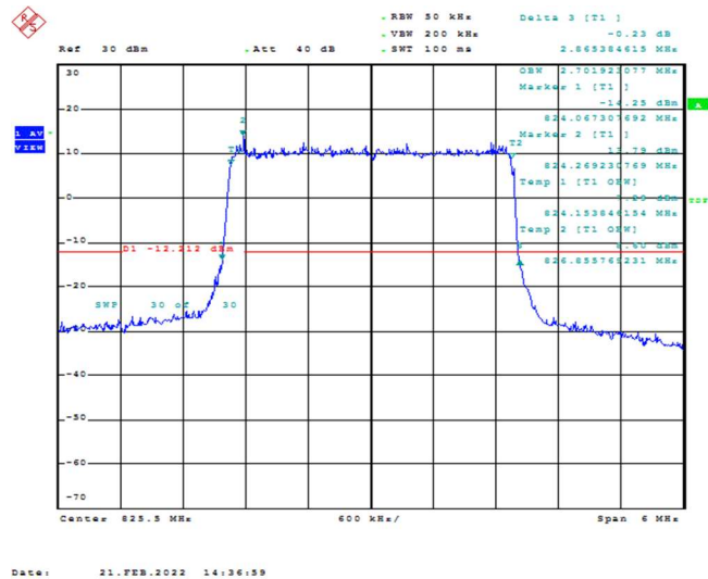
Band26-3MHz-QPSK-26805-15RB#0-2.702
