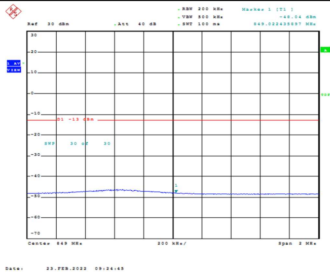
Band26-10MHz-QPSK-26990-1RB#0
