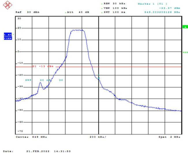
Band26-1.4MHz-QPSK-27033-1RB#5
