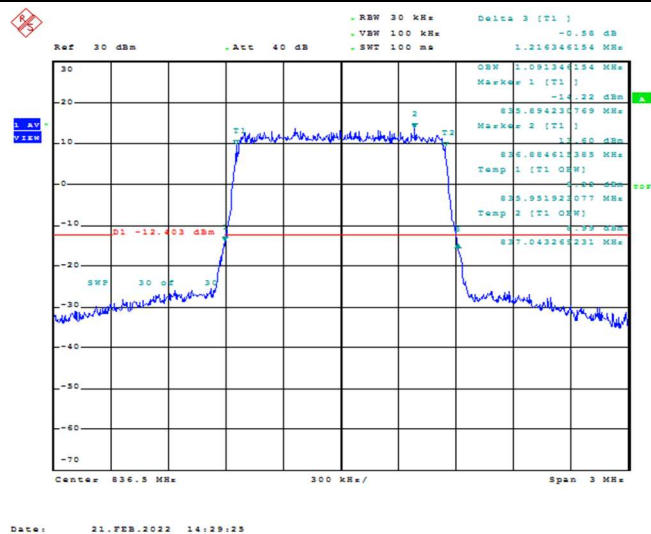
Band26-1.4MHz-16QAM-26915-6RB#0-1.091
