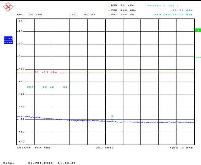
Band26-3MHz-16QAM-27025-1RB#0
