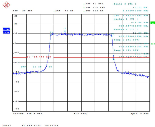
Band26-3MHz-16QAM-26915-15RB#0-2.692
