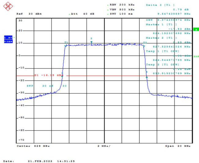
Band26-10MHz-16QAM-26840-50RB#0-8.974
