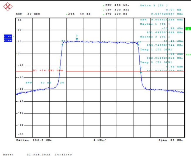
Band26-10MHz-QPSK-26915-50RB#0-9.006
