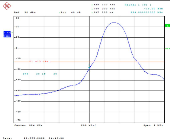
Band26-5MHz-QPSK-26815-1RB#0
