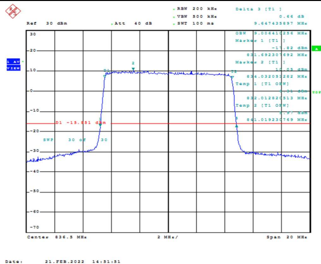
Band26-10MHz-16QAM-26915-50RB#0-9.006
