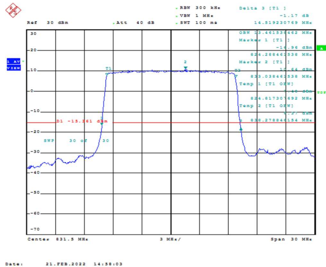
Band26-15MHz-QPSK-26865-75RB#0-13.462
