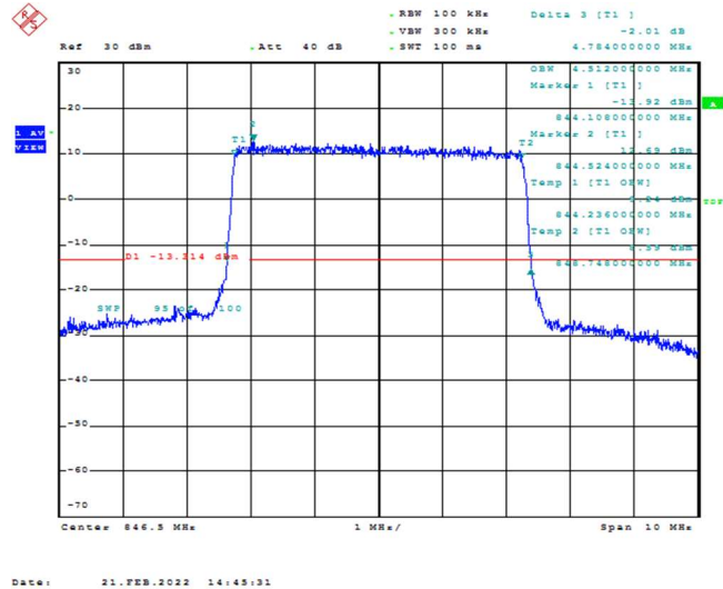
Band26-5MHz-16QAM-27015-25RB#0-4.512
