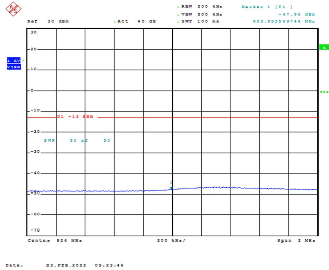
Band26-10MHz-QPSK-26840-1RB#49
