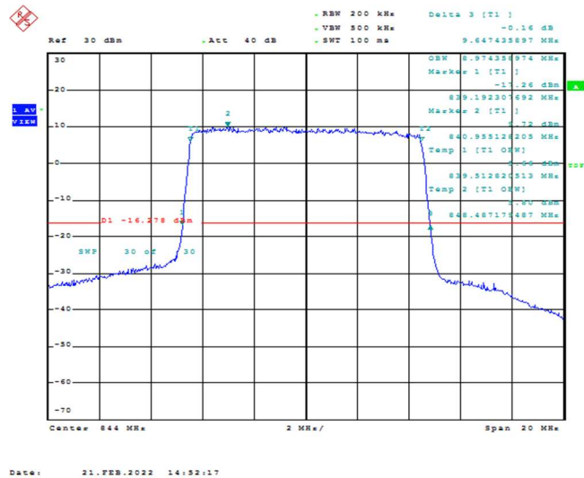
Band26-10MHz-16QAM-26990-50RB#0-8.974
