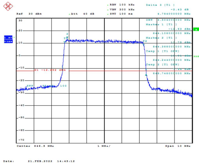
Band26-5MHz-QPSK-27015-25RB#0-4.504
