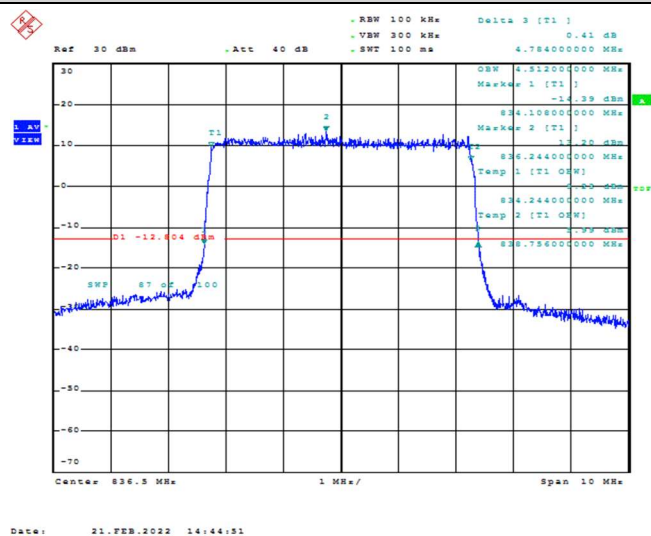
Band26-5MHz-16QAM-26915-25RB#0-4.512
