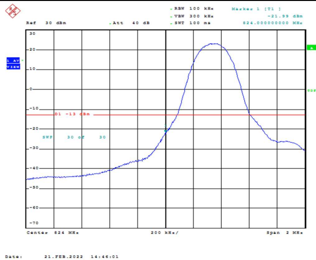
Band26-5MHz-16QAM-26815-1RB#0
