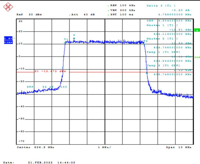
Band26-5MHz-QPSK-26915-25RB#0-4.504
