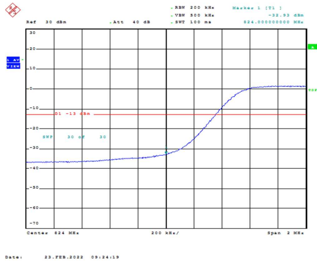
Band26-10MHz-16QAM-26840-50RB#0
