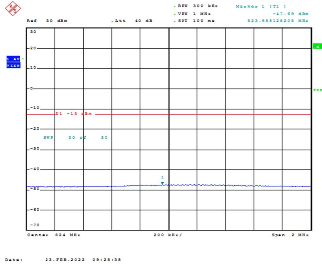
Band26-15MHz-QPSK-26865-1RB#74
