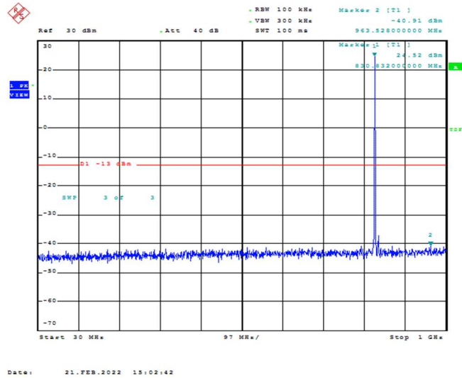
Band26-15MHz-QPSK-26915-1RB#0-Range1:30~1000MHz
