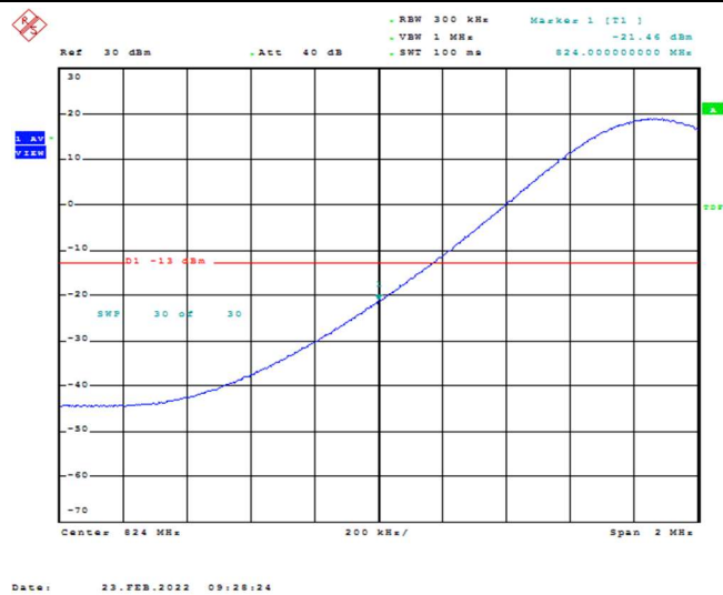
Band26-15MHz-16QAM-26865-1RB#0
