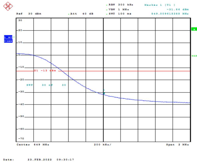
Band26-15MHz-QPSK-26965-75RB#0
