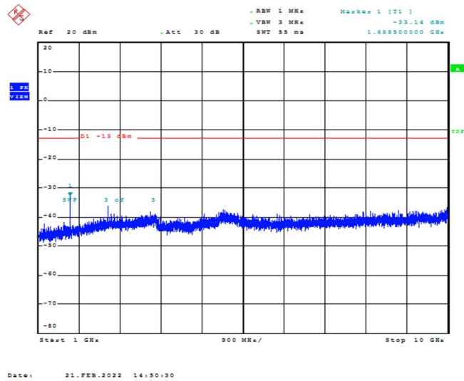
Band26-5MHz-16QAM-27015-1RB#0-Range2:1000~10000MHz
