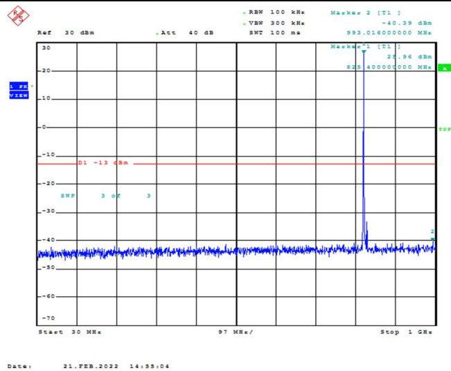
Band26-10MHz-QPSK-26840-1RB#0-Range1:30~1000MHz
