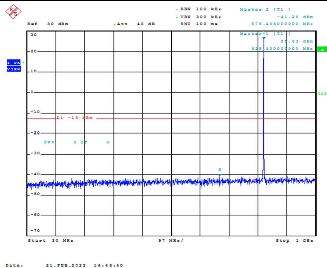
Band26-5MHz-16QAM-26815-1RB#0-Range1:30~1000MHz
