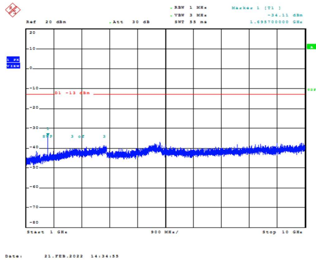
Band26-1.4MHz-16QAM-27033-1RB#0-Range2:1000~10000MHz
