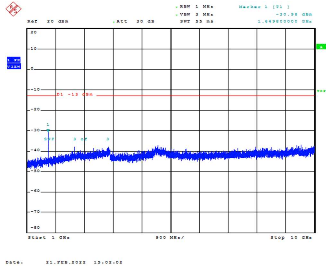
Band26-15MHz-QPSK-26865-1RB#0-Range2:1000~10000MHz
