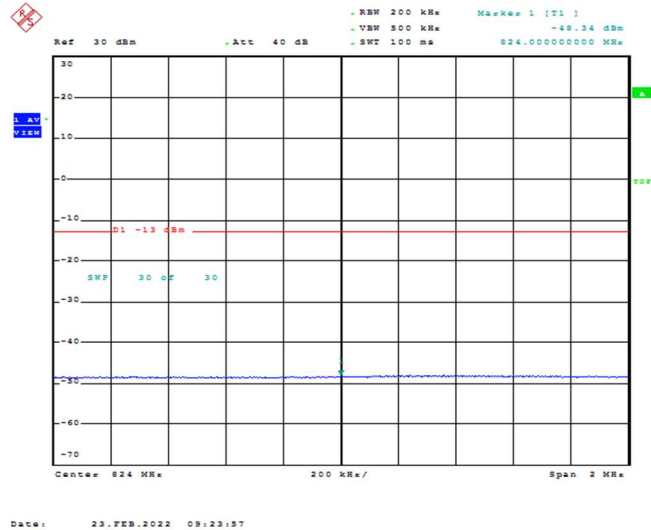
Band26-10MHz-16QAM-26840-1RB#49
