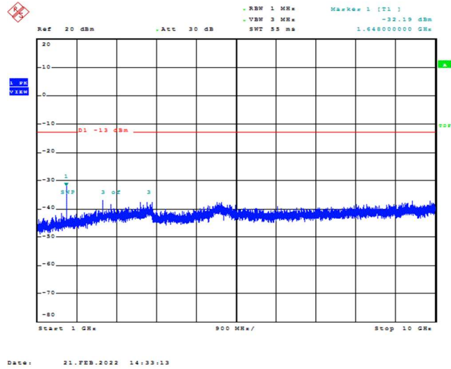
Band26-1.4MHz-16QAM-26797-1RB#0-Range2:1000~10000MHz
