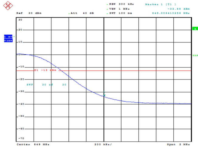
Band26-15MHz-16QAM-26965-1RB#74
