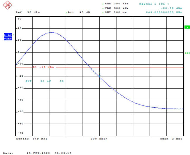
Band26-10MHz-16QAM-26990-1RB#49
