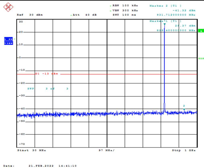
Band26-3MHz-16QAM-26805-1RB#0-Range1:30~1000MHz
