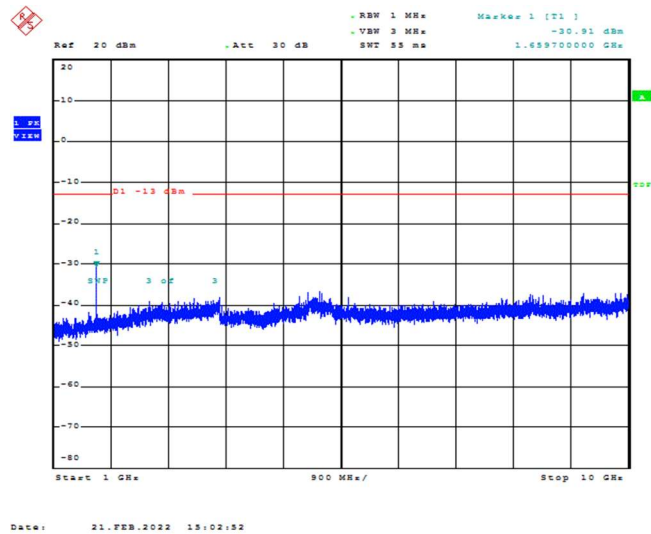
Band26-15MHz-QPSK-26915-1RB#0-Range2:1000~10000MHz
