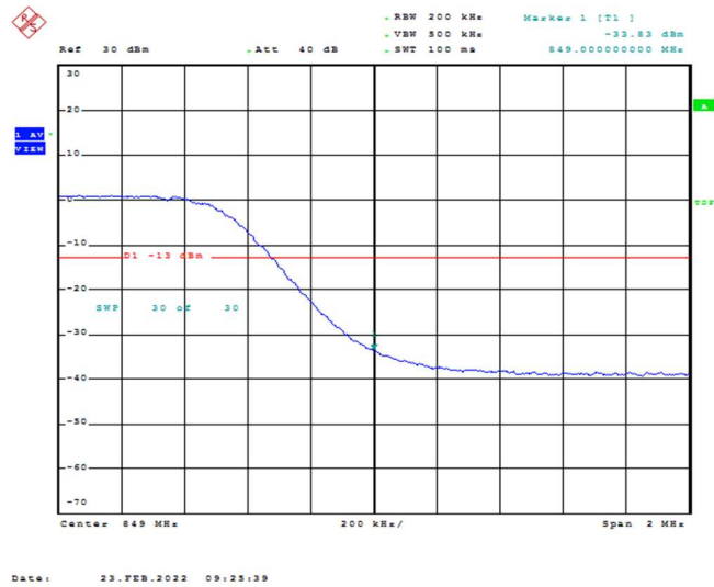
Band26-10MHz-16QAM-26990-50RB#0
