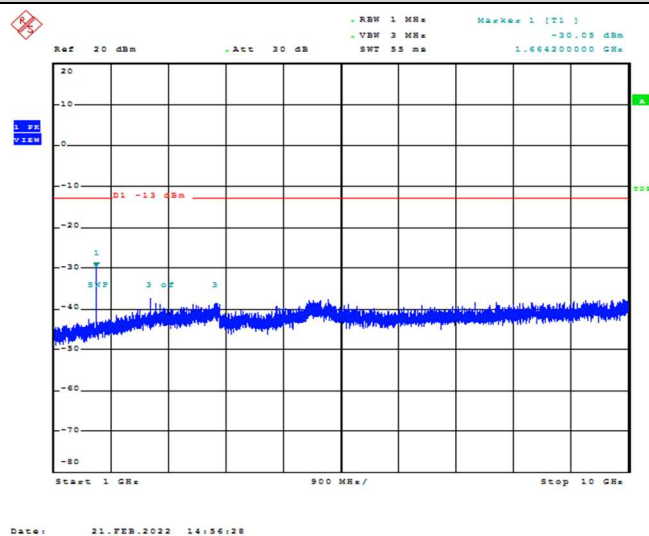
Band26-10MHz-16QAM-26915-1RB#0-Range2: 1000~10000MHz
