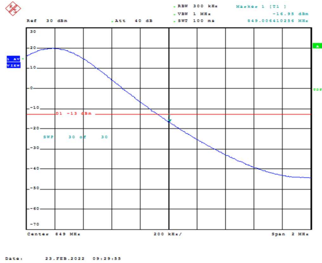
Band26-15MHz-QPSK-26965-1RB#74
