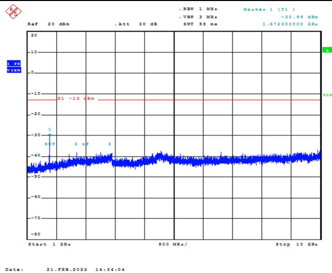
Band26-1.4MHz-16QAM-26915-1RB#0-Range2:1000~10000MHz
