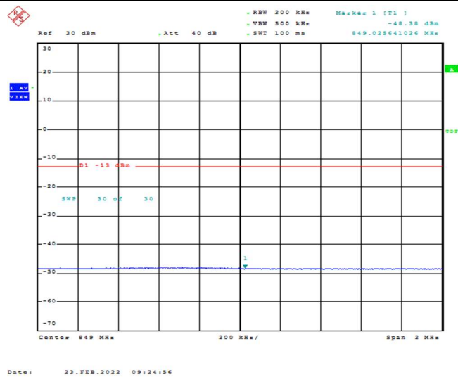
Band26-10MHz-16QAM-26990-1RB#0
