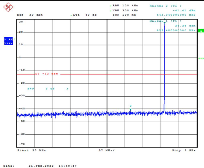
Band26-3MHz-QPSK-26805-1RB#0-Range1:30~1000MHz
