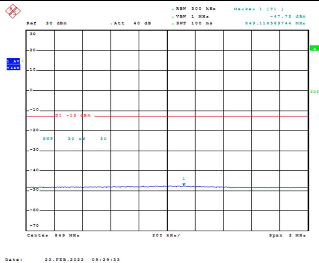
Band26-15MHz-QPSK-26965-1RB#0
