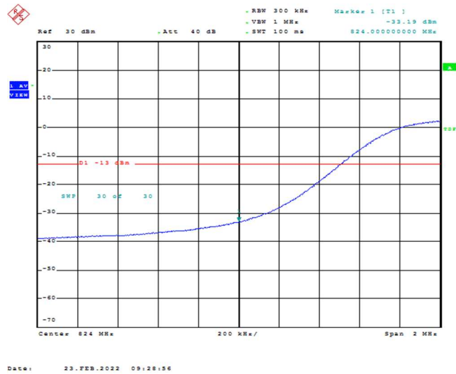
Band26-15MHz-QPSK-26865-75RB#0
