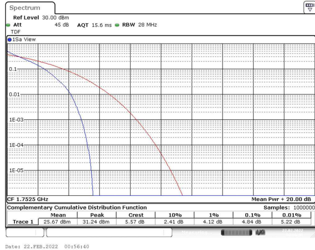
Band4-5MHz-QPSK-20375-25RB#0
