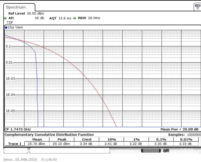
Band4-15MHz-QPSK-20325-1RB#0
