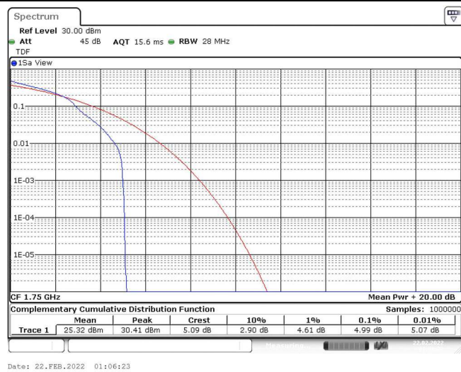
Band4-10MHz-16QAM-20350-1RB#0
