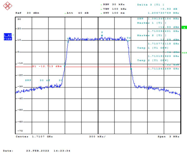
Band4-1.4MHz-16QAM-19957-6RB#0-1.091
