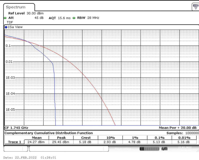
Band4-20MHz-16QAM-20300-1RB#0
