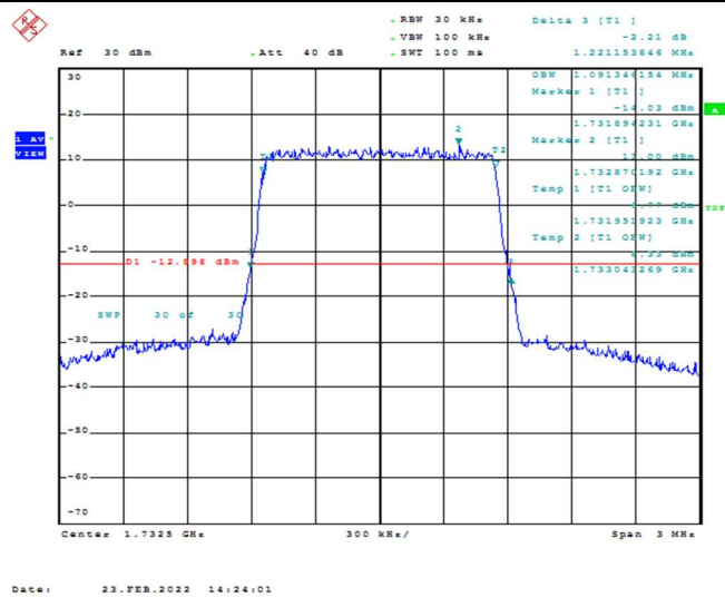
Band4-1.4MHz-16QAM-20175-6RB#0-1.091
