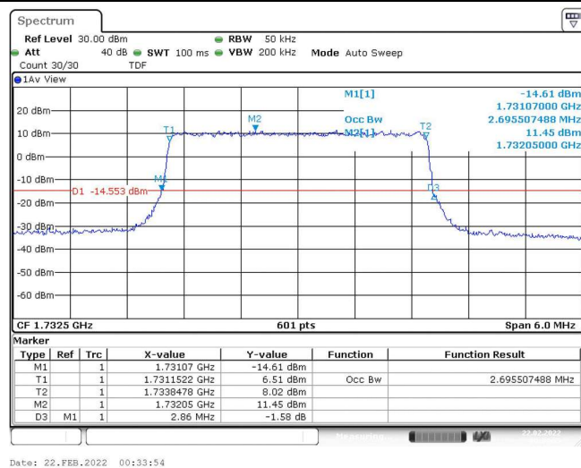
Band4-3MHz-QPSK-20175-15RB#0-2.696
