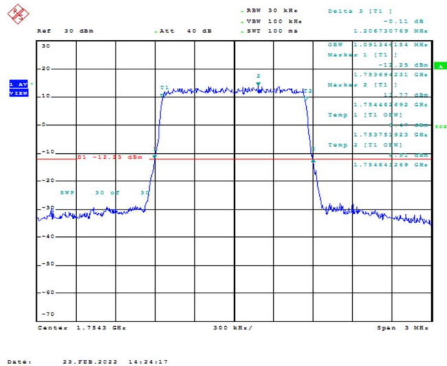
Band4-1.4MHz-QPSK-20393-6RB#0-1.091
