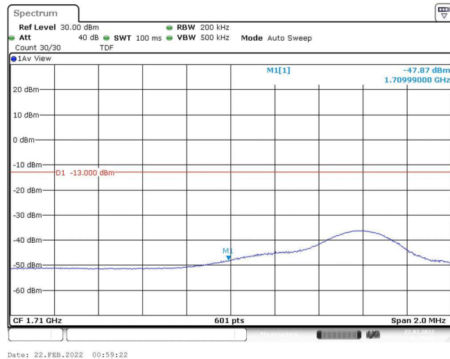
Band4-10MHz-QPSK-20000-1RB#49
