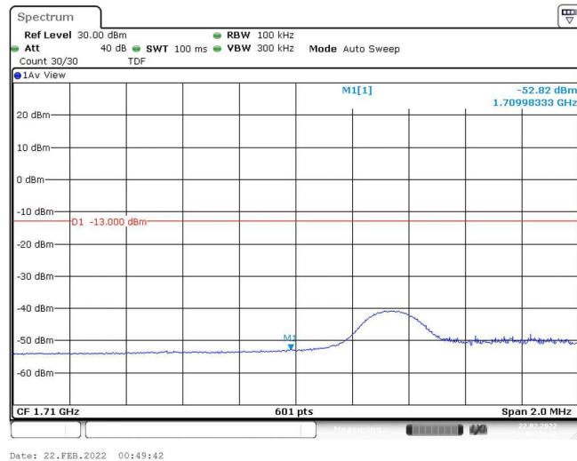
Band4-5MHz-16QAM-19975-1RB#24
