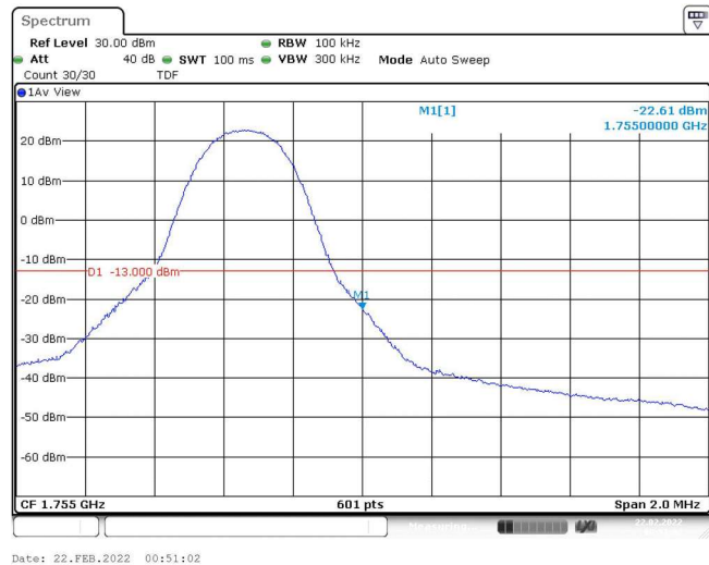
Band4-5MHz-16QAM-20375-1RB#24
