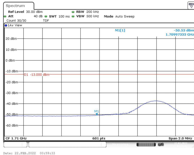
Band4-10MHz-16QAM-20000-1RB#49
