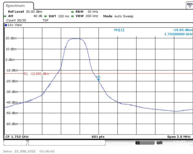
Band4-3MHz-16QAM-20385-1RB#14
