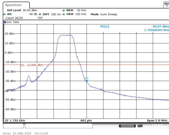
Band4-1.4MHz-QPSK-20393-1RB#5
