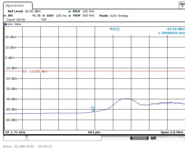
Band4-5MHz-QPSK-19975-1RB#24
