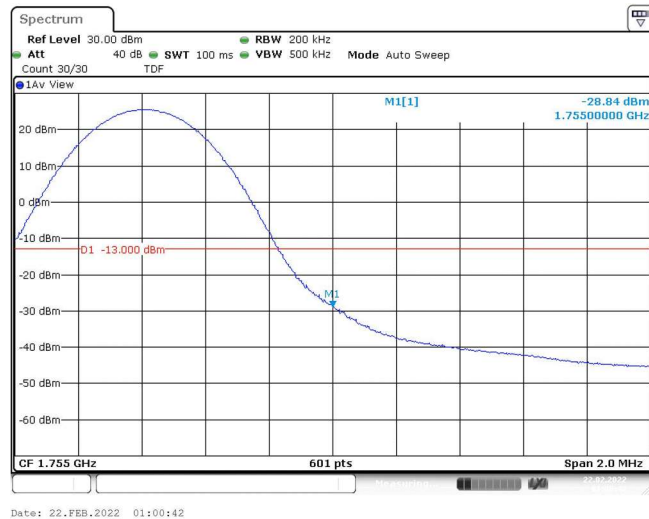
Band4-10MHz-QPSK-20350-1RB#49
