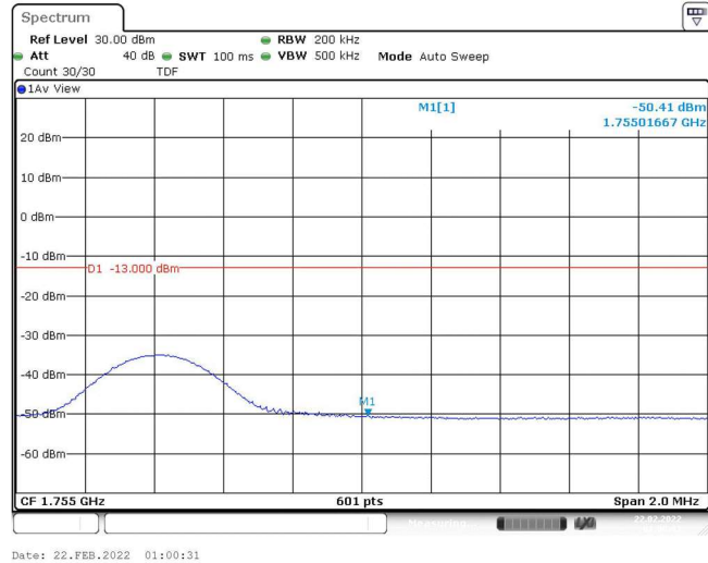
Band4-10MHz-16QAM-20350-1RB#0
