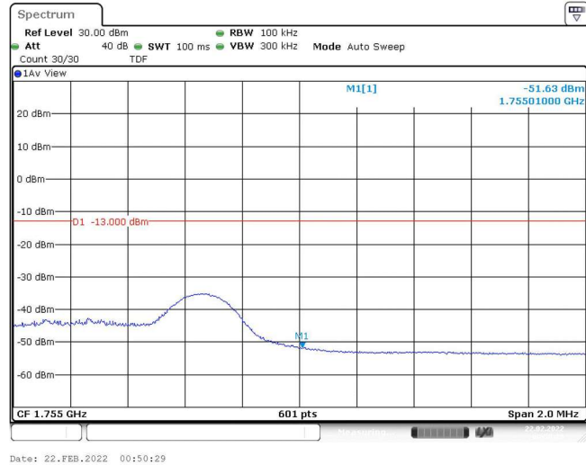
Band4-5MHz-QPSK-20375-1RB#0
