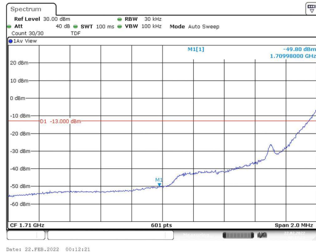
Band4-1.4MHz-QPSK-19957-1RB#5
