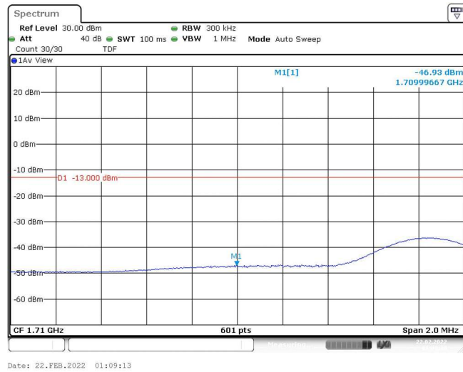
Band4-15MHz-QPSK-20025-1RB#74
