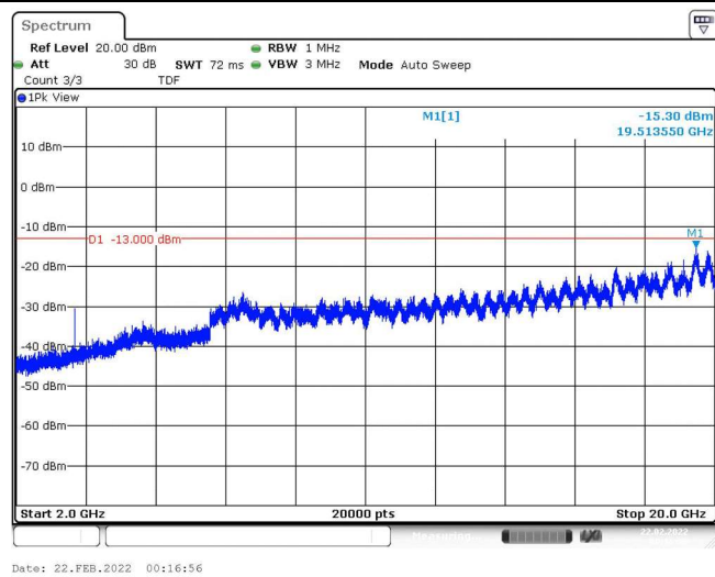
Band4-1.4MHz-QPSK-20393-1RB#0-Range3:2000~20000MHz
