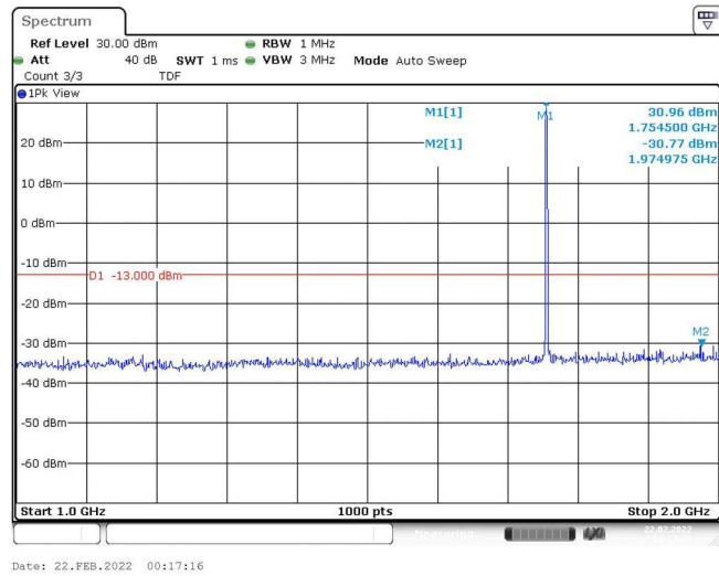
Band4-1.4MHz-16QAM-20393-1RB#0-Range2:1000~2000MHz
