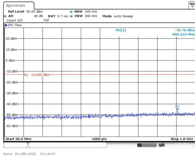
Band4-1.4MHz-16QAM-20175-1RB#0-Range1:30~1000MHz
