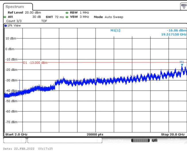
Band4-1.4MHz-16QAM-20393-1RB#0-Range3:2000~20000MHz
