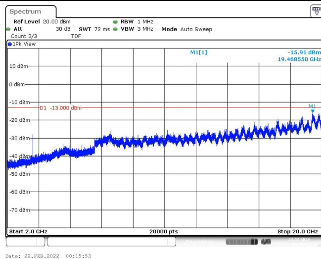
Band4-1.4MHz-QPSK-20175-1RB#0-Range3:2000~20000MHz
