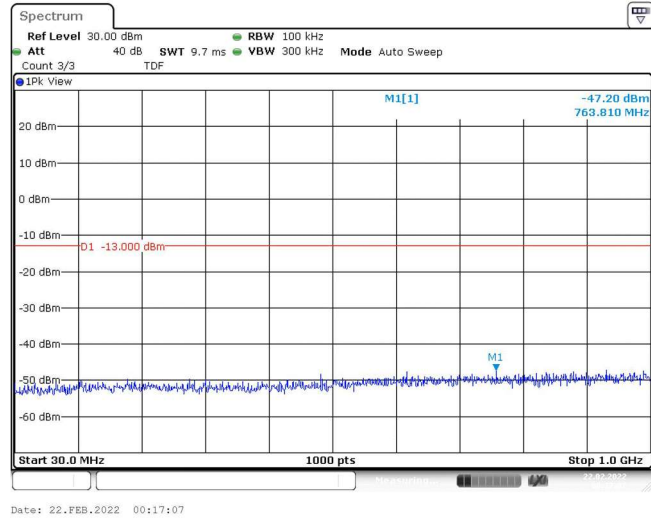
Band4-1.4MHz-16QAM-20393-1RB#0-Range1:30~1000MHz
