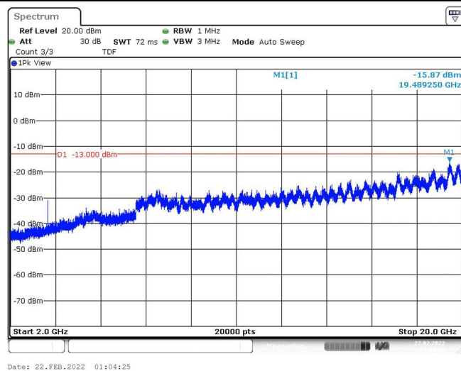
Band4-10MHz-16QAM-20350-1RB#0-Range3:2000~20000MHz
