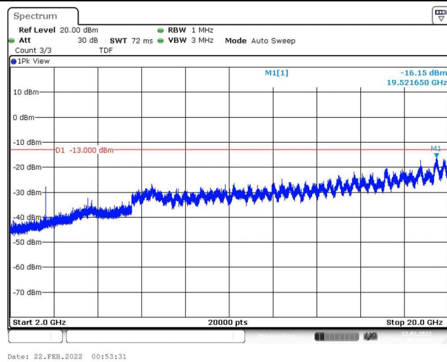
Band4-5MHz-16QAM-20175-1RB#0-Range3:2000~20000MHz
