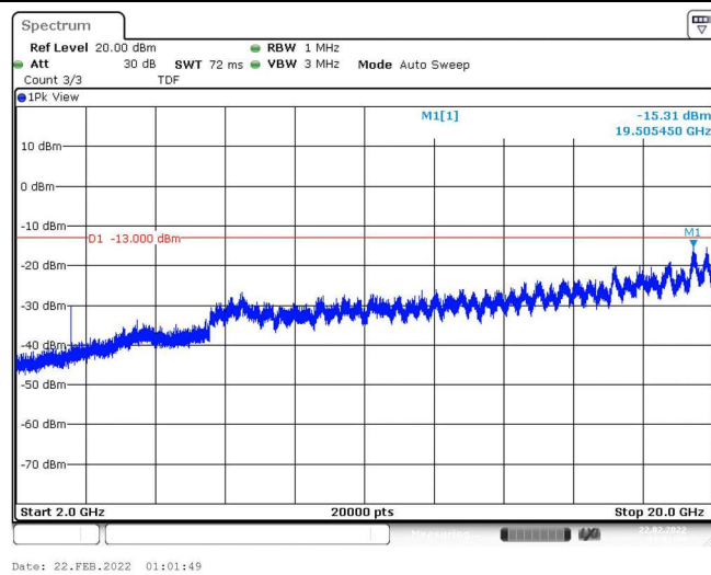
Band4-10MHz-QPSK-20000-1RB#0-Range3:2000~20000MHz
