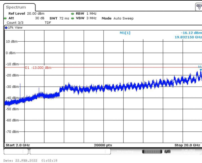
Band4-10MHz-16QAM-20000-1RB#0-Range3:2000~20000MHz
