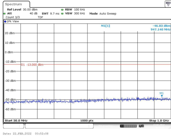
Band4-5MHz-16QAM-19975-1RB#0-Range1:30~1000MHz
