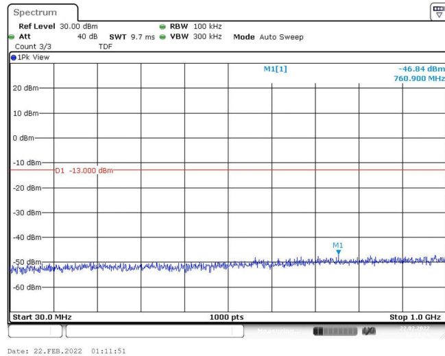
Band4-15MHz-16QAM-20025-1RB#0-Range1:30~1000MHz
