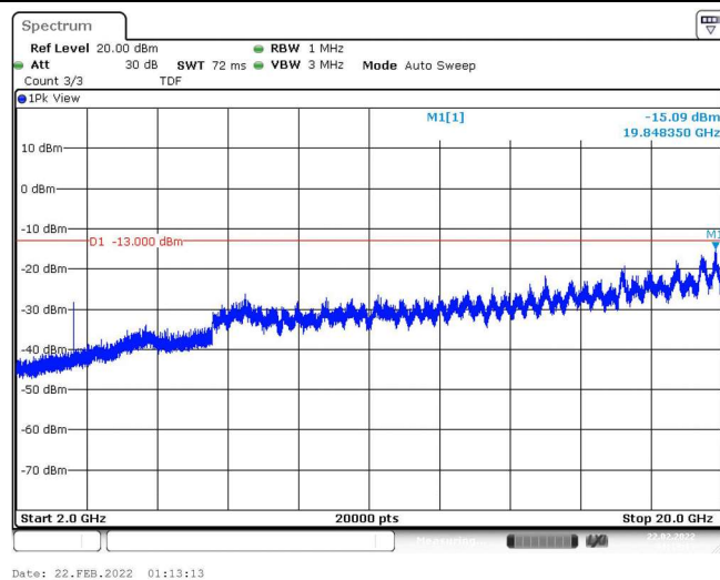
Band4-15MHz-16QAM-20175-1RB#0-Range3:2000~20000MHz
