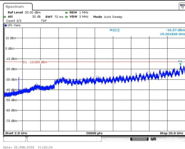
Band4-20MHz-QPSK-20175-1RB#0-Range3:2000~20000MHz
