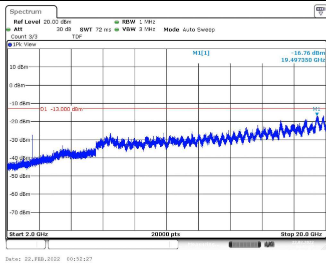
Band4-5MHz-16QAM-19975-1RB#0-Range3:2000~20000MHz
