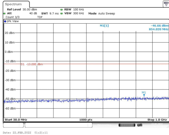
Band4-20MHz-QPSK-20050-1RB#0-Range1:30~1000MHz
