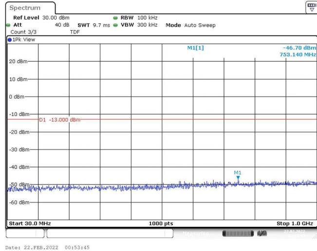
Band4-5MHz-QPSK-20375-1RB#0-Range1:30~1000MHz
