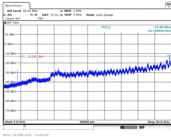
Band4-10MHz-16QAM-20175-1RB#0-Range3:2000~20000MHz
