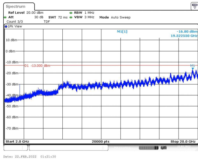
Band4-20MHz-QPSK-20050-1RB#0-Range3:2000~20000MHz
