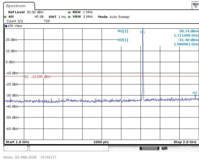
Band4-5MHz-16QAM-19975-1RB#0-Range2:1000~2000MHz
