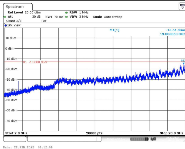
Band4-15MHz-16QAM-20025-1RB#0-Range3:2000~20000MHz
