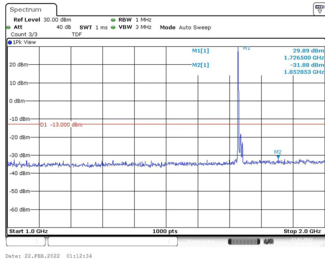
Band4-15MHz-QPSK-20175-1RB#0-Range2:1000~2000MHz
