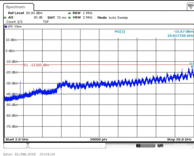
Band4-5MHz-QPSK-20375-1RB#0-Range3:2000~20000MHz
