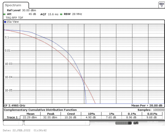
Band41-5MHz-QPSK-39675-25RB#0
