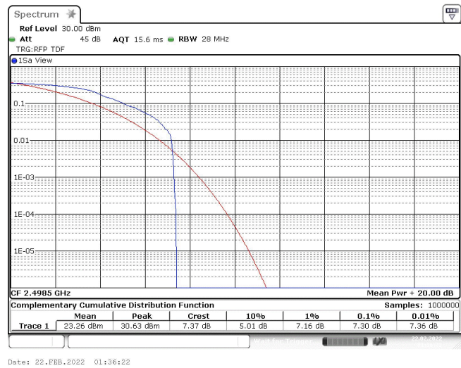
Band41-5MHz-QPSK-39675-1RB#0
