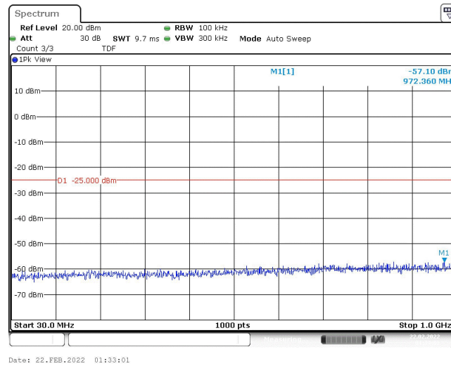
Band41-5MHz-QPSK-39675-1RB#0-Range1:30~1000MHz
