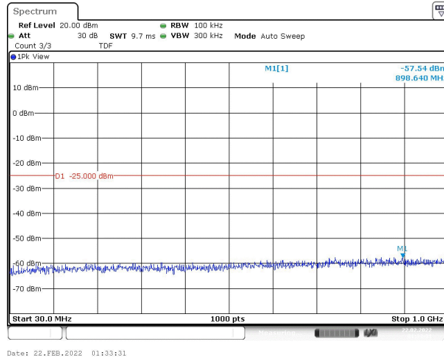
Band41-5MHz-16QAM-39675-1RB#0-Range1:30~1000MHz
