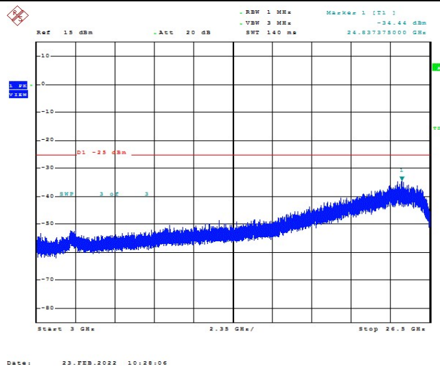
Band41-5MHz-16QAM-39675-1RB#0-Range1:3000~26500MHz
