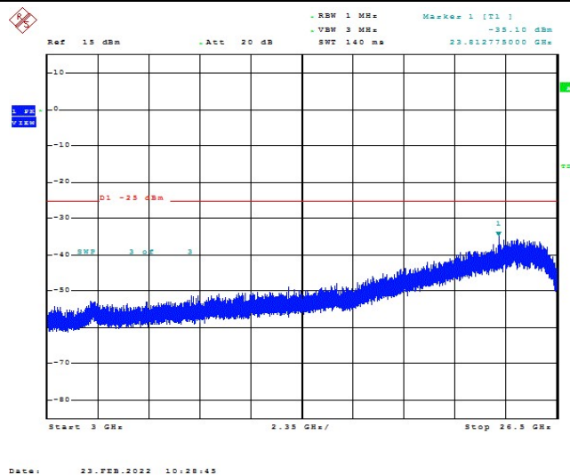
Band41-5MHz-16QAM-40620-1RB#0-Range1:3000~26500MHz
