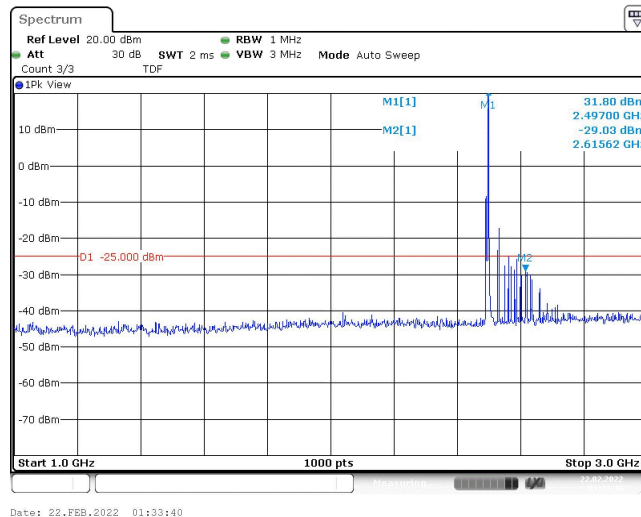
Band41-5MHz-16QAM-39675-1RB#0-Range2:1000~3000MHz
