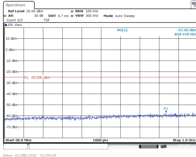
Band41-5MHz-16QAM-40620-1RB#0-Range1:30~1000MHz
