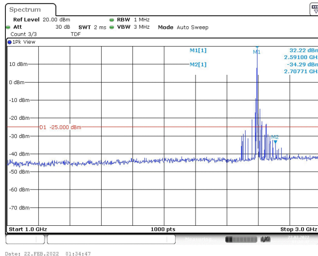
Band41-5MHz-16QAM-40620-1RB#0-Range2:1000~3000MHz
