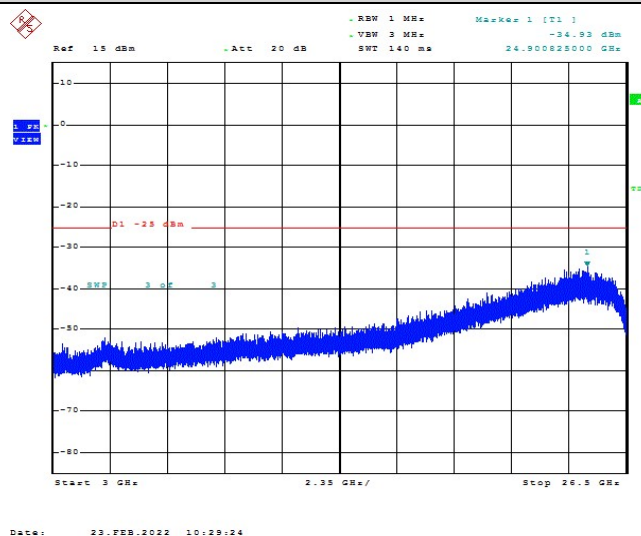
Band41-5MHz-16QAM-41565-1RB#0-Range1:3000~26500MHz
