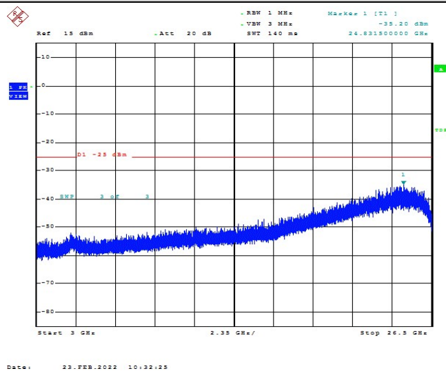
Band41-10MHz-16QAM-40620-1RB#0-Range1:3000~26500MHz
