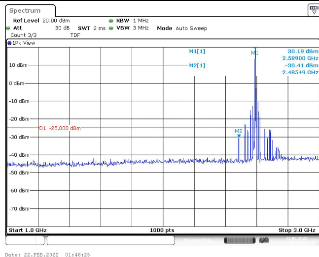
Band41-10MHz-16QAM-40620-1RB#0-Range2:1000~3000MHz
