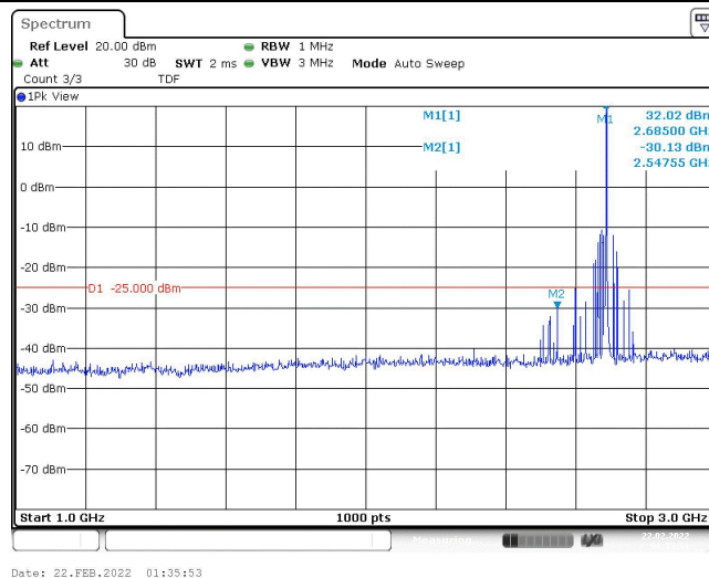
Band41-5MHz-16QAM-41565-1RB#0-Range2:1000~3000MHz
