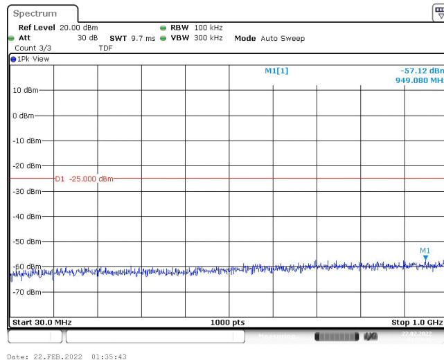
Band41-5MHz-16QAM-41565-1RB#0-Range1:30~1000MHz
