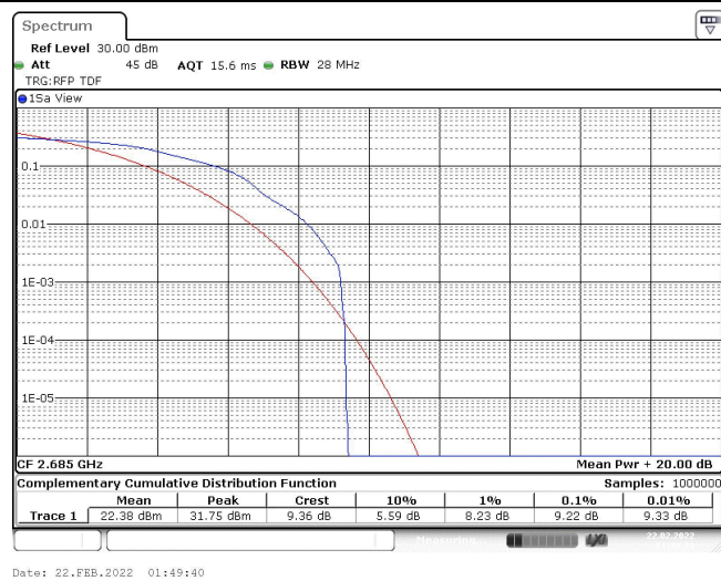
Band41-10MHz-16QAM-41540-1RB#0
