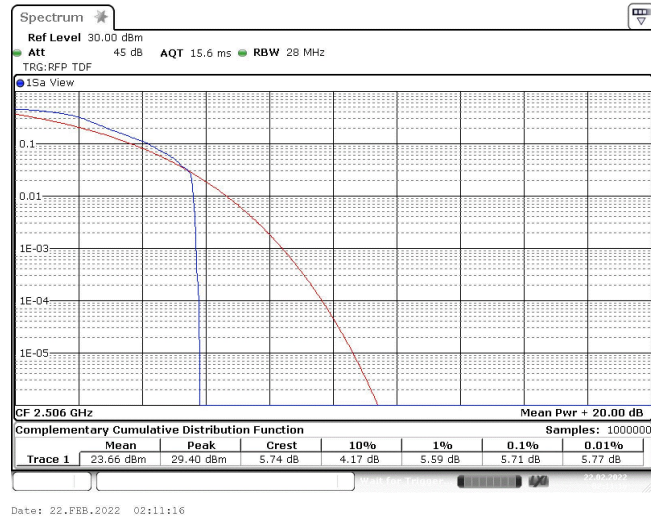
Band41-20MHz-QPSK-39750-1RB#0
