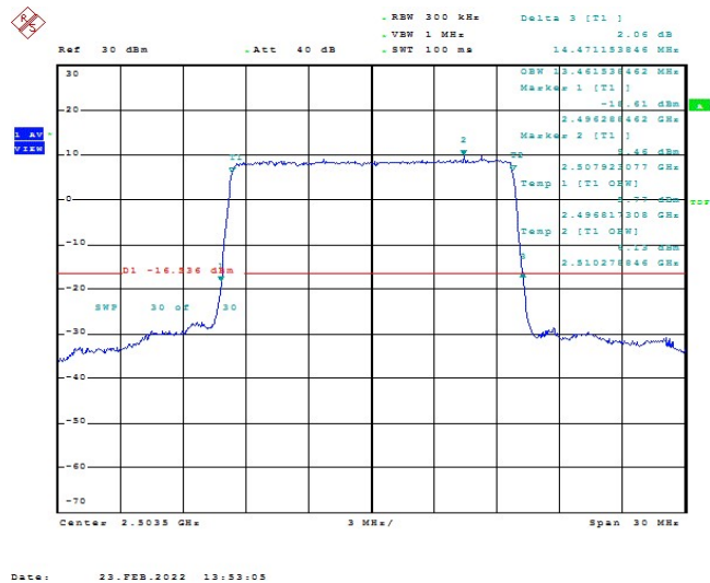
Band41-15MHz-16QAM-39725-75RB#0-13.462
