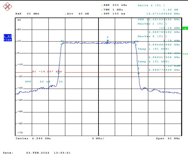
Band41-15MHz-16QAM-40620-75RB#0-13.462
