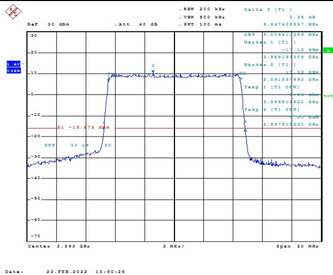
Band41-10MHz-16QAM-40620-50RB#0-9.006
