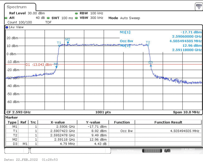
Band41-5MHz-QPSK-40620-25RB#0-4.505
