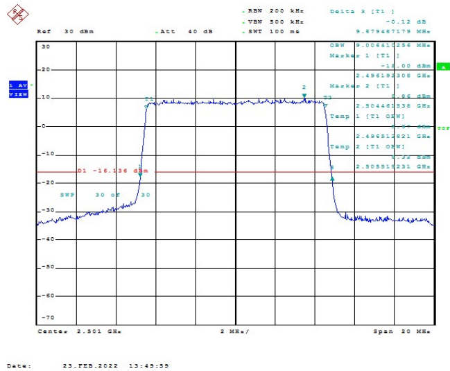
Band41-10MHz-16QAM-39700-50RB#0-9.006
