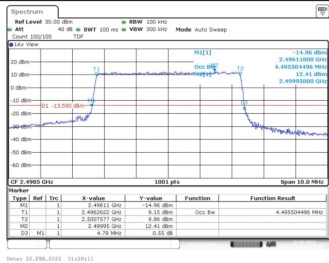
Band41-5MHz-QPSK-39675-25RB#0-4.496
