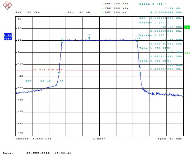
Band41-10MHz-QPSK-41540-50RB#0-9.006
