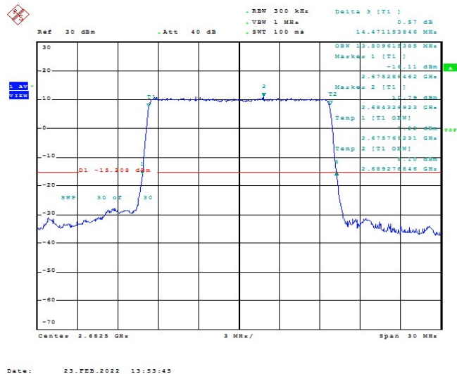
Band41-15MHz-QPSK-41515-75RB#0-13.51
