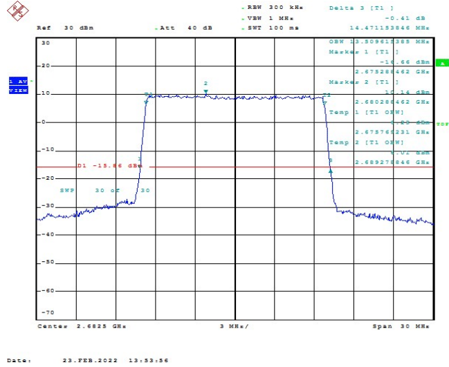
Band41-15MHz-16QAM-41515-75RB#0-13.51
