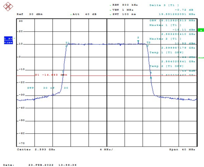
Band41-20MHz-QPSK-40620-100RB#0-18.013
