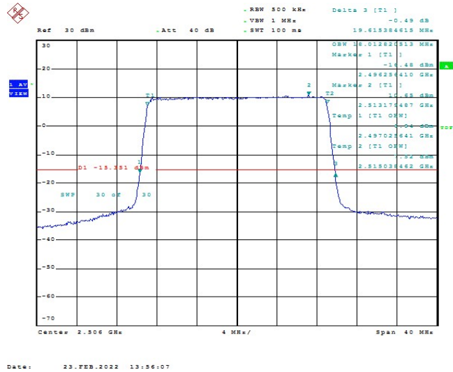
Band41-20MHz-QPSK-39750-100RB#0-18.013
