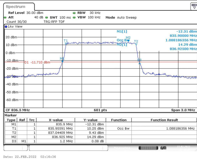
Band5-1.4MHz-QPSK-20525-6RB#0-1.088
