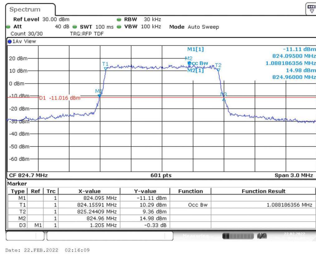
Band5-1.4MHz-QPSK-20407-6RB#0-1.088
