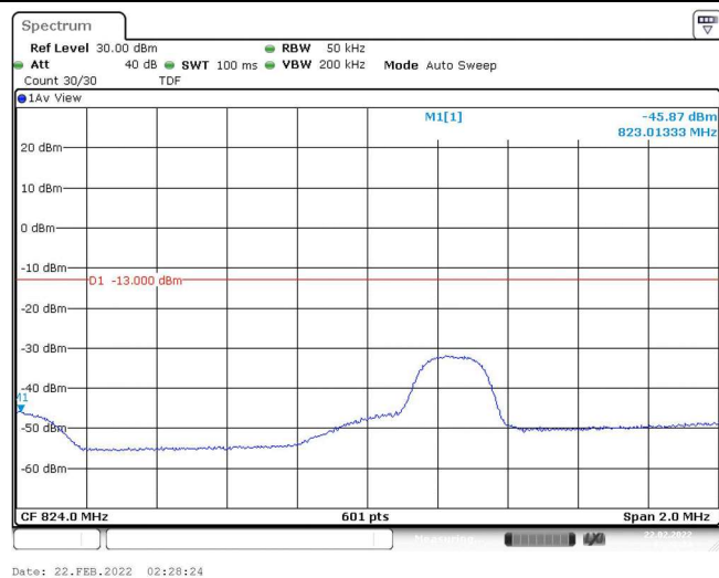
Band5-3MHz-QPSK-20415-1RB#14
