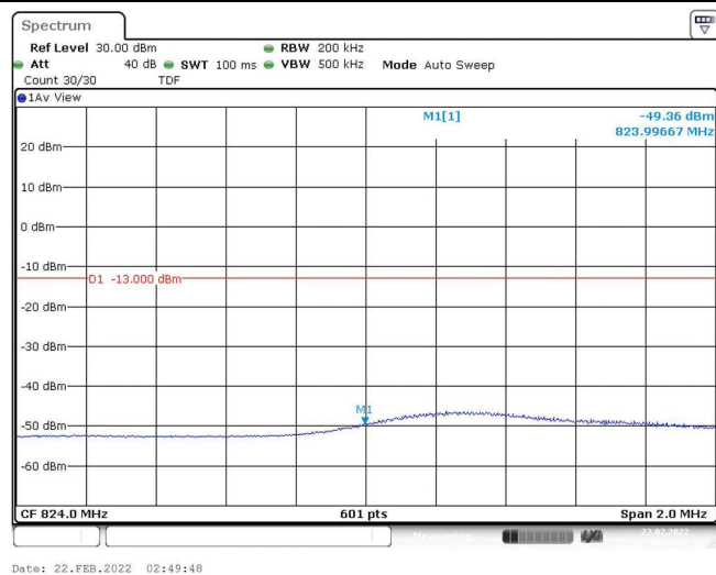
Band5-10MHz-QPSK-20450-1RB#49
