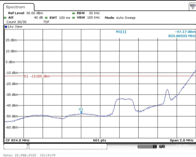
Band5-1.4MHz-16QAM-20407-1RB#5
