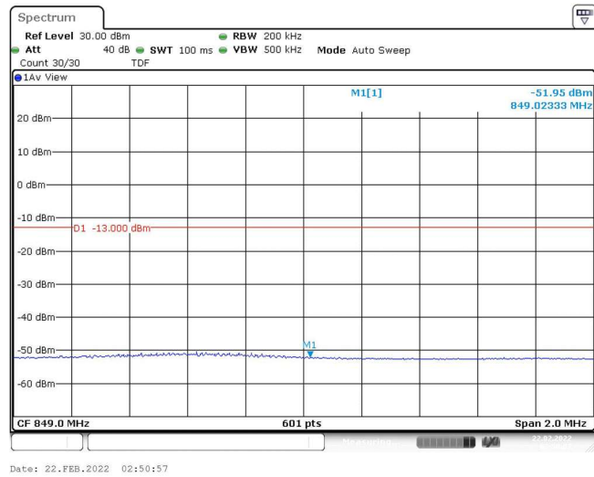
Band5-10MHz-16QAM-20600-1RB#0
