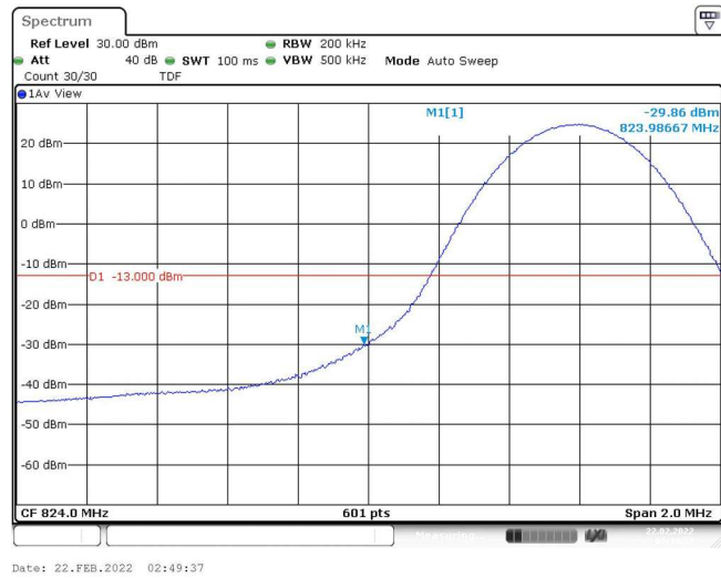
Band5-10MHz-16QAM-20450-1RB#0
