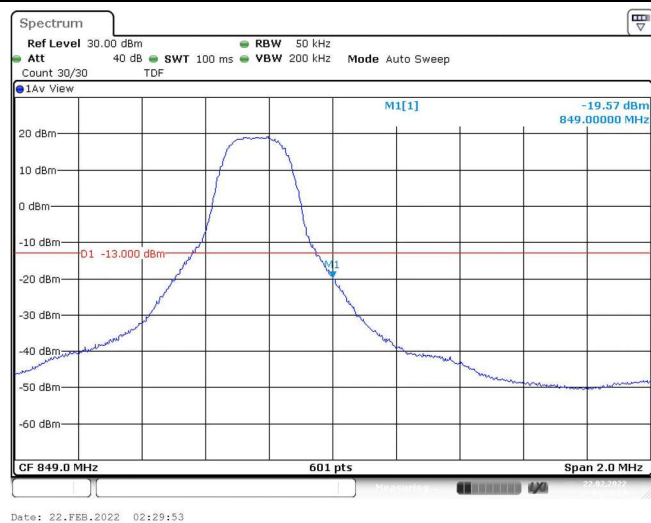
Band5-3MHz-16QAM-20635-1RB#14
