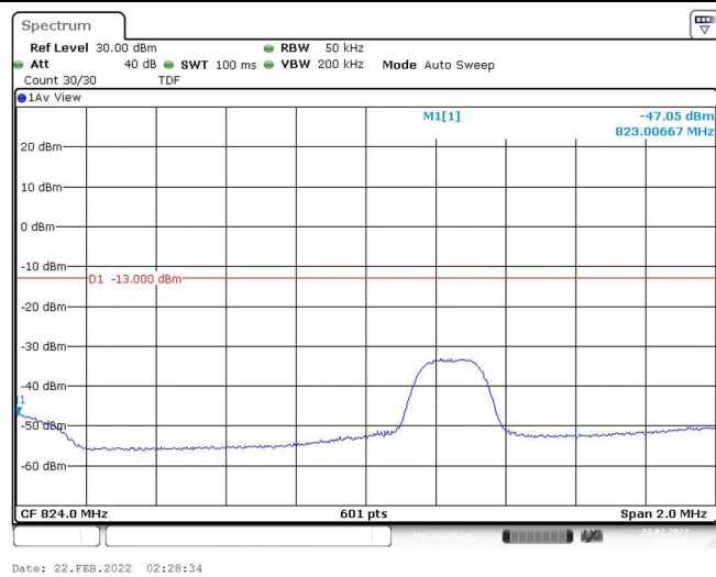
Band5-3MHz-16QAM-20415-1RB#14
