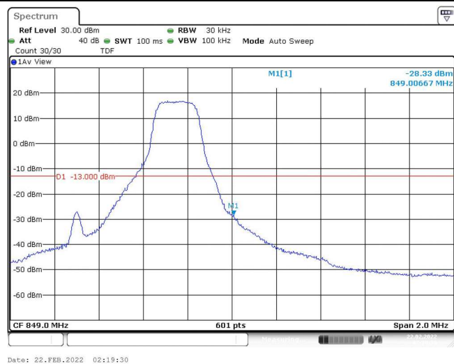
Band5-1.4MHz-16QAM-20643-1RB#5
