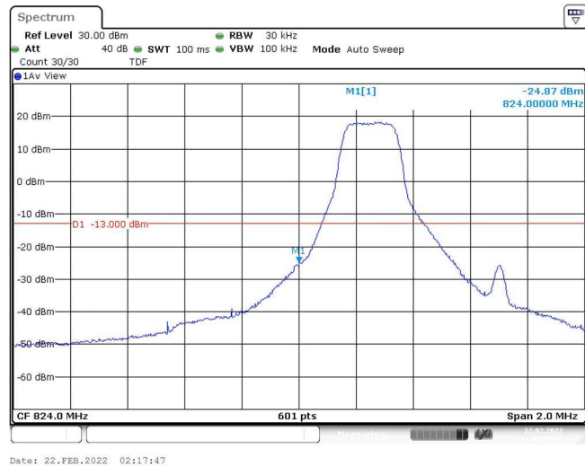
Band5-1.4MHz-16QAM-20407-1RB#0
