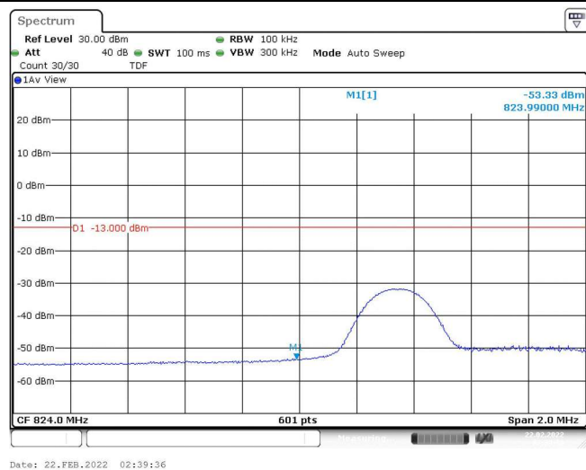
Band5-5MHz-16QAM-20425-1RB#24
