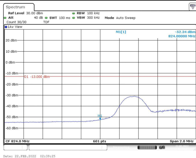
Band5-5MHz-QPSK-20425-1RB#24
