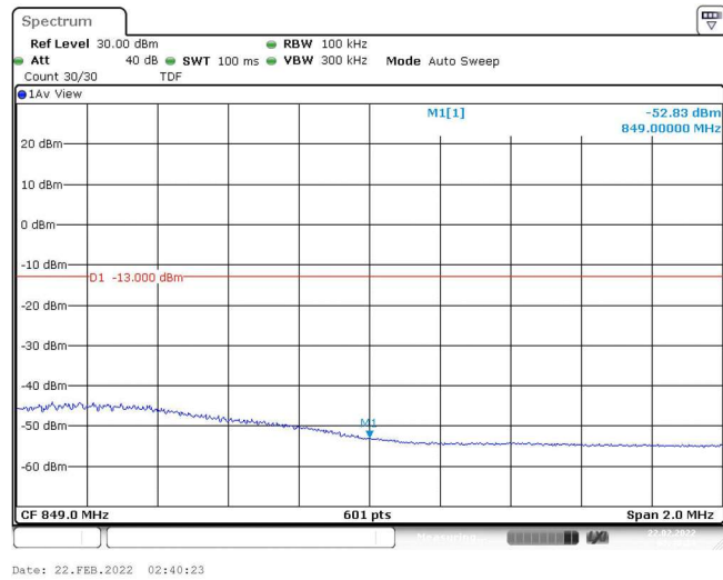
Band5-5MHz-QPSK-20625-1RB#0
