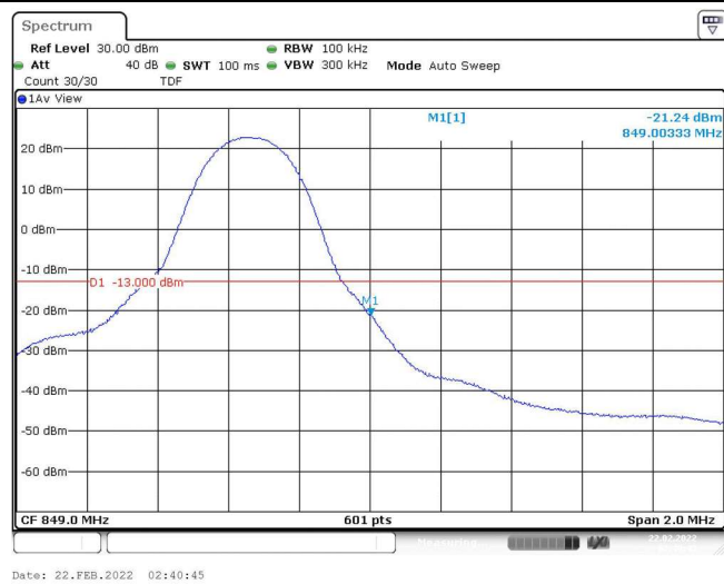
Band5-5MHz-QPSK-20625-1RB#24
