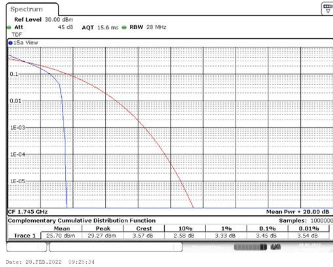
Band66-5MHz-QPSK-132322-1RB#0
