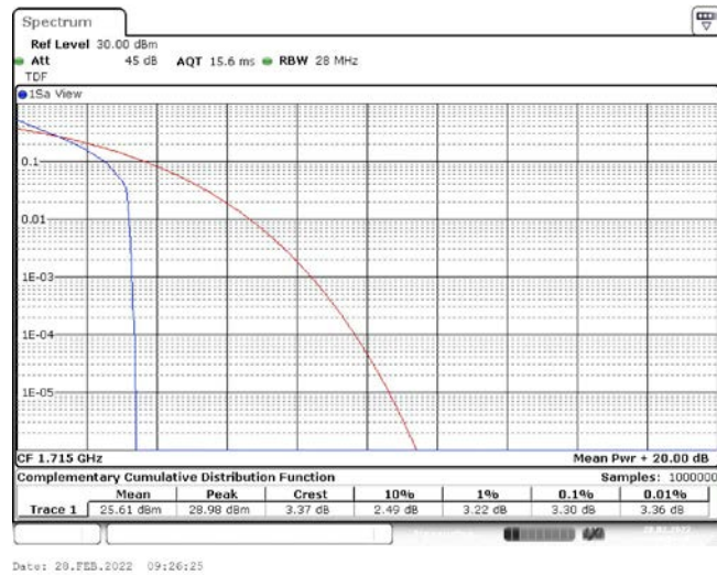
Band66-10MHz-QPSK-132022-1RB#0
