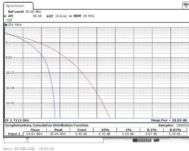
Band66-3MHz-QPSK-131987-15RB#0
