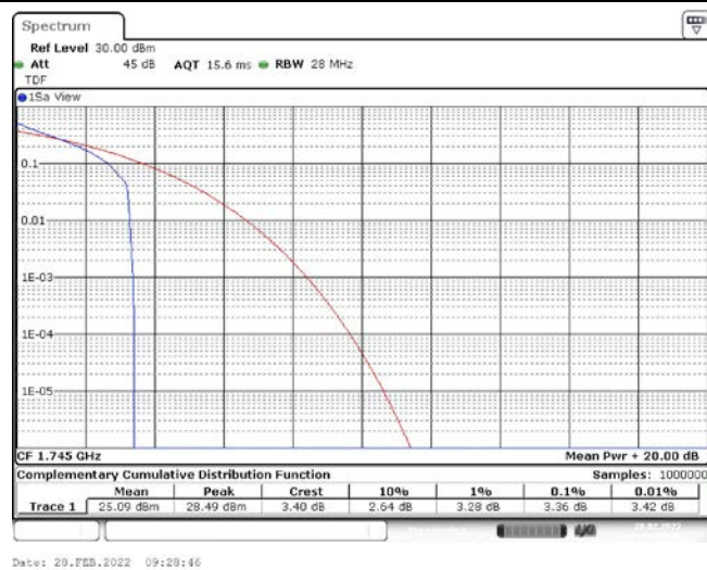
Band66-15MHz-QPSK-132322-1RB#0
