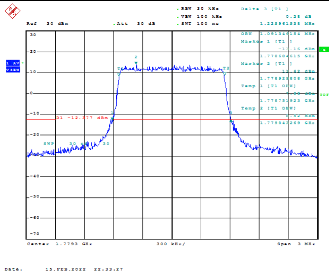
Band66-1.4MHz-16QAM-132665-6RB#0-1.091
