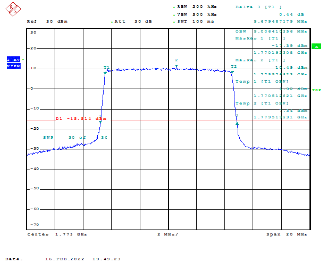
Band66-10MHz-QPSK-132622-50RB#0-9.006
