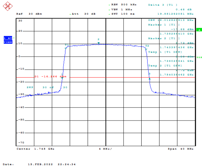
Band66-20MHz-16QAM-132322-100RB#0-18.013
