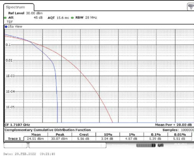
Band66-1.4MHz-16QAM-131979-1RB#0
