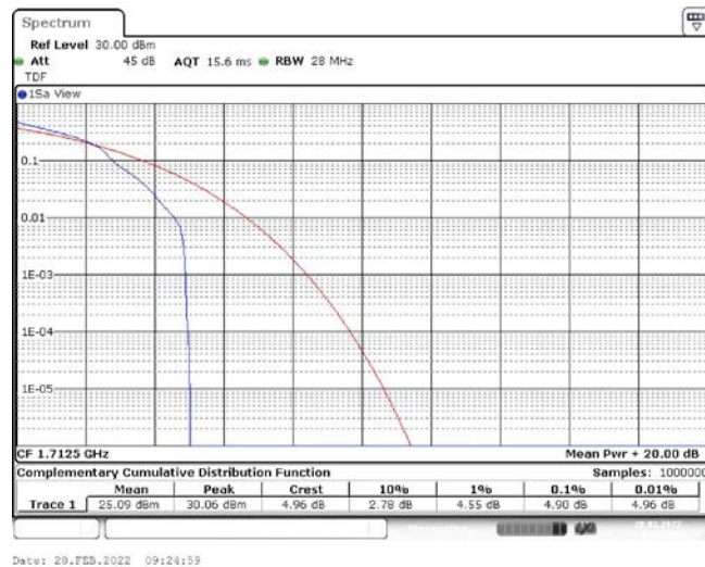
Band66-5MHz-16QAM-131997-1RB#0
