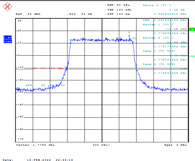
Band66-1.4MHz-QPSK-132665-6RB#0-1.091
