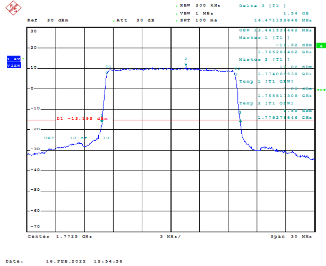
Band66-15MHz-QPSK-132597-75RB#0-13.462
