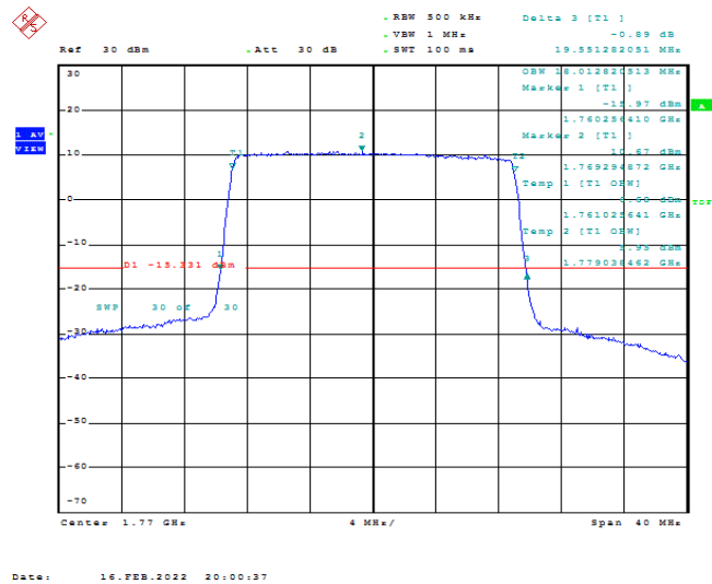
Band66-20MHz-QPSK-132572-100RB#0-18.013
