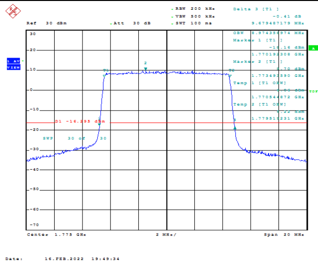
Band66-10MHz-16QAM-132622-50RB#0-8.974
