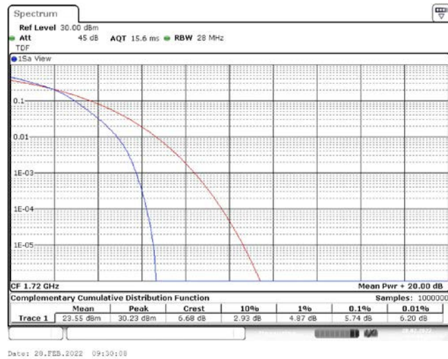
Band66-20MHz-16QAM-132047-100RB#0
