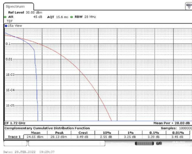
Band66-20MHz-QPSK-132047-1RB#0
