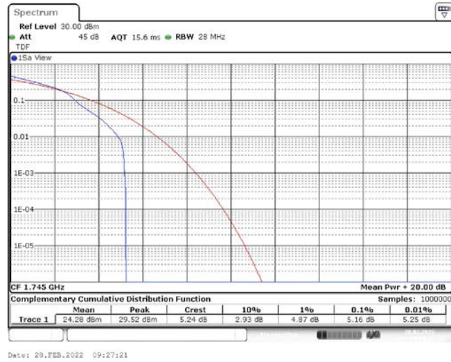
Band66-10MHz-16QAM-132322-1RB#0
