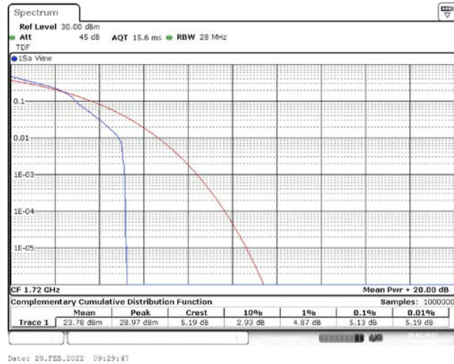
Band66-20MHz-16QAM-132047-1RB#0
