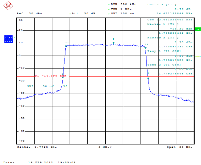
Band66-15MHz-16QAM-132597-75RB#0-13.462
