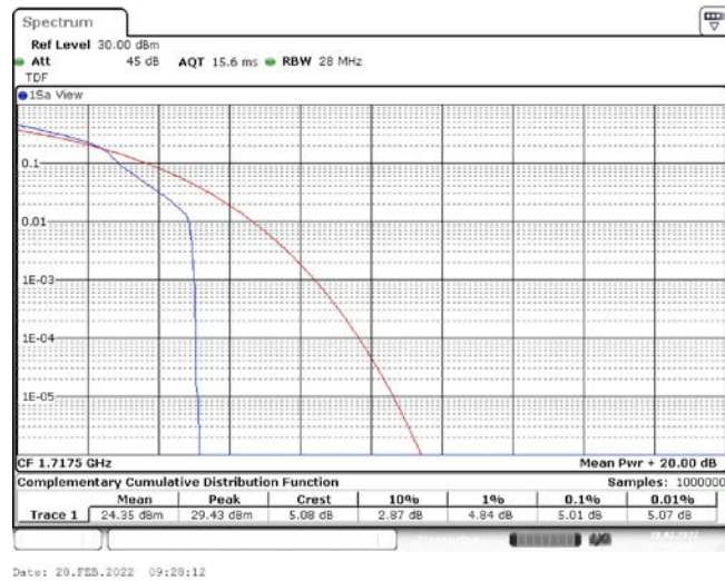
Band66-15MHz-16QAM-132047-1RB#0
