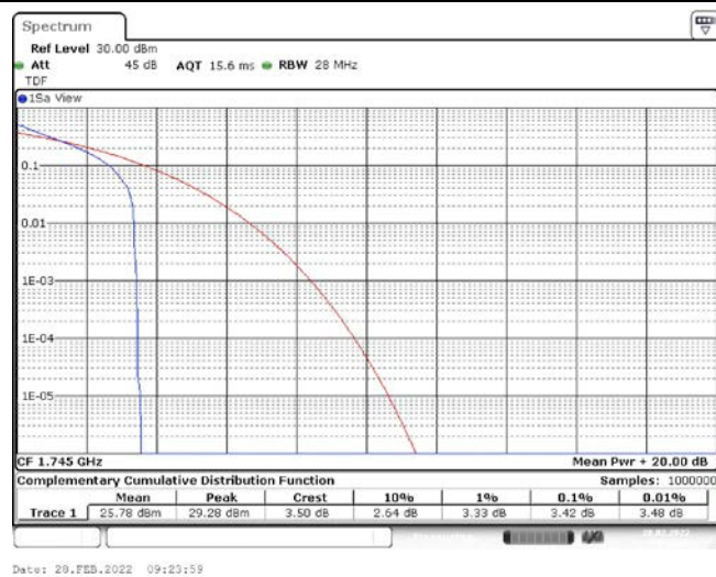
Band66-3MHz-QPSK-132322-1RB#0
