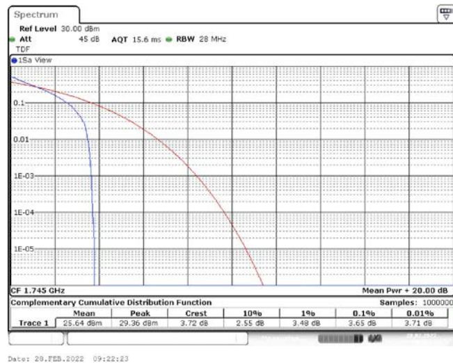
Band66-1.4MHz-QPSK-132322-1RB#0
