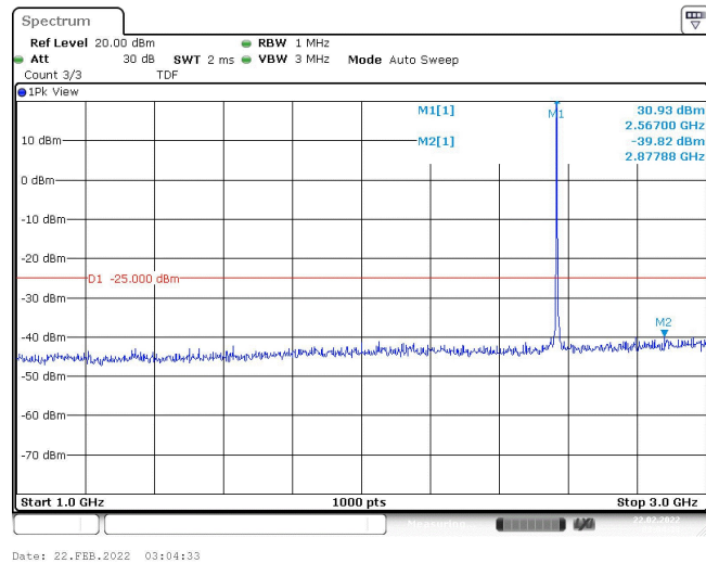
Band7-5MHz-16QAM-21425-1RB#0-Range2:1000~3000MHz
