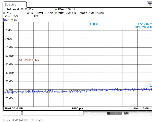
Band7-5MHz-QPSK-20775-1RB#0-Range1:30~1000MHz
