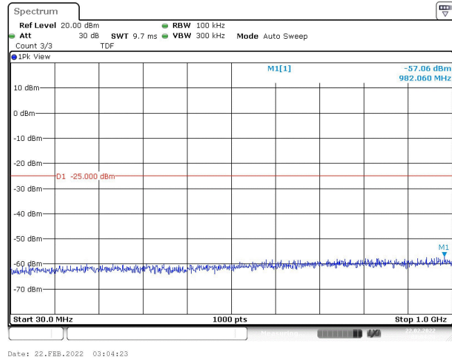
Band7-5MHz-16QAM-21425-1RB#0-Range1:30~1000MHz
