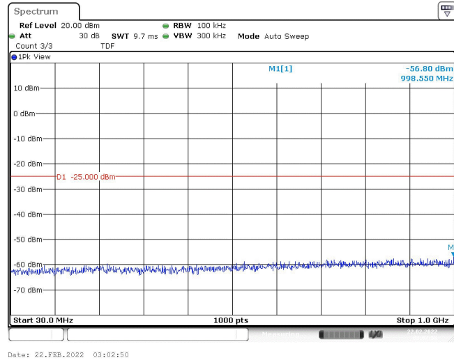
Band7-5MHz-QPSK-21100-1RB#0-Range1:30~1000MHz
