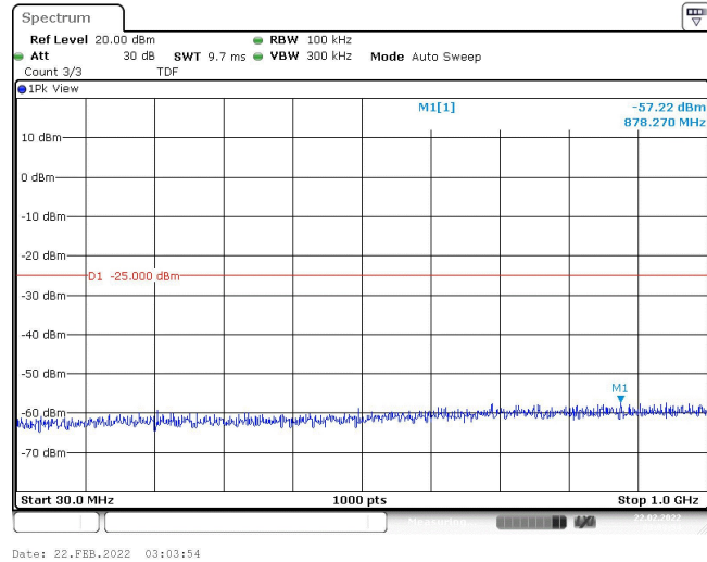
Band7-5MHz-QPSK-21425-1RB#0-Range1:30~1000MHz
