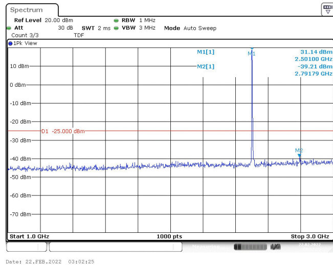
Band7-5MHz-16QAM-20775-1RB#0-Range2:1000~3000MHz
