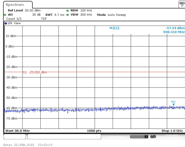
Band7-5MHz-16QAM-20775-1RB#0-Range1:30~1000MHz
