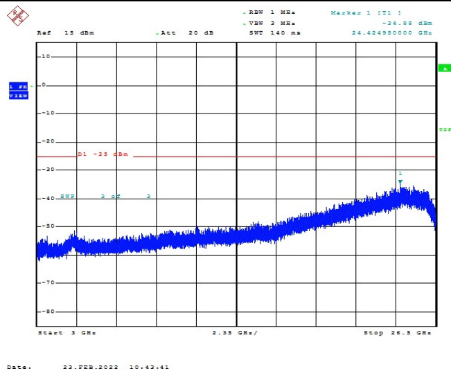
Band7-5MHz-16QAM-21425-1RB#0-Range1:3000~26500MHz
