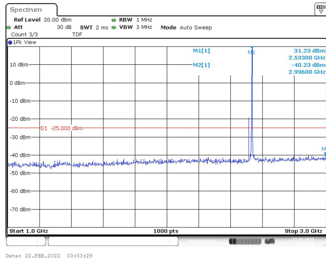
Band7-5MHz-16QAM-21100-1RB#0-Range2:1000~3000MHz
