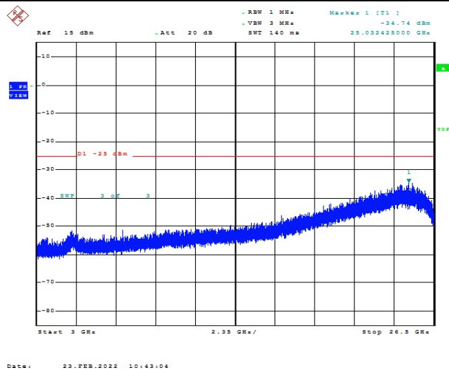
Band7-5MHz-16QAM-21100-1RB#0-Range1:3000~26500MHz
