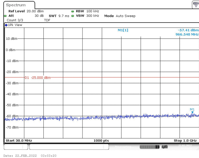
Band7-5MHz-16QAM-21100-1RB#0-Range1:30~1000MHz
