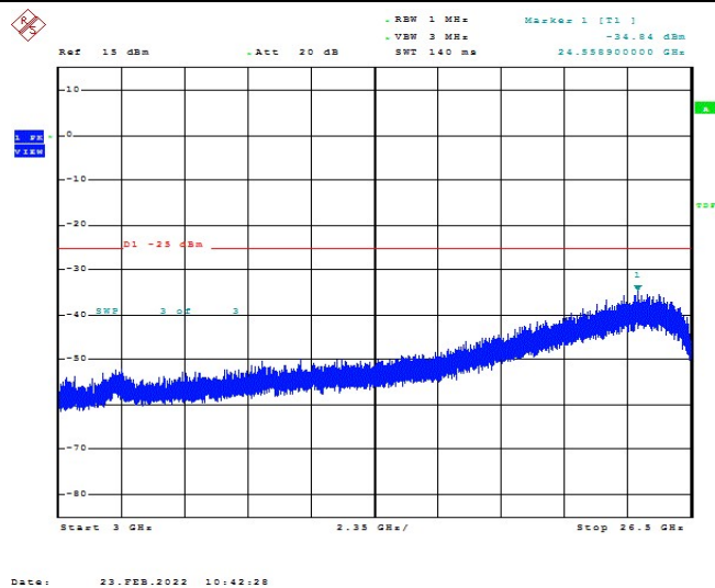
Band7-5MHz-16QAM-20775-1RB#0-Range1:3000~26500MHz
